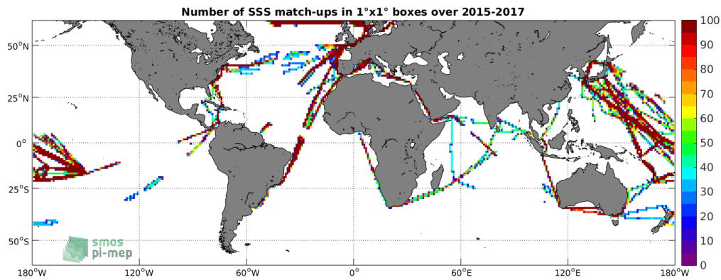
Figure 4: Number of SSS match-ups between TSG-LEGOS-DM SSS and the SMAP-L3-JPL-V4-MONTHLY-60KM SSS product for the SMOS coastal zone ( \pm 800\text{km} ) 60N-60S Pi-MEP region over 1^\circ \times 1^\circ boxes and for the full satellite product period.
