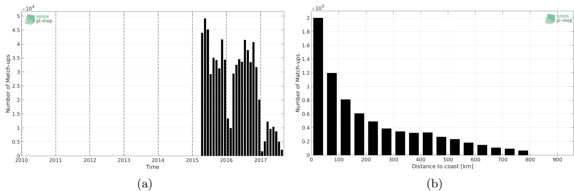
Figure 1: Number of match-ups between TSG-LEGOS-DM and SMAP-L3-JPL-V4-MONTHLY-60KM SSS as a function of time (a) and as function of the distance to coast (b) over the SMOS coastal zone ( \leq 800 km) 60N-60S Pi-MEP region and for the full satellite product period.
