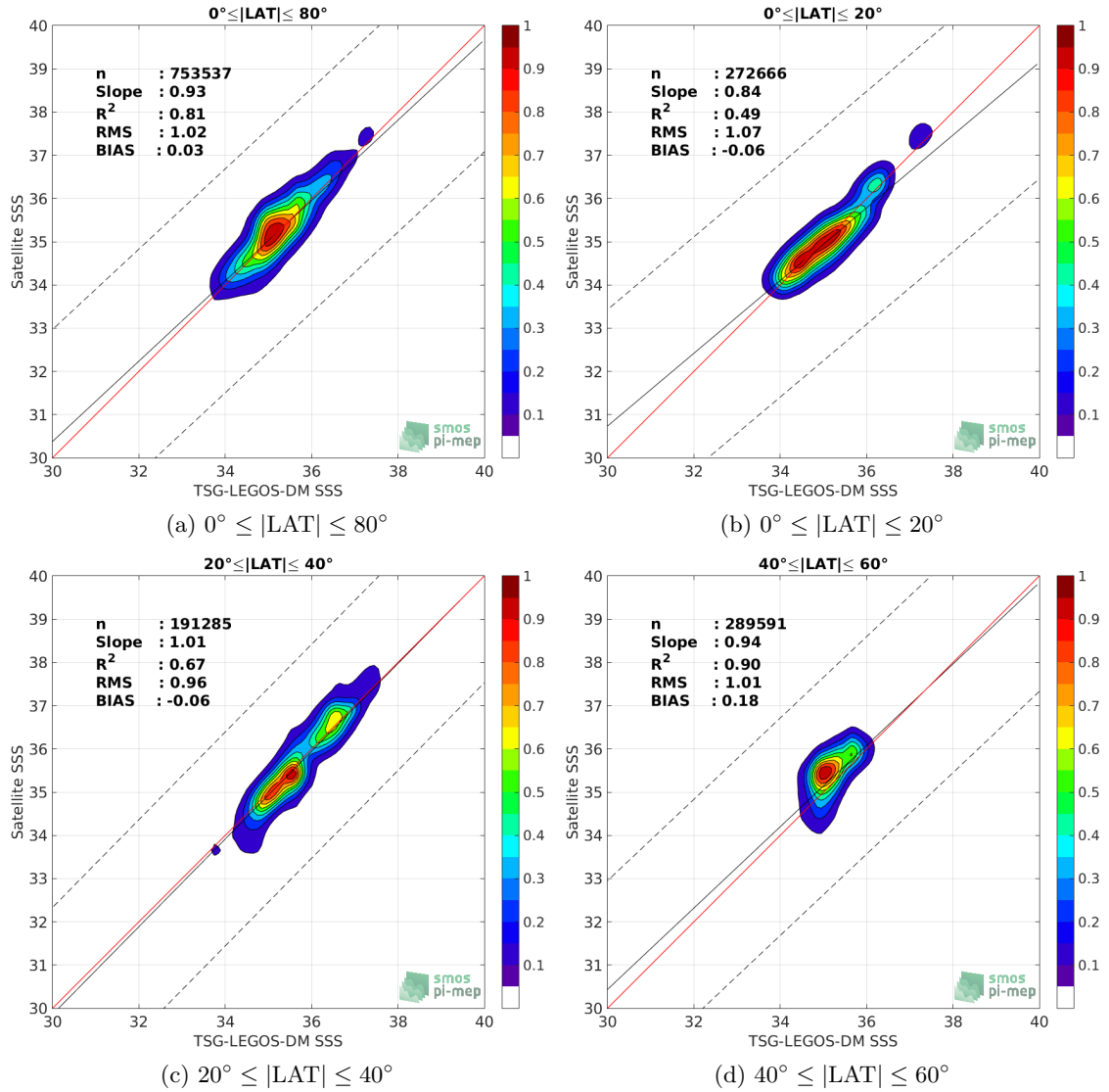
Figure 9: Contour maps of the concentration of SMAP-L3-JPL-V4-MONTHLY-60KM SSS (y-axis) versus TSG-LEGOS-DM SSS (x-axis) at match-up pairs for different latitude bands. For each plot, the red line shows x=y . The black thin and dashed lines indicate a linear fit through the data cloud and the \pm 95\% confidence levels, respectively. The number match-up pairs n , the slope and R^2 coefficient of the linear fit, the root mean square (RMS) and the mean bias between satellite and in situ data are indicated for each latitude band in each plots.
