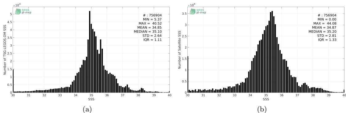
Figure 2: Histograms of SSS from TSG-LEGOS-DM (a) and SMAP-L3-JPL-V4-MONTHLY-60KM (b) considering all match-up pairs per bins of 0.1 over the SMOS coastal zone ( \leq 800 km) 60N-60S Pi-MEP region and for the full satellite product period.
