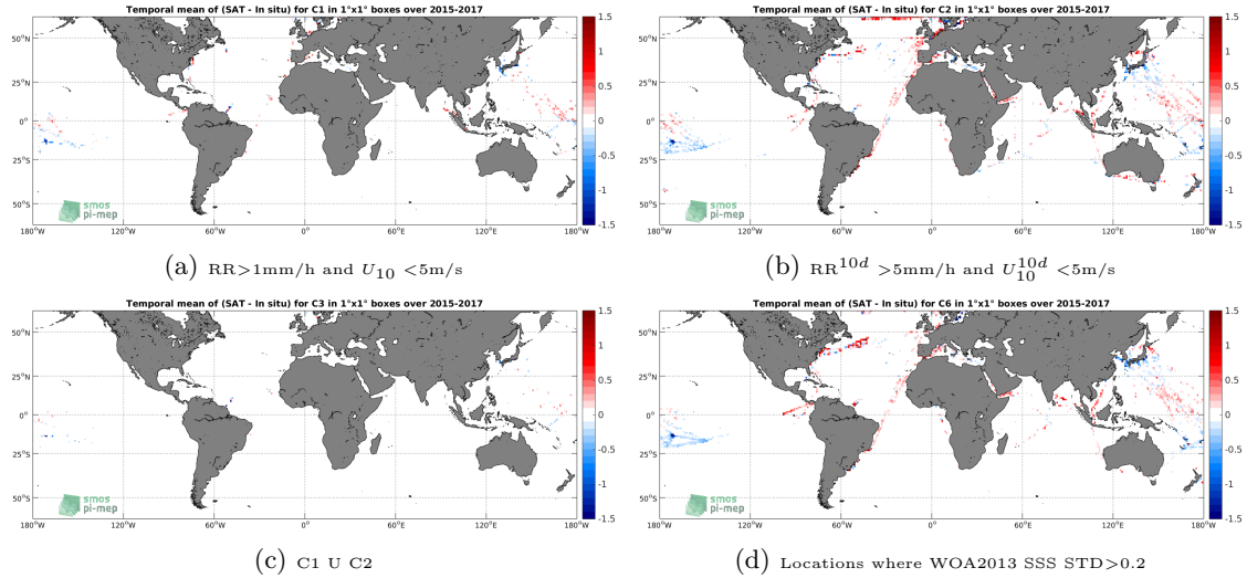
Figure 12: Temporal mean gridded over spatial boxes of size 1^\circ \times 1^\circ of \Delta SSS (SMAP-L3-JPL-V4-MONTHLY-60KM - TSG-LEGOS-DM) for 4 different subdatasets corresponding to: RR > 1\text{mm/h} and U_{10} < 5\text{m/s} (a), RR^{10d} > 5\text{mm/h} and U_{10}^{10d} < 5\text{m/s} (b), C1 U C2 (c), Locations where WOA2013 SSS STD > 0.2 (d).
