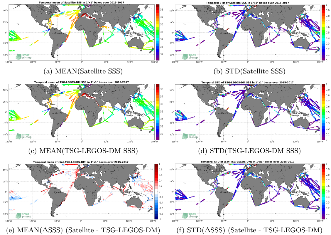
Figure 6: Temporal mean (left) and STD (right) of SSS from SMAP-L3-JPL-V4-MONTHLY-60KM (top), TSG-LEGOS-DM (middle), and of \Delta SSS (Satellite - TSG-LEGOS-DM). Only match-up pairs are used to generate these maps.
