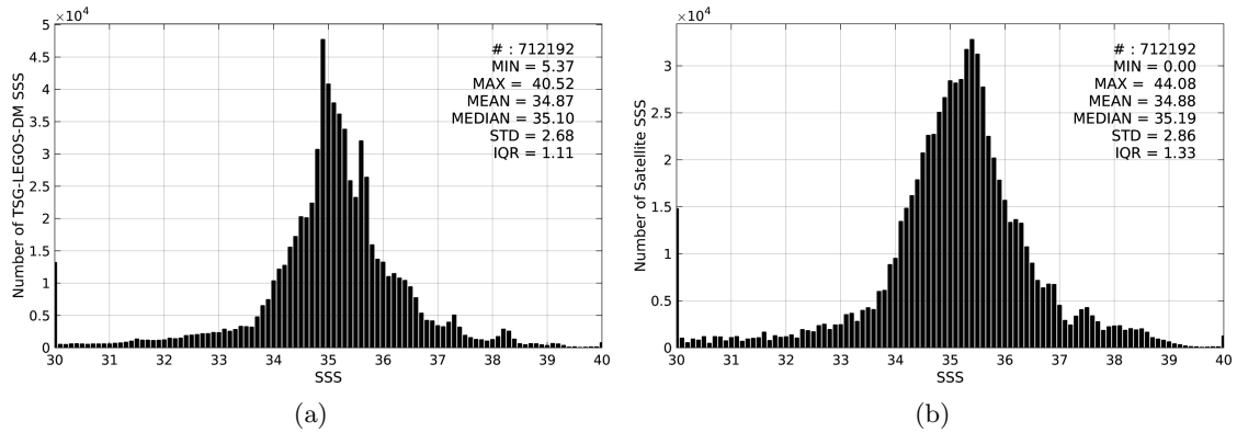
Figure 2: Histograms of SSS from TSG-LEGOS-DM (a) and SMAP-L3-JPL-V4-MONTHLY-60KM (b) considering all match-up pairs per bins of 0.1 over the SMOS coastal zone ( \pm 800 km) 60N-60S Pi-MEP region and for the full satellite product period.
