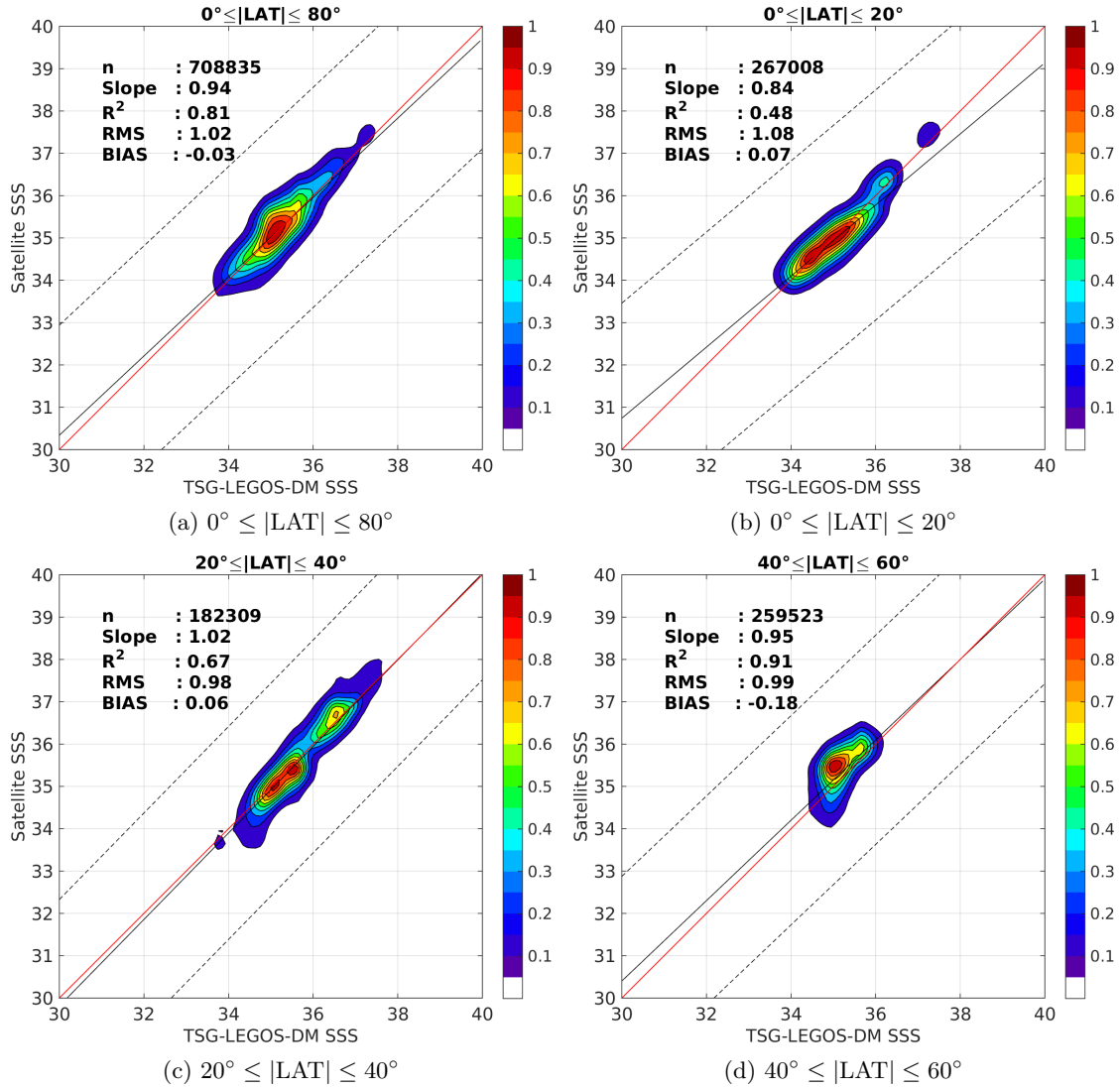
Figure 9: Contour maps of the concentration of SMAP-L3-JPL-V4-MONTHLY-60KM SSS (y-axis) versus TSG-LEGOS-DM SSS (x-axis) at match-up pairs for different latitude bands. For each plot, the red line shows x=y . The black thin and dashed lines indicate a linear fit through the data cloud and the \pm 95\% confidence levels, respectively. The number match-up pairs n , the slope and R^2 coefficient of the linear fit, the root mean square (RMS) and the mean bias between satellite and in situ data are indicated for each latitude band in each plots.
