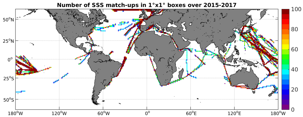
Figure 4: Number of SSS match-ups between TSG-LEGOS-DM SSS and the SMAP-L3-JPL-V4-MONTHLY-60KM SSS product for the SMOS coastal zone ( \approx 800\text{km} ) 60N-60S Pi-MEP region over 1^\circ \times 1^\circ boxes and for the full satellite product period.
