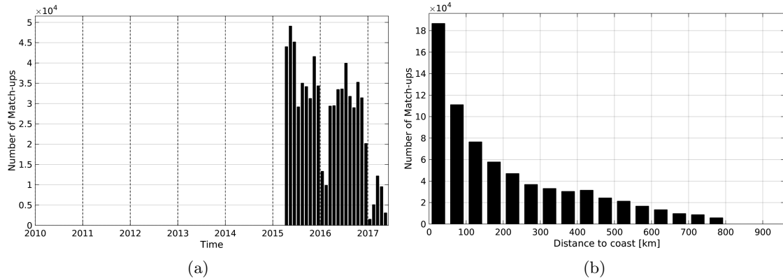
Figure 1: Number of match-ups between TSG-LEGOS-DM and SMAP-L3-JPL-V4-MONTHLY-60KM SSS as a function of time (a) and as function of the distance to coast (b) over the SMOS coastal zone ( \pm 800 km) 60N-60S Pi-MEP region and for the full satellite product period.
