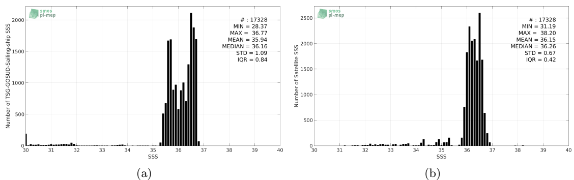
Figure 2: Histograms of SSS from TSG-GOSUD-Sailing-ship (a) and SMAP-L3-JPL-V4-MONTHLY-60KM (b) considering all match-up pairs per bins of 0.1 over the SMOS coastal zone ( \leq 800 km) 60N-60S Pi-MEP region and for the full satellite product period.
