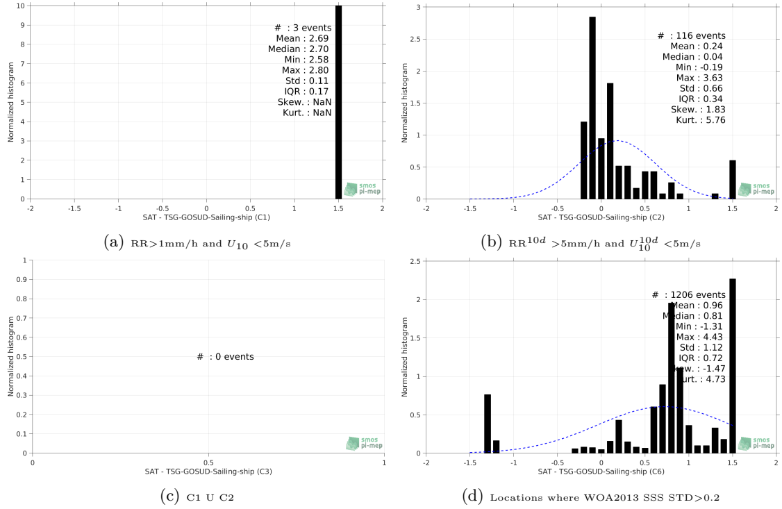
Figure 13: Normalized histogram of \Delta\text{SSS} (SMAP-L3-JPL-V4-MONTHLY-60KM - TSG-GOSUD-Sailing-ship) for 6 different subdatasets corresponding to: RR > 1mm/h and U_{10} < 5\text{m/s} (a), RR^{10d} > 5\text{mm/h} and U_{10}^{10d} < 5\text{m/s} (b), C1 U C2 (c), Locations where WOA2013 SSS STD > 0.2 (d).
