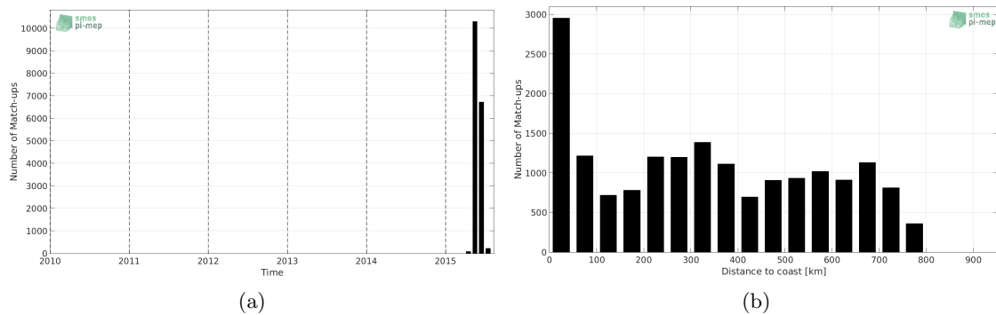
Figure 1: Number of match-ups between TSG-GOSUD-Sailing-ship and SMAP-L3-JPL-V4-MONTHLY-60KM SSS as a function of time (a) and as function of the distance to coast (b) over the SMOS coastal zone ( \leq 800 km) 60N-60S Pi-MEP region and for the full satellite product period.
