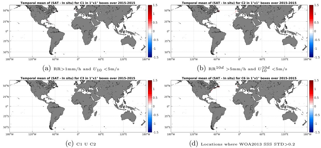
Figure 12: Temporal mean gridded over spatial boxes of size 1^\circ \times 1^\circ of \Delta SSS (SMAP-L3-JPL-V4-MONTHLY-60KM - TSG-GOSUD-Sailing-ship) for 4 different subdatasets corresponding to: RR > 1mm/h and U_{10} < 5\text{m/s} (a), RR 10d > 5mm/h and U_{10}^{10d} < 5\text{m/s} (b), C1 U C2 (c), Locations where WOA2013 SSS STD > 0.2 (d).
