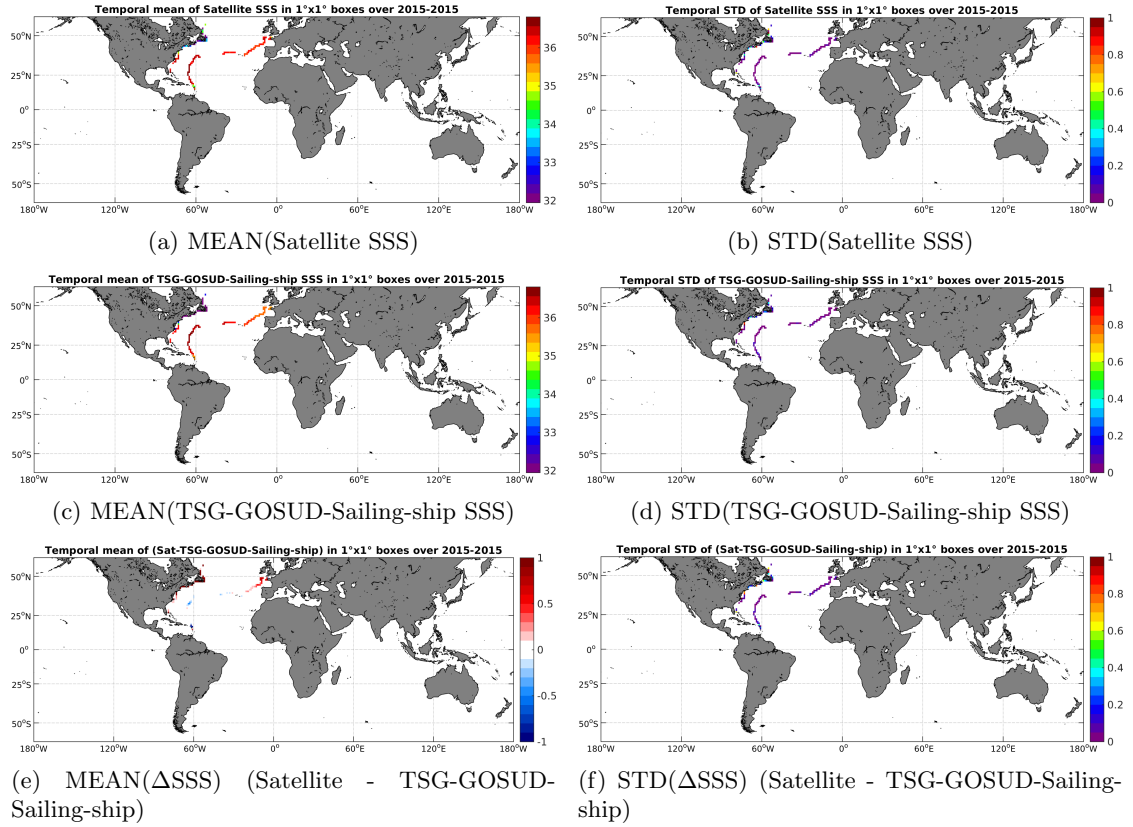
Figure 6: Temporal mean (left) and STD (right) of SSS from SMAP-L3-JPL-V4-MONTHLY-60KM (top), TSG-GOSUD-Sailing-ship (middle), and of \Delta SSS (Satellite - TSG-GOSUD-Sailing-ship). Only match-up pairs are used to generate these maps.
