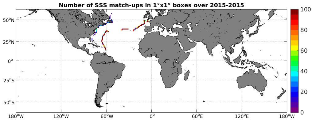
Figure 4: Number of SSS match-ups between TSG-GOSUD-Sailing-ship SSS and the SMAP-L3-JPL-V4-MONTHLY-60KM SSS product for the SMOS coastal zone ( \pm 800\text{km} ) 60N-60S Pi-MEP region over 1^\circ \times 1^\circ boxes and for the full satellite product period.
