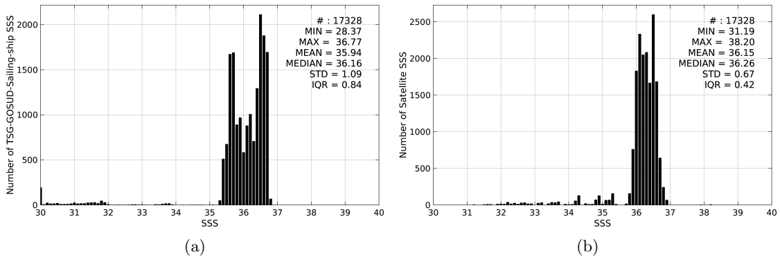
Figure 2: Histograms of SSS from TSG-GOSUD-Sailing-ship (a) and SMAP-L3-JPL-V4-MONTHLY-60KM (b) considering all match-up pairs per bins of 0.1 over the SMOS coastal zone ( \approx 800\text{km} ) 60N-60S Pi-MEP region and for the full satellite product period.
