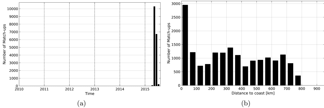
Figure 1: Number of match-ups between TSG-GOSUD-Sailing-ship and SMAP-L3-JPL-V4-MONTHLY-60KM SSS as a function of time (a) and as function of the distance to coast (b) over the SMOS coastal zone ( \approx 800\text{km} ) 60N-60S Pi-MEP region and for the full satellite product period.
