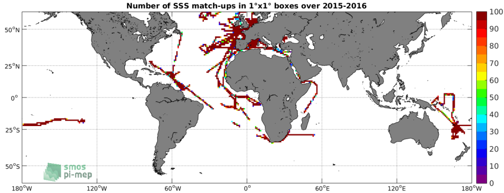
Figure 4: Number of SSS match-ups between TSG-GOSUD-Research-vessel SSS and the SMAP-L3-JPL-V4-MONTHLY-60KM SSS product for the SMOS coastal zone ( \approx 800\text{km} ) 60N-60S Pi-MEP region over 1^\circ \times 1^\circ boxes and for the full satellite product period.
