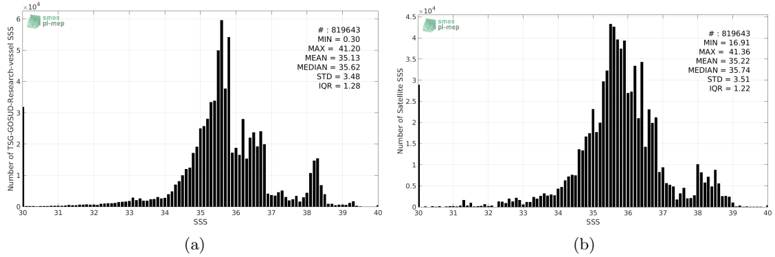
Figure 2: Histograms of SSS from TSG-GOSUD-Research-vessel (a) and SMAP-L3-JPL-V4-MONTHLY-60KM (b) considering all match-up pairs per bins of 0.1 over the SMOS coastal zone ( \approx 800\text{km} ) 60N-60S Pi-MEP region and for the full satellite product period.
