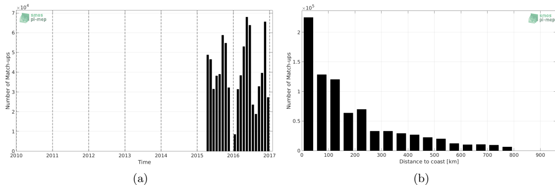
Figure 1: Number of match-ups between TSG-GOSUD-Research-vessel and SMAP-L3-JPL-V4-MONTHLY-60KM SSS as a function of time (a) and as function of the distance to coast (b) over the SMOS coastal zone ( \approx 800 km) 60N-60S Pi-MEP region and for the full satellite product period.
