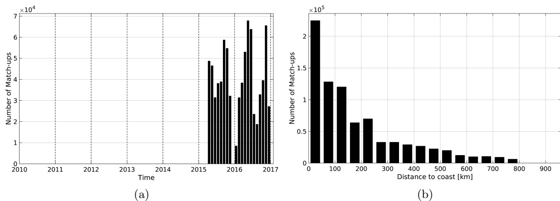
Figure 1: Number of match-ups between TSG-GOSUD-Research-vessel and SMAP-L3-JPL-V4-MONTHLY-60KM SSS as a function of time (a) and as function of the distance to coast (b) over the SMOS coastal zone ( \pm 800 km) 60N-60S Pi-MEP region and for the full satellite product period.
