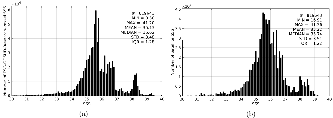
Figure 2: Histograms of SSS from TSG-GOSUD-Research-vessel (a) and SMAP-L3-JPL-V4-MONTHLY-60KM (b) considering all match-up pairs per bins of 0.1 over the SMOS coastal zone ( \pm 800\text{km} ) 60N-60S Pi-MEP region and for the full satellite product period.
