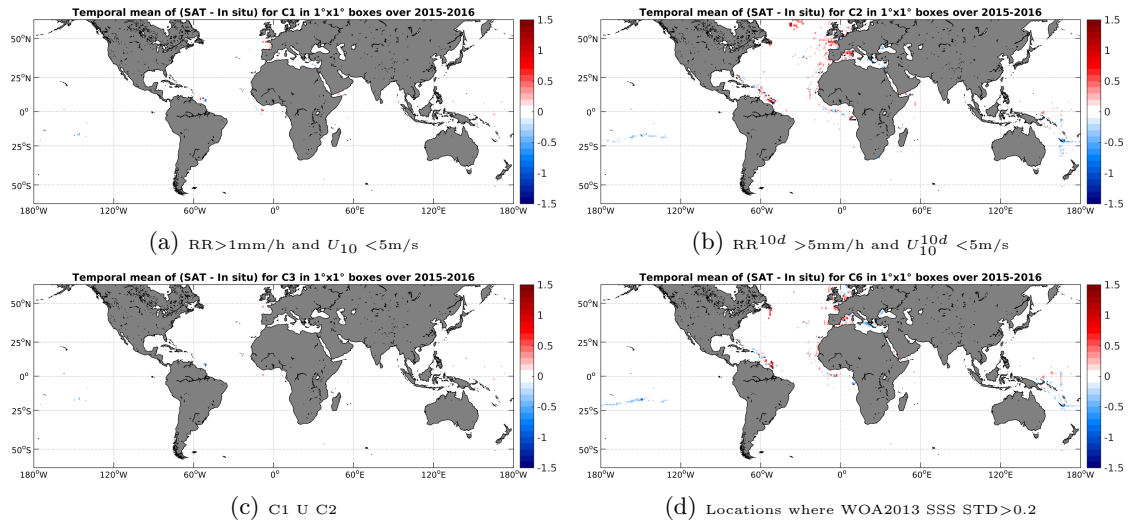
Figure 12: Temporal mean gridded over spatial boxes of size 1^\circ \times 1^\circ of \Delta SSS (SMAP-L3-JPL-V4-MONTHLY-60KM - TSG-GOSUD-Research-vessel) for 4 different subdatasets corresponding to: RR > 1\text{mm/h} and U_{10} < 5\text{m/s} (a), RR^{10d} > 5\text{mm/h} and U_{10}^{10d} < 5\text{m/s} (b), C1 U C2 (c), Locations where WOA2013 SSS STD > 0.2 (d).
