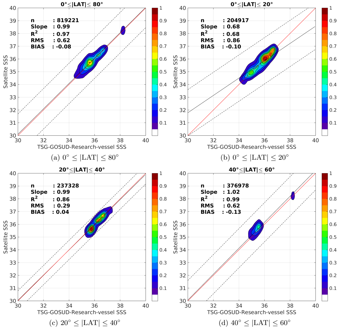
Figure 9: Contour maps of the concentration of SMAP-L3-JPL-V4-MONTHLY-60KM SSS (y-axis) versus TSG-GOSUD-Research-vessel SSS (x-axis) at match-up pairs for different latitude bands. For each plot, the red line shows x=y . The black thin and dashed lines indicate a linear fit through the data cloud and the \pm 95\% confidence levels, respectively. The number match-up pairs n , the slope and R^2 coefficient of the linear fit, the root mean square (RMS) and the mean bias between satellite and in situ data are indicated for each latitude band in each plots.
