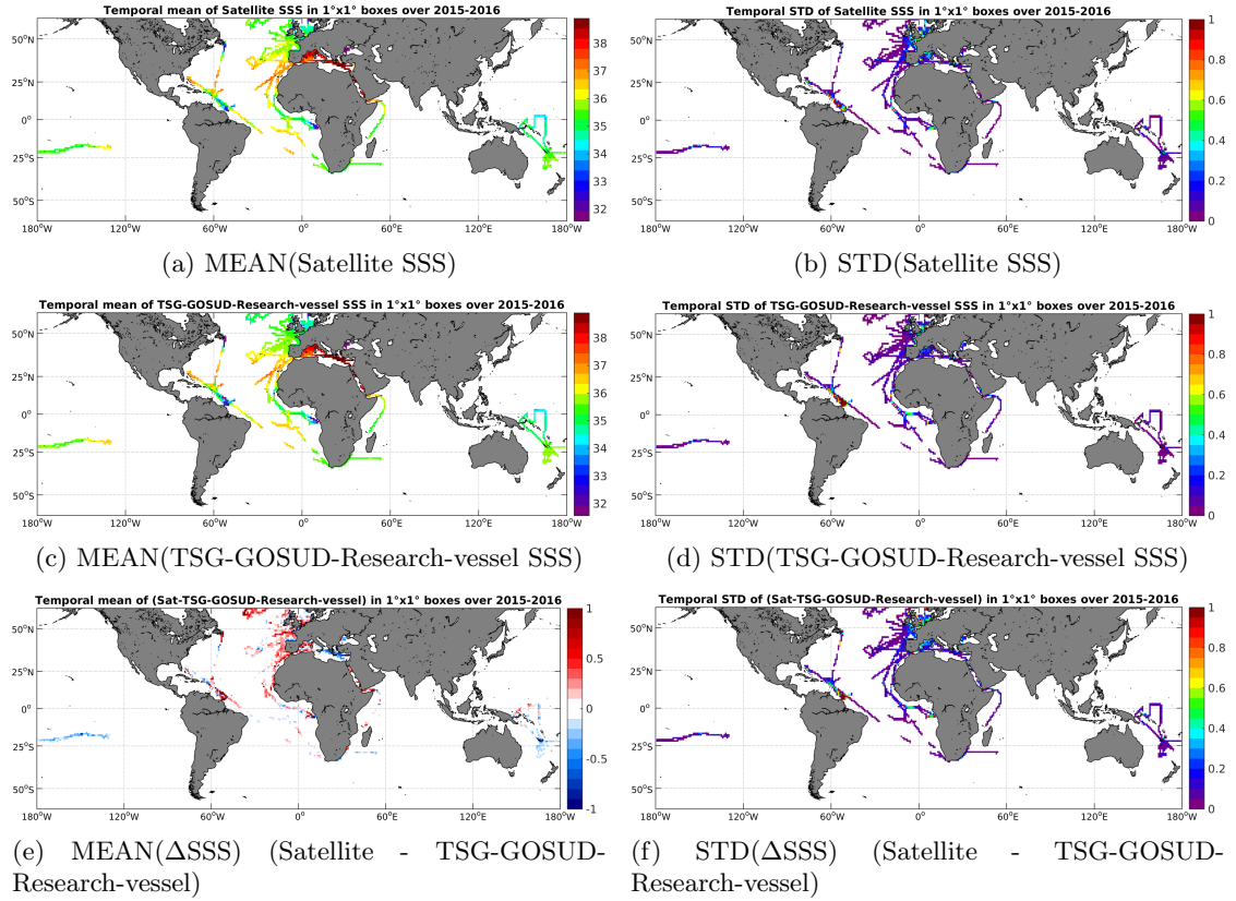
Figure 6: Temporal mean (left) and STD (right) of SSS from SMAP-L3-JPL-V4-MONTHLY-60KM (top), TSG-GOSUD-Research-vessel (middle), and of \Delta SSS (Satellite - TSG-GOSUD-Research-vessel). Only match-up pairs are used to generate these maps.
