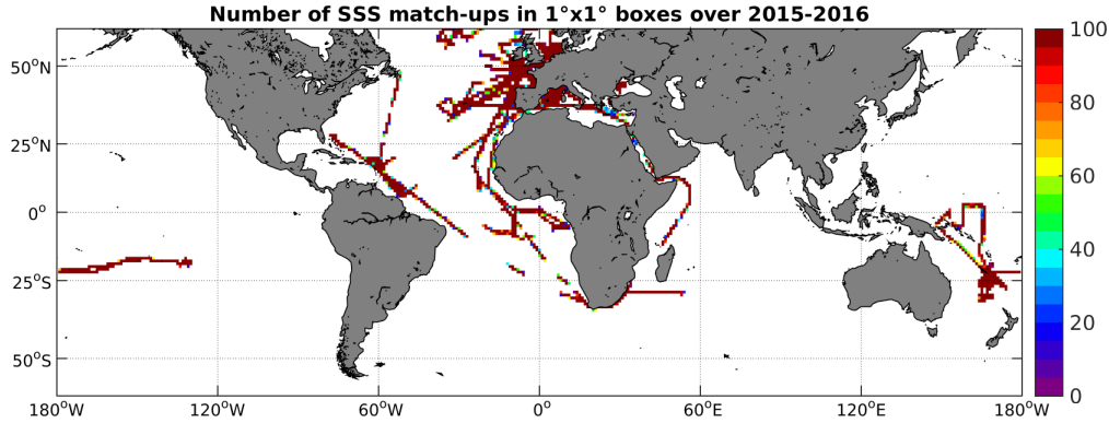
Figure 4: Number of SSS match-ups between TSG-GOSUD-Research-vessel SSS and the SMAP-L3-JPL-V4-MONTHLY-60KM SSS product for the SMOS coastal zone ( \geq 800\text{km} ) 60N-60S Pi-MEP region over 1^\circ \times 1^\circ boxes and for the full satellite product period.
