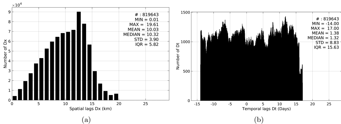
Figure 5: Histograms of the spatial (a) and temporal (b) lags between the time of the TSG-GOSUD-Research-vessel measurements and the date of the corresponding SMAP-L3-JPL-V4-MONTHLY-60KM SSS product.
