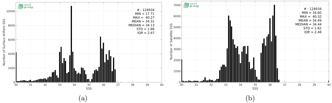
Figure 2: Histograms of SSS from Surface drifters (a) and SMAP-L3-JPL-V4-MONTHLY-60KM (b) considering all match-up pairs per bins of 0.1 over the SMOS coastal zone ( \approx 800\text{km} ) 60N-60S Pi-MEP region and for the full satellite product period.
