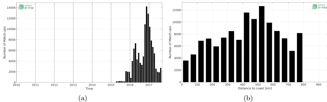
Figure 1: Number of match-ups between Surface drifters and SMAP-L3-JPL-V4-MONTHLY-60KM SSS as a function of time (a) and as function of the distance to coast (b) over the SMOS coastal zone ( \pm 800\text{km} ) 60N-60S Pi-MEP region and for the full satellite product period.
