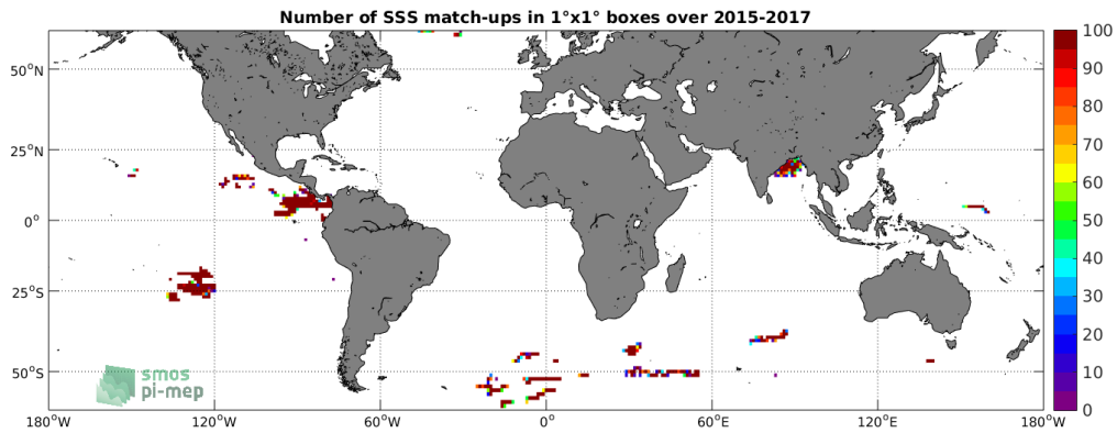
Figure 3: Number of SSS match-ups between Surface drifters SSS and the SMAP-L3-JPL-V4-MONTHLY-60KM SSS product for the SMOS coastal zone ( \approx 800\text{km} ) 60N-60S Pi-MEP region over 1^\circ \times 1^\circ boxes and for the full satellite product period.
