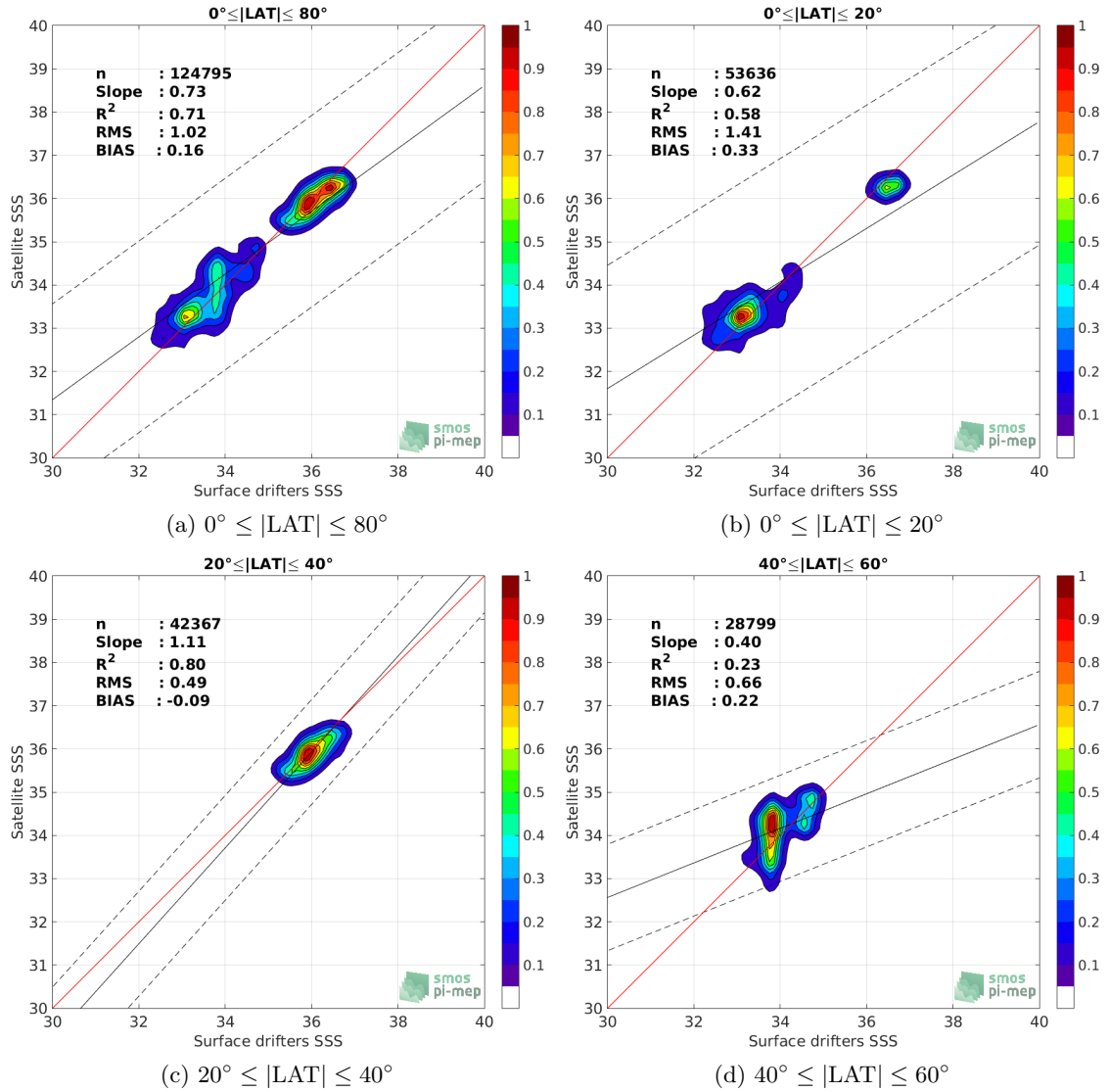
Figure 8: Contour maps of the concentration of SMAP-L3-JPL-V4-MONTHLY-60KM SSS (y-axis) versus Surface drifters SSS (x-axis) at match-up pairs for different latitude bands. For each plot, the red line shows x=y . The black thin and dashed lines indicate a linear fit through the data cloud and the \pm 95\% confidence levels, respectively. The number match-up pairs n , the slope and R^2 coefficient of the linear fit, the root mean square (RMS) and the mean bias between satellite and in situ data are indicated for each latitude band in each plots.
