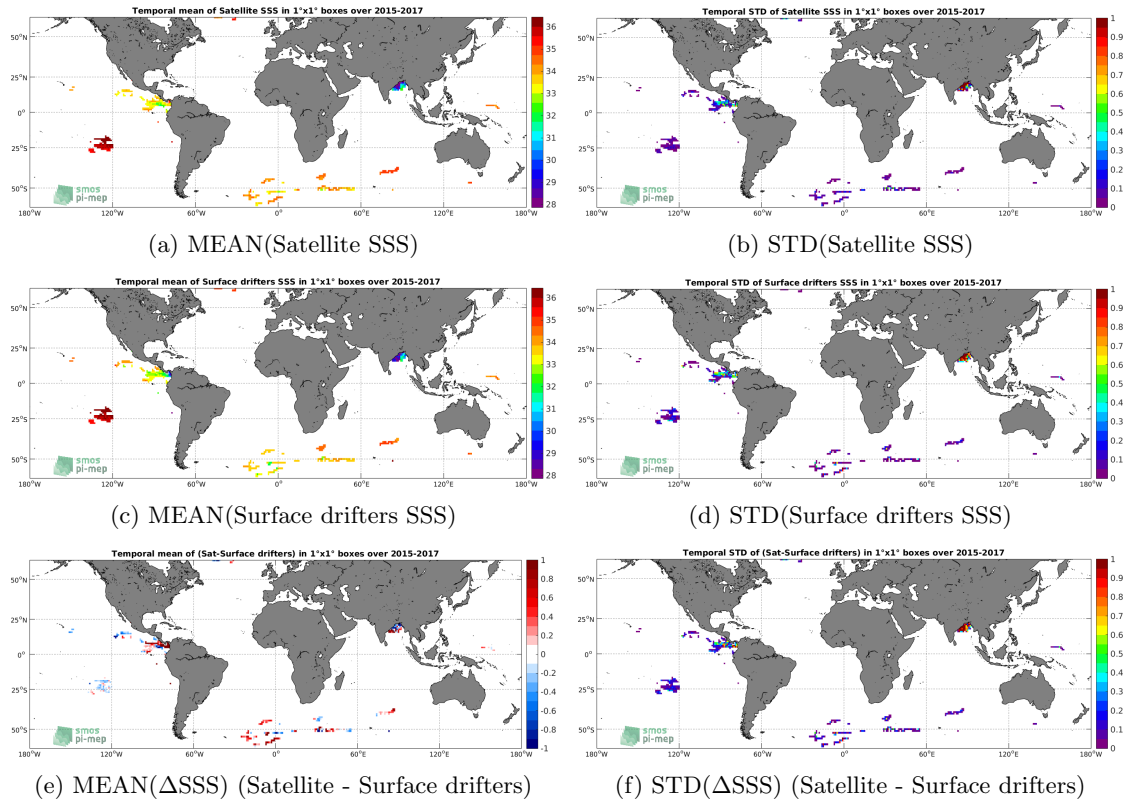
Figure 5: Temporal mean (left) and STD (right) of SSS from SMAP-L3-JPL-V4-MONTHLY-60KM (top), Surface drifters (middle), and of \Delta SSS (Satellite - Surface drifters). Only match-up pairs are used to generate these maps.
