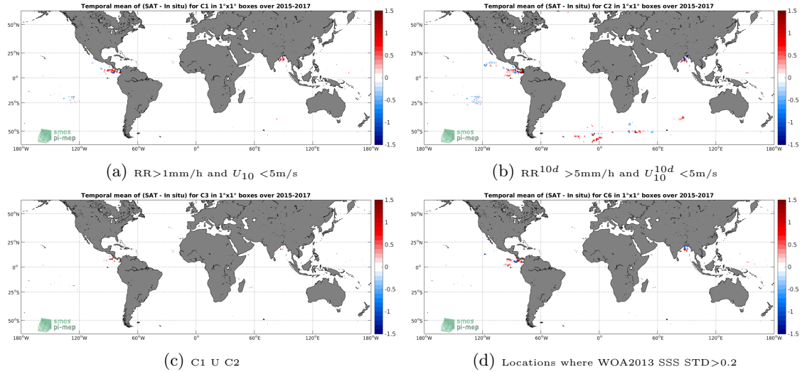
Figure 11: Temporal mean gridded over spatial boxes of size 1^\circ \times 1^\circ of \Delta\text{SSS} (SMAP-L3-JPL-V4-MONTHLY-60KM - Surface drifters) for 4 different subdatasets corresponding to: RR > 1\text{mm/h} and U_{10} < 5\text{m/s} (a), RR^{10d} > 5\text{mm/h} and U_{10}^{10d} < 5\text{m/s} (b), C1 U C2 (c), Locations where WOA2013 SSS STD > 0.2 (d).
