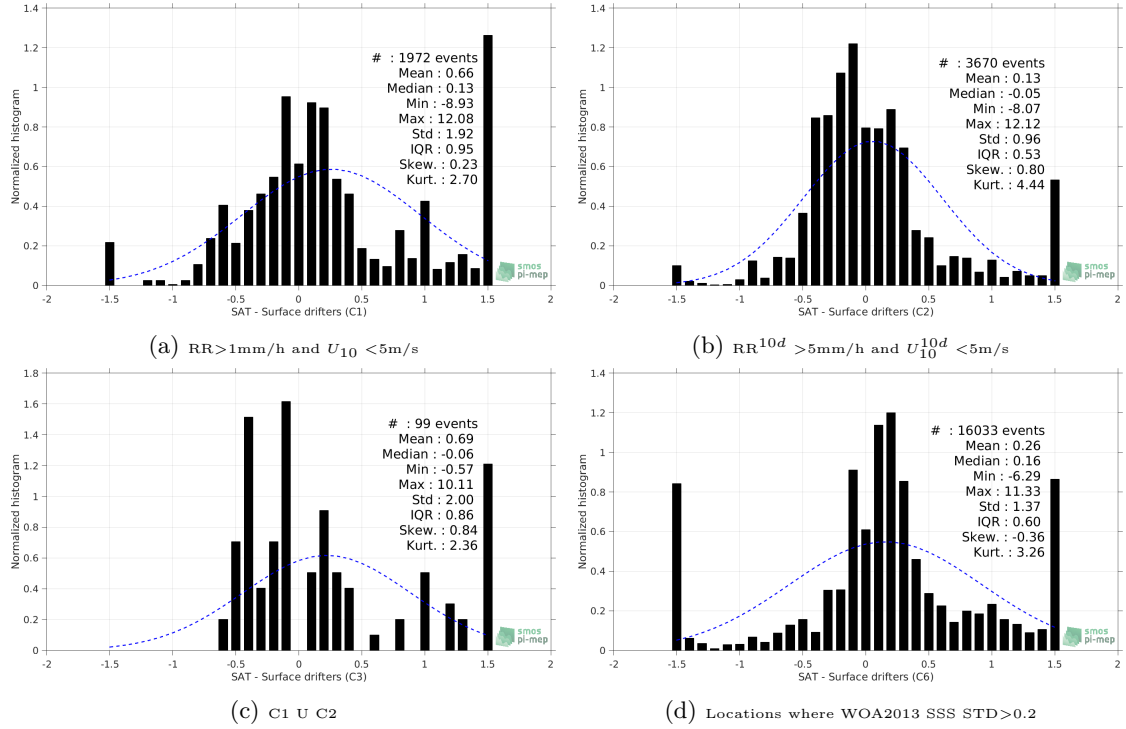
Figure 12: Normalized histogram of \Delta SSS (SMAP-L3-JPL-V4-MONTHLY-60KM - Surface drifters) for 6 different subdatasets corresponding to: RR > 1mm/h and U_{10} < 5 m/s (a), RR^{10d} > 5 mm/h and U_{10}^{10d} < 5 m/s (b), C1 U C2 (c), Locations where WOA2013 SSS STD > 0.2 (d).
