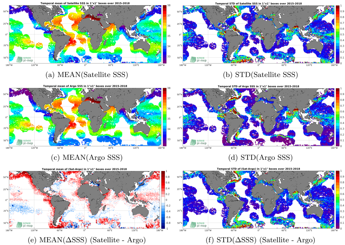
Figure 6: Temporal mean (left) and STD (right) of SSS from SMAP-L3-JPL-V4-MONTHLY-60KM (top), Argo (middle), and of \Delta SSS (Satellite - Argo). Only match-up pairs are used to generate these maps.
