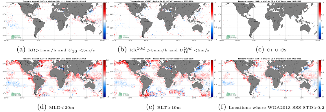
Figure 12: Temporal mean gridded over spatial boxes of size 1^\circ \times 1^\circ of \Delta\text{SSS} (SMAP-L3-JPL-V4-MONTHLY-60KM - Argo) for 6 different subdatasets corresponding to: \text{RR} > 1\text{mm/h} and U_{10} < 5\text{m/s} (a), \text{RR}^{10d} > 5\text{mm/h} and U_{10}^{10d} < 5\text{m/s} (b), C1 U C2 (c), \text{MLD} < 20\text{m} (d), \text{BLT} > 10\text{m} (e), Locations where WOA2013 SSS \text{STD} > 0.2 (f).
