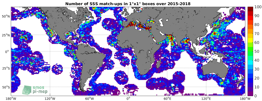
Figure 4: Number of SSS match-ups between Argo SSS and the SMAP-L3-JPL-V4-MONTHLY-60KM SSS product for the SMOS coastal zone ( \approx 800 km) 60N-60S Pi-MEP region over 1^\circ \times 1^\circ boxes and for the full satellite product period.
