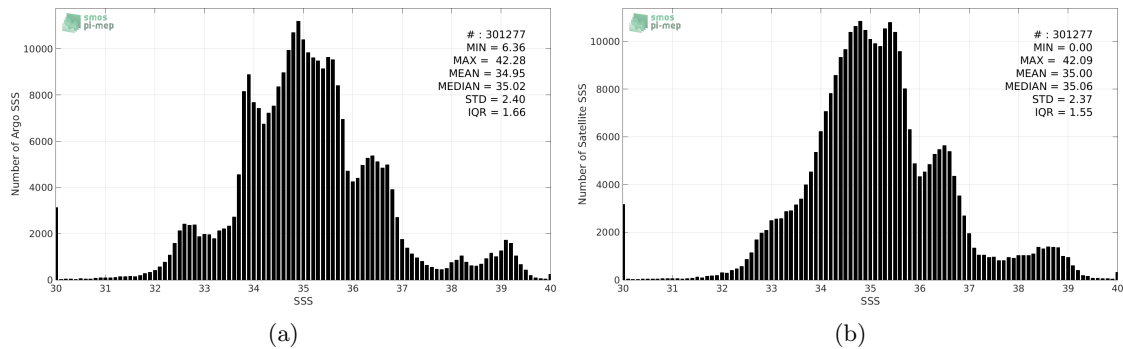
Figure 2: Histograms of SSS from Argo (a) and SMAP-L3-JPL-V4-MONTHLY-60KM (b) considering all match-up pairs per bins of 0.1 over the SMOS coastal zone ( \leq 800 km) 60N-60S Pi-MEP region and for the full satellite product period.
