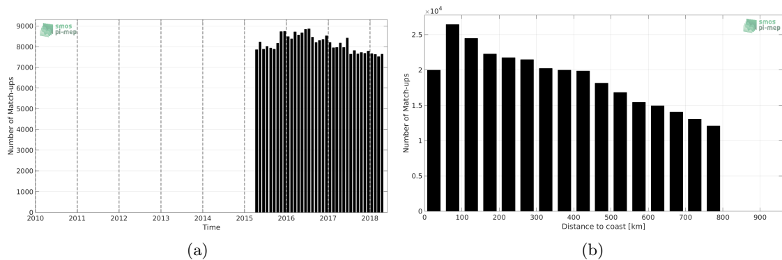
Figure 1: Number of match-ups between Argo and SMAP-L3-JPL-V4-MONTHLY-60KM SSS as a function of time (a) and as function of the distance to coast (b) over the SMOS coastal zone ( \leq 800 km) 60N-60S Pi-MEP region and for the full satellite product period.
