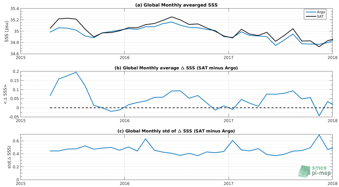
Figure 7: Time series of the monthly averaged mean SSS (top), mean \Delta \text{SSS} (Satellite - Argo) and STD of \Delta \text{SSS} (Satellite - Argo) over the SMOS coastal zone ( \pm 800\text{km} ) 60N-60S Pi-MEP region considering all match-ups collected by the Pi-MEP platform.
