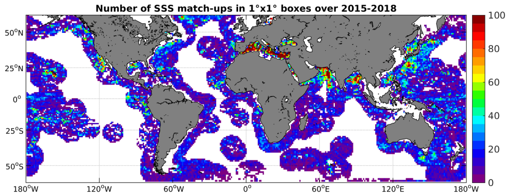
Figure 4: Number of SSS match-ups between Argo SSS and the SMAP-L3-JPL-V4-MONTHLY-60KM SSS product for the SMOS coastal zone ( \approx 800\text{km} ) 60N-60S Pi-MEP region over 1^\circ \times 1^\circ boxes and for the full satellite product period.
