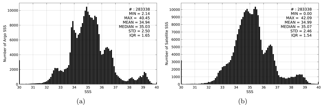
Figure 2: Histograms of SSS from Argo (a) and SMAP-L3-JPL-V4-MONTHLY-60KM (b) considering all match-up pairs per bins of 0.1 over the SMOS coastal zone ( \geq 800\text{km} ) 60N-60S Pi-MEP region and for the full satellite product period.
