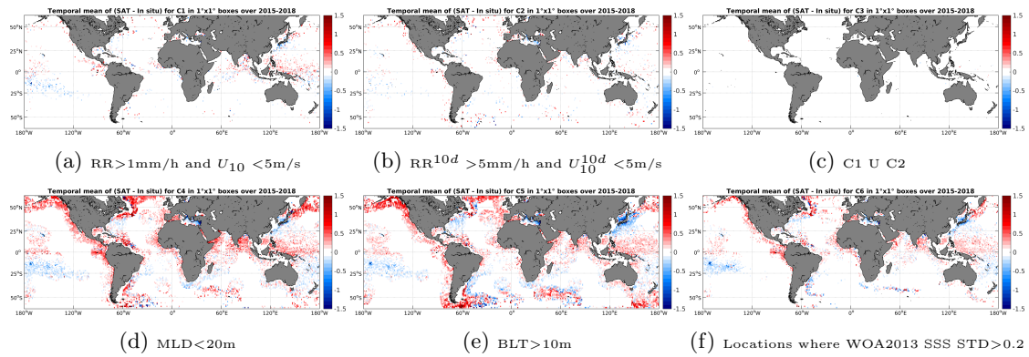
Figure 12: Temporal mean gridded over spatial boxes of size 1^\circ \times 1^\circ of \Delta SSS (SMAP-L3-JPL-V4-MONTHLY-60KM - Argo) for 6 different subdatasets corresponding to: RR > 1\text{mm/h} and U_{10} < 5\text{m/s} (a), RR^{10d} > 5\text{mm/h} and U_{10}^{10d} < 5\text{m/s} (b), C1 U C2 (c), MLD < 20\text{m} (d), BLT > 10\text{m} (e), Locations where WOA2013 SSS STD > 0.2 (f).
