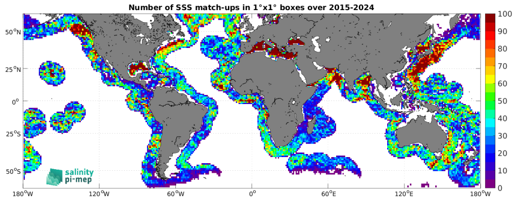
Figure 5: Number of SSS match-ups between Argo SSS and the SMAP SSS L2-AVERAGED v6 (RSS) SSS product for the SMOS coastal zone ( <800\text{km} ) 60N-60S Pi-MEP region over 1^\circ \times 1^\circ boxes and for the full satellite product period.
