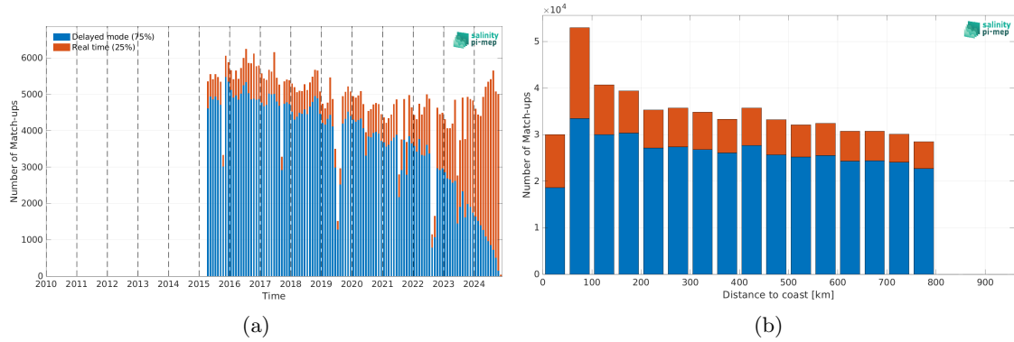
Figure 2: Number of match-ups between Argo and SMAP SSS L2-AVERAGED v6 (RSS) SSS as a function of time (a) and as function of the distance to coast (b) over the SMOS coastal zone (<800km) 60N-60S Pi-MEP region and for the full satellite product period.
