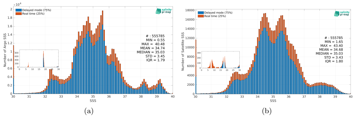
Figure 3: Histograms of SSS from Argo (a) and SMAP SSS L2-AVERAGED v6 (RSS) (b) considering all match-up pairs per bins of 0.1 over the SMOS coastal zone (<800km) 60N-60S Pi-MEP region and for the full satellite product period.
