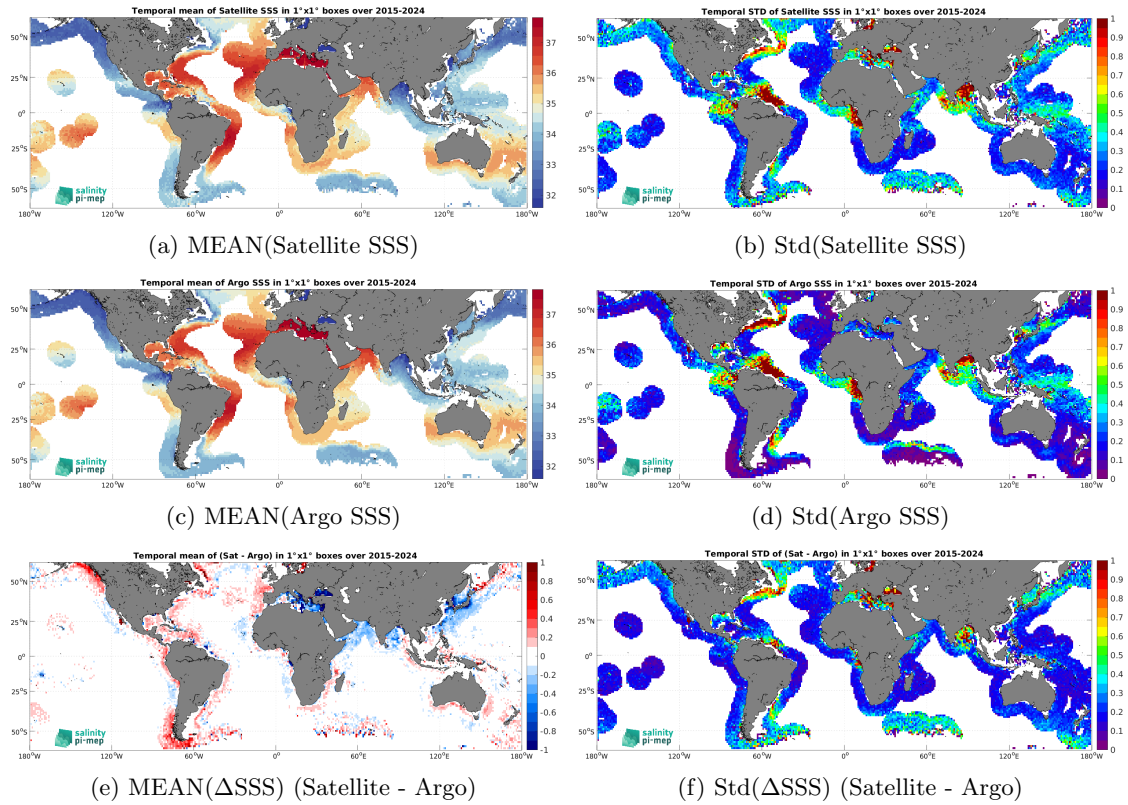
Figure 7: Temporal mean (left) and Std (right) of SSS from SMAP SSS L2-AVERAGED v6 (RSS) (top), Argo (middle), and of \Delta SSS (Satellite - Argo). Only match-up pairs are used to generate these maps.
