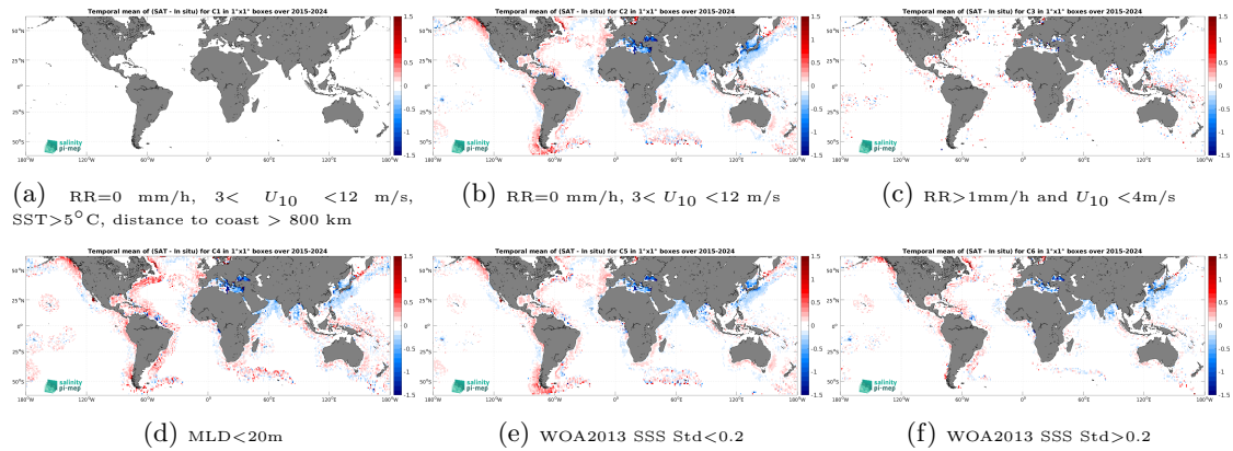
Figure 14: Temporal mean gridded over spatial boxes of size 1^\circ \times 1^\circ of \Delta SSS (SMAP SSS L2-AVERAGED v6 (RSS) - Argo) for 6 different subdatasets corresponding to:RR=0 mm/h, 3 < U_{10} < 12 m/s, SST > 5^\circ\text{C} , distance to coast > 800 km (a), RR=0 mm/h, 3 < U_{10} < 12 m/s (b), RR > 1 mm/h and U_{10} < 4 m/s (c),MLD < 20 m (d),WOA2013 SSS Std < 0.2 (e),WOA2013 SSS Std > 0.2 (f).
