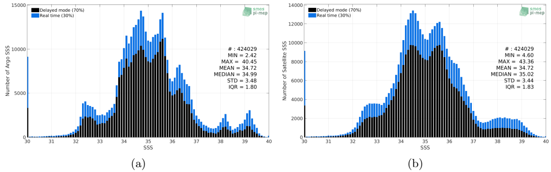
Figure 2: Histograms of SSS from Argo (a) and SMAP SSS L2-AVERAGED v5 (RSS) (b) considering all match-up pairs per bins of 0.1 over the SMOS coastal zone (<800km) 60N-60S Pi-MEP region and for the full satellite product period.
