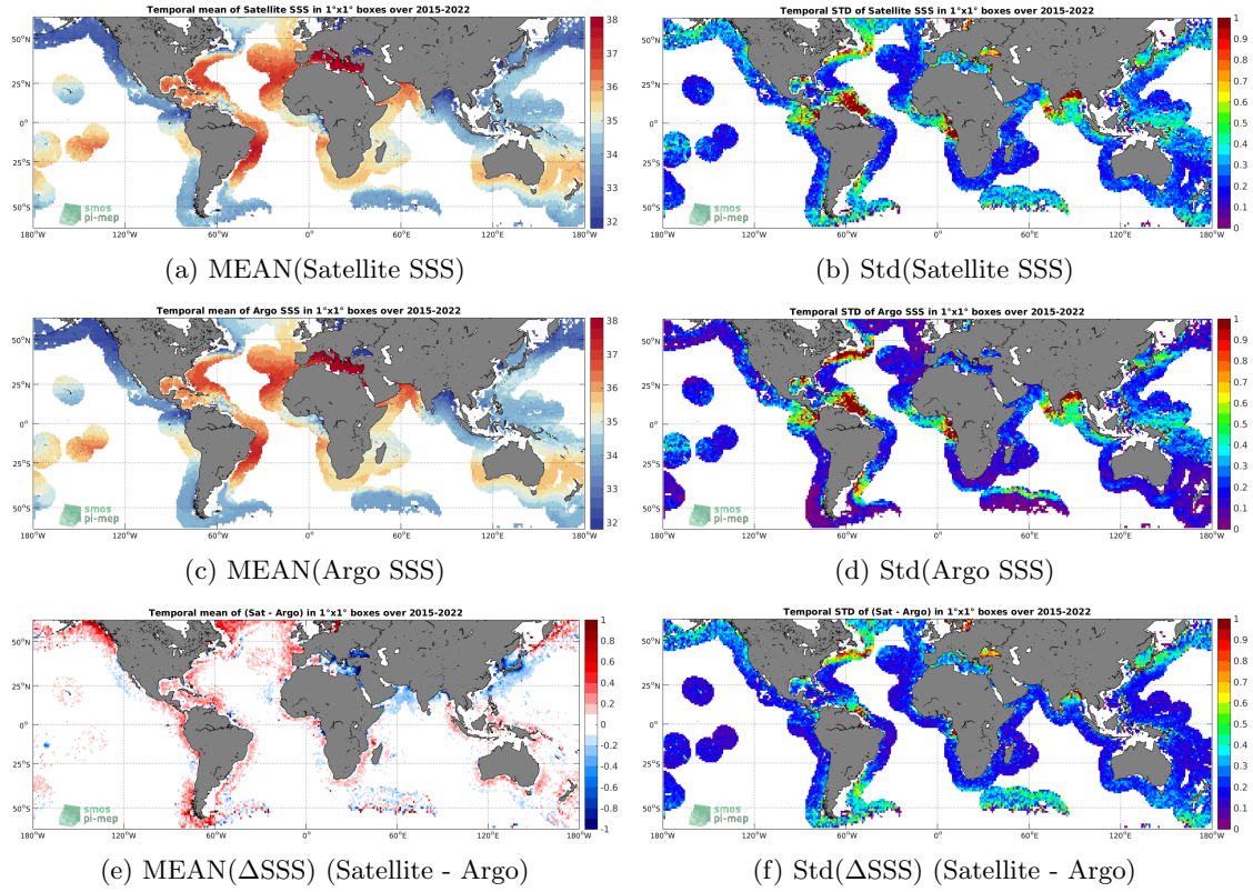
Figure 6: Temporal mean (left) and Std (right) of SSS from SMAP SSS L2-AVERAGED v5 (RSS) (top), Argo (middle), and of \Delta SSS (Satellite - Argo). Only match-up pairs are used to generate these maps.
