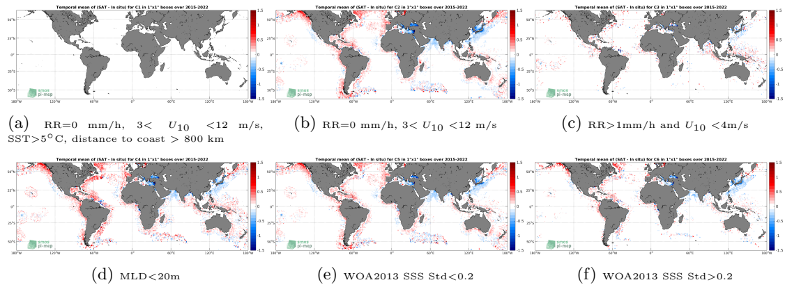
Figure 12: Temporal mean gridded over spatial boxes of size 1^\circ \times 1^\circ of \Delta SSS (SMAP SSS L2-AVERAGED v5 (RSS) - Argo) for 6 different subdatasets corresponding to:RR=0 mm/h, 3 < U_{10} < 12 m/s, SST >5^\circ C, distance to coast > 800 km (a), RR=0 mm/h, 3 < U_{10} < 12 m/s (b), RR >1 mm/h and U_{10} < 4 m/s (c),MLD <20 m (d),WOA2013 SSS Std <0.2 (e),WOA2013 SSS Std >0.2 (f).
