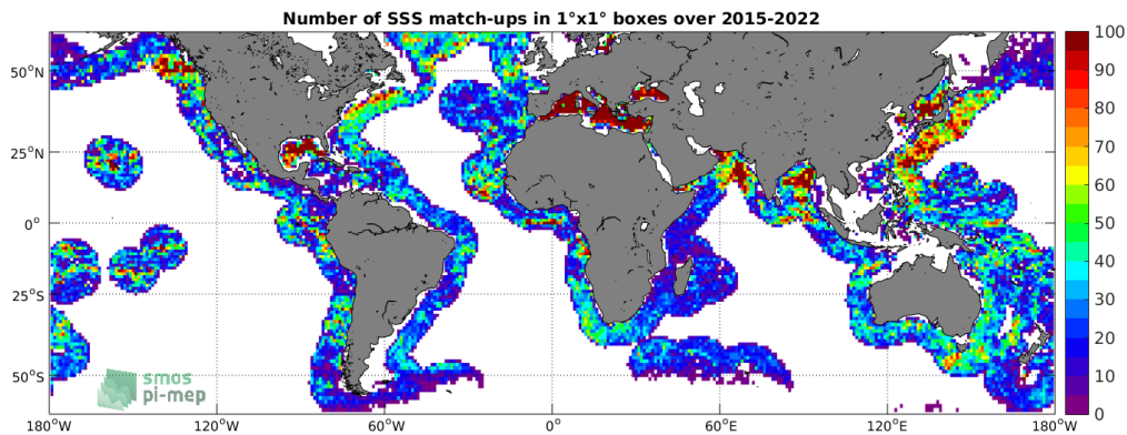
Figure 4: Number of SSS match-ups between Argo SSS and the SMAP SSS L2-AVERAGED v5 (RSS) SSS product for the SMOS coastal zone (<800km) 60N-60S Pi-MEP region over 1^\circ \times 1^\circ boxes and for the full satellite product period.
