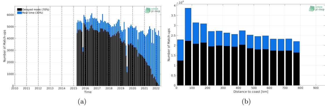
Figure 1: Number of match-ups between Argo and SMAP SSS L2-AVERAGED v5 (RSS) SSS as a function of time (a) and as function of the distance to coast (b) over the SMOS coastal zone (<800km) 60N-60S Pi-MEP region and for the full satellite product period.
