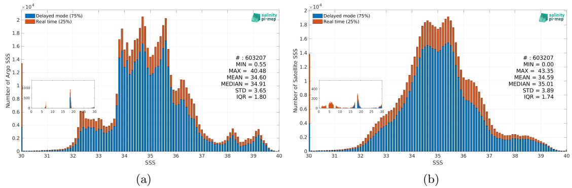
Figure 3: Histograms of SSS from Argo (a) and SMAP SSS L2-AVERAGED v5.0 (JPL) (b) considering all match-up pairs per bins of 0.1 over the SMOS coastal zone (<800km) 60N-60S Pi-MEP region and for the full satellite product period.
