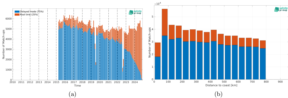
Figure 2: Number of match-ups between Argo and SMAP SSS L2-AVERAGED v5.0 (JPL) SSS as a function of time (a) and as function of the distance to coast (b) over the SMOS coastal zone ( < 800\text{km} ) 60N-60S Pi-MEP region and for the full satellite product period.
