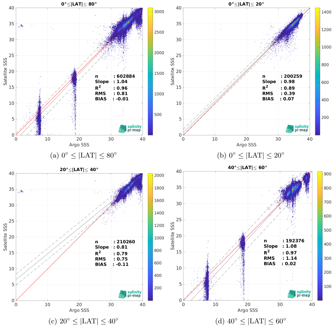
Figure 10: Contour maps of the concentration of SMAP SSS L2-AVERAGED v5.0 (JPL) SSS (y-axis) versus Argo SSS (x-axis) at match-up pairs for different latitude bands. For each plot, the red line shows x=y . The black thin and dashed lines indicate a linear fit through the data cloud and the \pm 95\% confidence levels, respectively. The number match-up pairs n , the slope and R^2 coefficient of the linear fit, the root mean square (RMS) and the mean bias between satellite and in situ data are indicated for each latitude band in each plots.
