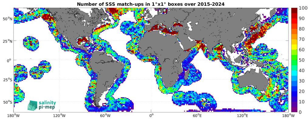
Figure 5: Number of SSS match-ups between Argo SSS and the SMAP SSS L2-AVERAGED v5.0 (JPL) SSS product for the SMOS coastal zone (<800km) 60N-60S Pi-MEP region over 1^\circ \times 1^\circ boxes and for the full satellite product period.
