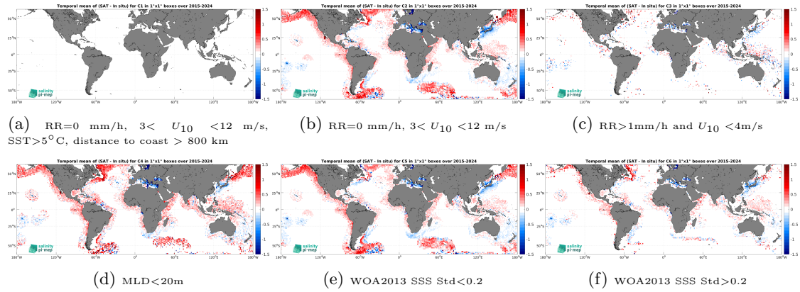
Figure 14: Temporal mean gridded over spatial boxes of size 1^\circ \times 1^\circ of \Delta SSS (SMAP SSS L2-AVERAGED v5.0 (JPL) - Argo) for 6 different subdatasets corresponding to:RR=0 mm/h, 3 < U_{10} < 12 m/s, SST >5^\circ C, distance to coast > 800 km (a), RR=0 mm/h, 3 < U_{10} < 12 m/s (b), RR >1 mm/h and U_{10} < 4 m/s (c),MLD <20 m (d),WOA2013 SSS Std <0.2 (e),WOA2013 SSS Std >0.2 (f).
