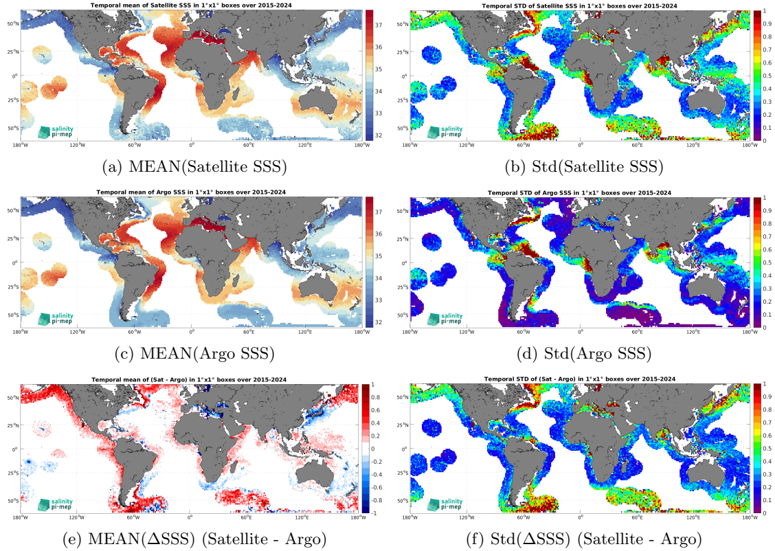
Figure 7: Temporal mean (left) and Std (right) of SSS from SMAP SSS L2-AVERAGED v5.0 (JPL) (top), Argo (middle), and of \Delta SSS (Satellite - Argo). Only match-up pairs are used to generate these maps.
