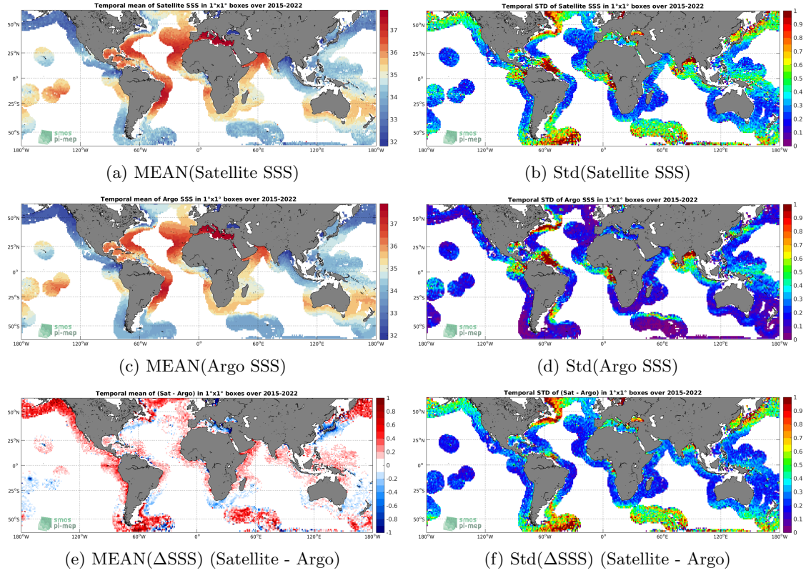
Figure 6: Temporal mean (left) and Std (right) of SSS from SMAP SSS L2-AVERAGED v5.0 (JPL) (top), Argo (middle), and of \Delta SSS (Satellite - Argo). Only match-up pairs are used to generate these maps.
