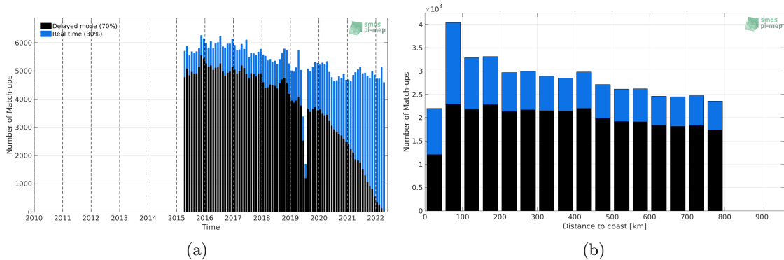
Figure 1: Number of match-ups between Argo and SMAP SSS L2-AVERAGED v5.0 (JPL) SSS as a function of time (a) and as function of the distance to coast (b) over the SMOS coastal zone (<800km) 60N-60S Pi-MEP region and for the full satellite product period.
