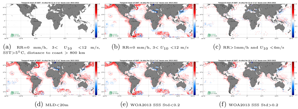
Figure 12: Temporal mean gridded over spatial boxes of size 1^\circ \times 1^\circ of \Delta SSS (SMAP SSS L2-AVERAGED v5.0 (JPL) - Argo) for 6 different subdatasets corresponding to:RR=0 mm/h, 3 < U_{10} < 12 m/s, SST >5^\circ C, distance to coast > 800 km (a), RR=0 mm/h, 3 < U_{10} < 12 m/s (b), RR >1 mm/h and U_{10} < 4 m/s (c),MLD <20 m (d),WOA2013 SSS Std <0.2 (e),WOA2013 SSS Std >0.2 (f).
