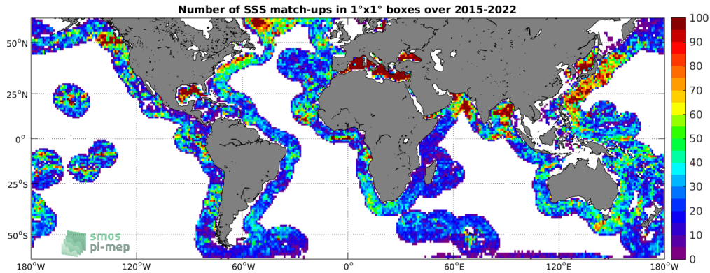
Figure 4: Number of SSS match-ups between Argo SSS and the SMAP SSS L2-AVERAGED v5.0 (JPL) SSS product for the SMOS coastal zone (<800km) 60N-60S Pi-MEP region over 1^\circ \times 1^\circ boxes and for the full satellite product period.
