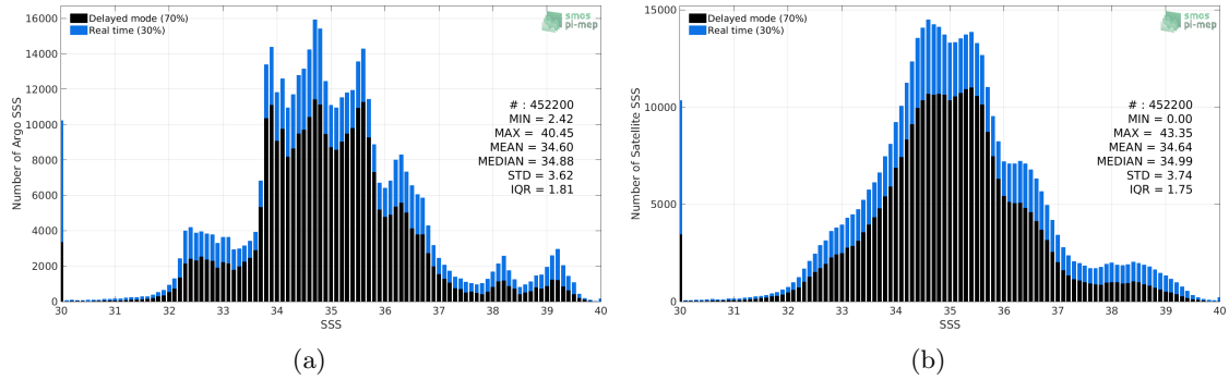
Figure 2: Histograms of SSS from Argo (a) and SMAP SSS L2-AVERAGED v5.0 (JPL) (b) considering all match-up pairs per bins of 0.1 over the SMOS coastal zone (<800km) 60N-60S Pi-MEP region and for the full satellite product period.
