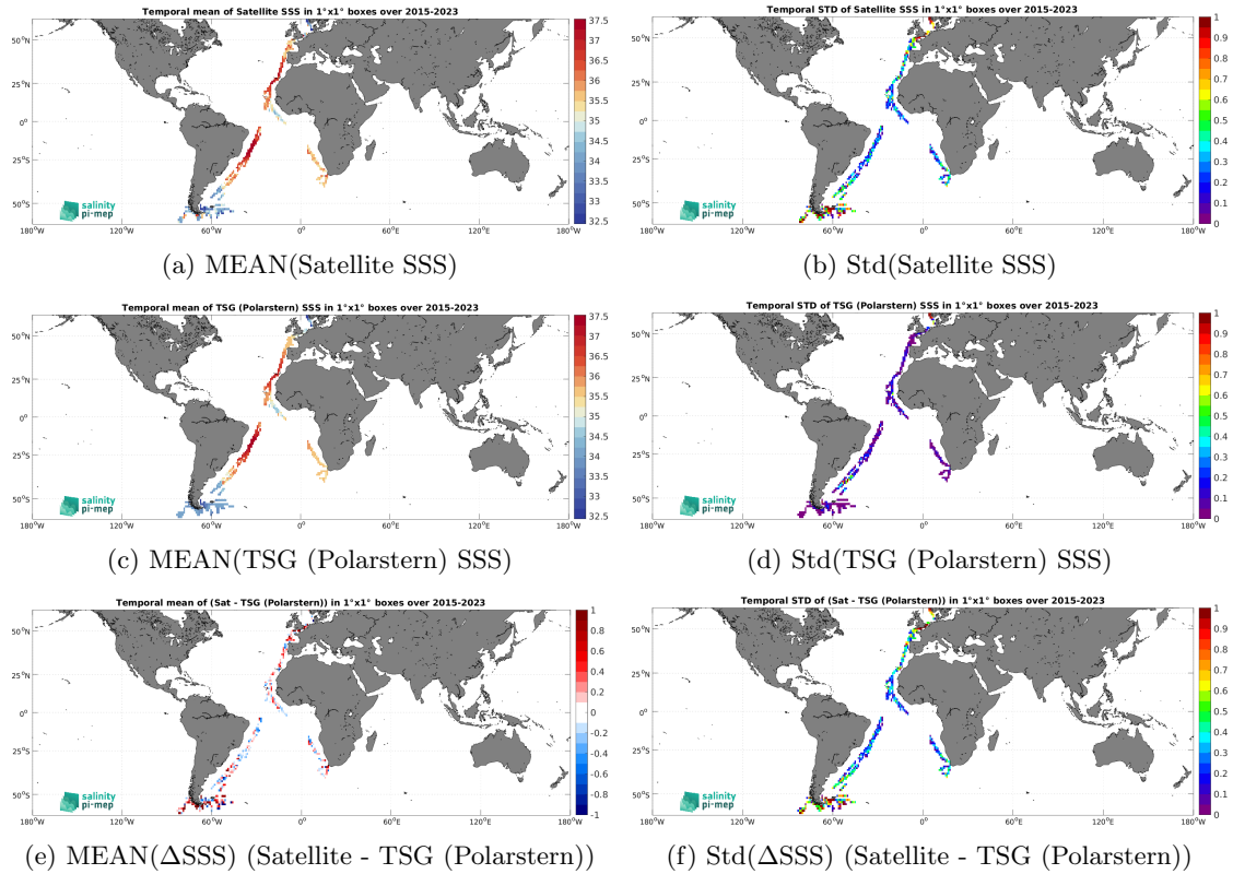
Figure 7: Temporal mean (left) and Std (right) of SSS from SMAP SSS L2 v6 (RSS) (top), TSG (Polarstern) (middle), and of \Delta SSS (Satellite - TSG (Polarstern)). Only match-up pairs are used to generate these maps.
