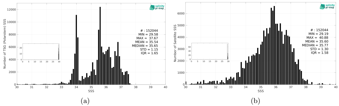
Figure 3: Histograms of SSS from TSG (Polarstern) (a) and SMAP SSS L2 v6 (RSS) (b) considering all match-up pairs per bins of 0.1 over the SMOS coastal zone (<800km) 60N-60S Pi-MEP region and for the full satellite product period.
