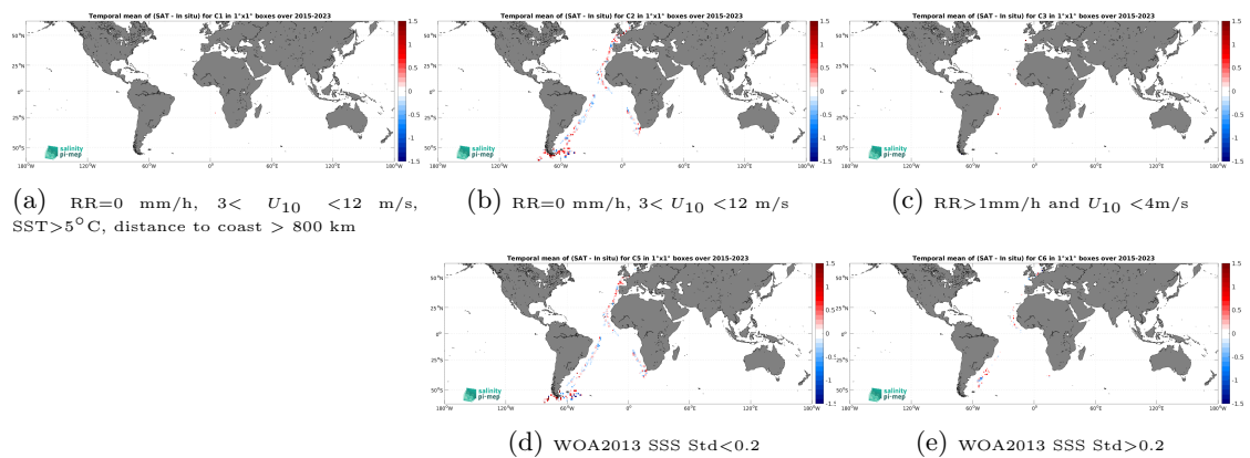
Figure 14: Temporal mean gridded over spatial boxes of size 1^\circ \times 1^\circ of \Delta SSS (SMAP SSS L2 v6 (RSS) - TSG (Polarstern)) for 5 different subdatasets corresponding to:RR=0 mm/h, 3 < U_{10} < 12 m/s, SST>5°C, distance to coast > 800 km (a), RR=0 mm/h, 3 < U_{10} < 12 m/s (b), RR>1mm/h and U_{10} < 4 m/s (c), WOA2013 SSS Std<0.2 (d), WOA2013 SSS Std>0.2 (e).
