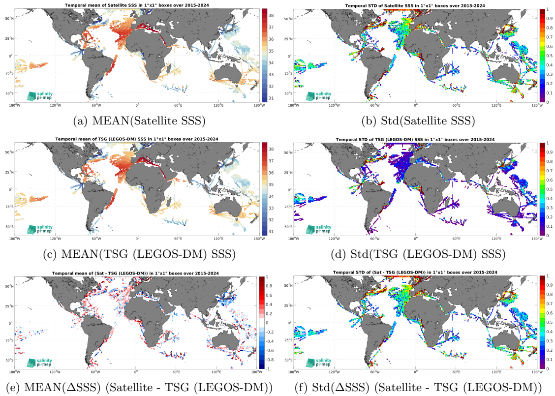
Figure 7: Temporal mean (left) and Std (right) of SSS from SMAP SSS L2 v6 (RSS) (top), TSG (LEGOS-DM) (middle), and of \Delta SSS (Satellite - TSG (LEGOS-DM)). Only match-up pairs are used to generate these maps.
