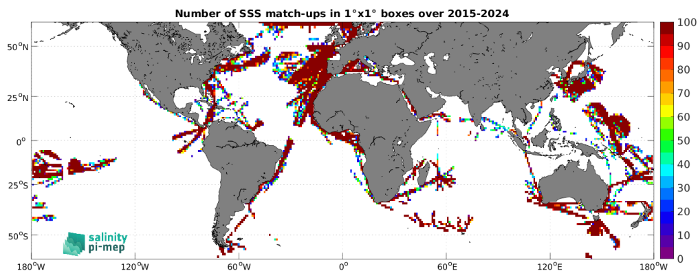
Figure 5: Number of SSS match-ups between TSG (LEGOS-DM) SSS and the SMAP SSS L2 v6 (RSS) SSS product for the SMOS coastal zone (<800km) 60N-60S Pi-MEP region over 1^\circ \times 1^\circ boxes and for the full satellite product period.
