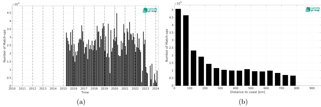
Figure 2: Number of match-ups between TSG (LEGOS-DM) and SMAP SSS L2 v6 (RSS) SSS as a function of time (a) and as function of the distance to coast (b) over the SMOS coastal zone (<800km) 60N-60S Pi-MEP region and for the full satellite product period.
