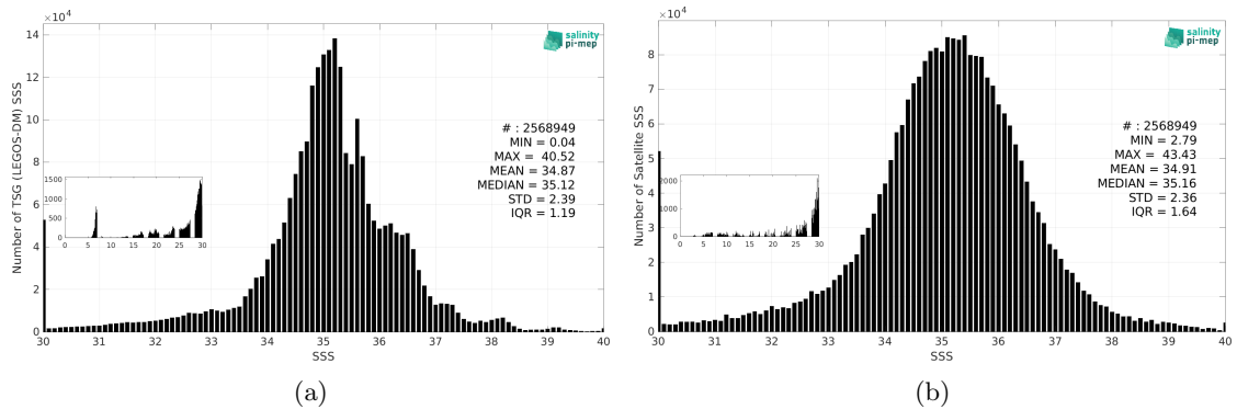
Figure 3: Histograms of SSS from TSG (LEGOS-DM) (a) and SMAP SSS L2 v6 (RSS) (b) considering all match-up pairs per bins of 0.1 over the SMOS coastal zone (<800km) 60N-60S Pi-MEP region and for the full satellite product period.
