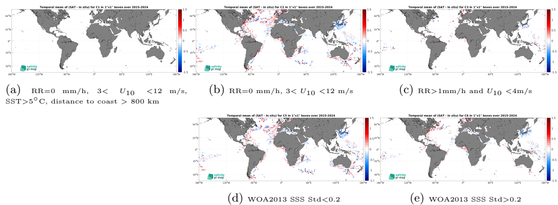
Figure 14: Temporal mean gridded over spatial boxes of size 1^\circ \times 1^\circ of \Delta\text{SSS} (SMAP SSS L2 v6 (RSS) - TSG (LEGOS-DM)) for 5 different subdatasets corresponding to:RR=0 mm/h, 3 < U_{10} < 12 m/s, SST>5°C, distance to coast > 800 km (a), RR=0 mm/h, 3 < U_{10} < 12 m/s (b), RR>1mm/h and U_{10} < 4 m/s (c), WOA2013 SSS Std<0.2 (d), WOA2013 SSS Std>0.2 (e).
