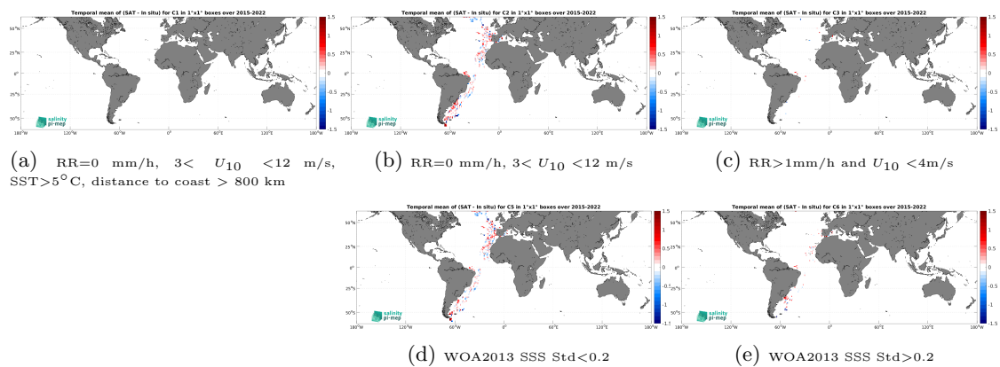
Figure 14: Temporal mean gridded over spatial boxes of size 1^\circ \times 1^\circ of \Delta SSS (SMAP SSS L2 v6 (RSS) - TSG (CSIC-UTM)) for 5 different subdatasets corresponding to:RR=0 mm/h, 3 < U_{10} < 12 m/s, SST >5^\circ\text{C} , distance to coast > 800 km (a), RR=0 mm/h, 3 < U_{10} < 12 m/s (b), RR >1 mm/h and U_{10} < 4 m/s (c), WOA2013 SSS Std <0.2 (d), WOA2013 SSS Std >0.2 (e).
