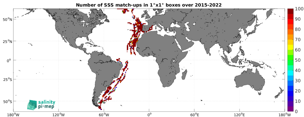
Figure 5: Number of SSS match-ups between TSG (CSIC-UTM) SSS and the SMAP SSS L2 v6 (RSS) SSS product for the SMOS coastal zone (<800km) 60N-60S Pi-MEP region over 1^\circ \times 1^\circ boxes and for the full satellite product period.
