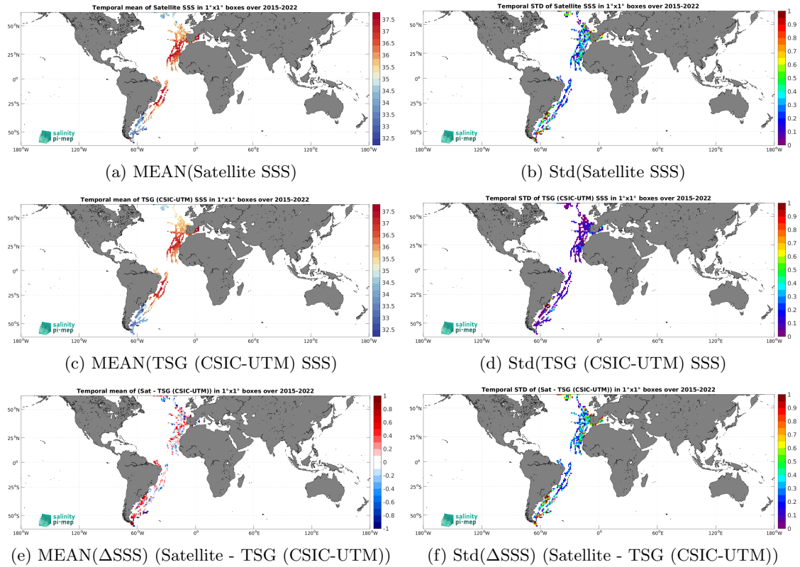
Figure 7: Temporal mean (left) and Std (right) of SSS from SMAP SSS L2 v6 (RSS) (top), TSG (CSIC-UTM) (middle), and of \Delta SSS (Satellite - TSG (CSIC-UTM)). Only match-up pairs are used to generate these maps.
