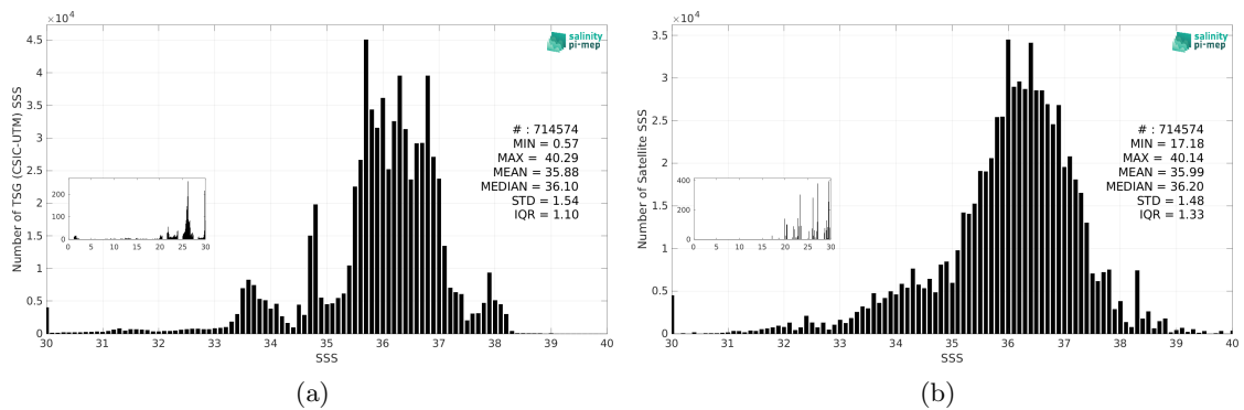
Figure 3: Histograms of SSS from TSG (CSIC-UTM) (a) and SMAP SSS L2 v6 (RSS) (b) considering all match-up pairs per bins of 0.1 over the SMOS coastal zone (<800km) 60N-60S Pi-MEP region and for the full satellite product period.
