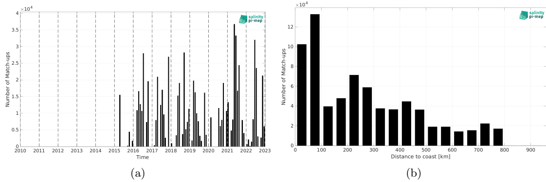
Figure 2: Number of match-ups between TSG (CSIC-UTM) and SMAP SSS L2 v6 (RSS) SSS as a function of time (a) and as function of the distance to coast (b) over the SMOS coastal zone (<800km) 60N-60S Pi-MEP region and for the full satellite product period.
