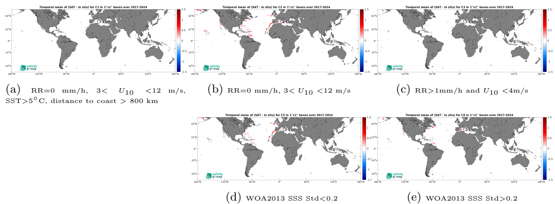
Figure 14: Temporal mean gridded over spatial boxes of size 1^\circ \times 1^\circ of \Delta SSS (SMAP SSS L2 v6 (RSS) - Saldrone) for 5 different subdatasets corresponding to:RR=0 mm/h, 3 < U_{10} < 12 m/s, SST >5^\circ\text{C} , distance to coast > 800 km (a), RR=0 mm/h, 3 < U_{10} < 12 m/s (b), RR >1 mm/h and U_{10} < 4 m/s (c), WOA2013 SSS Std <0.2 (d), WOA2013 SSS Std >0.2 (e).
