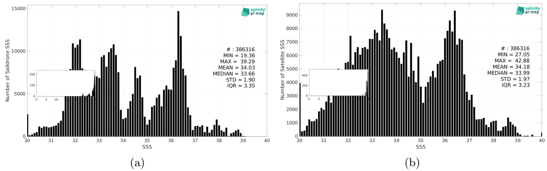
Figure 3: Histograms of SSS from Saildrone (a) and SMAP SSS L2 v6 (RSS) (b) considering all match-up pairs per bins of 0.1 over the SMOS coastal zone ( <800\text{km} ) 60N-60S Pi-MEP region and for the full satellite product period.
