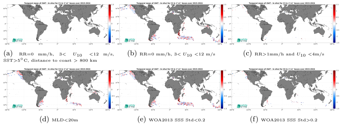
Figure 14: Temporal mean gridded over spatial boxes of size 1^\circ \times 1^\circ of \Delta SSS (SMAP SSS L2 v6 (RSS) - Marine mammals) for 6 different subdatasets corresponding to:RR=0 mm/h, 3 < U_{10} < 12 m/s, SST >5^\circ C, distance to coast > 800 km (a), RR=0 mm/h, 3 < U_{10} < 12 m/s (b), RR >1 mm/h and U_{10} < 4 m/s (c),MLD <20 m (d),WOA2013 SSS Std <0.2 (e),WOA2013 SSS Std >0.2 (f).
