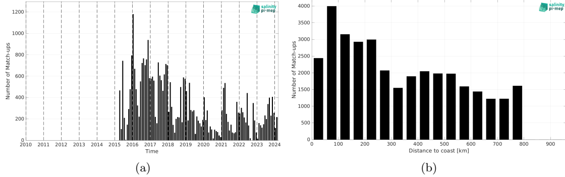
Figure 2: Number of match-ups between Marine mammals and SMAP SSS L2 v6 (RSS) SSS as a function of time (a) and as function of the distance to coast (b) over the SMOS coastal zone (<800km) 60N-60S Pi-MEP region and for the full satellite product period.
