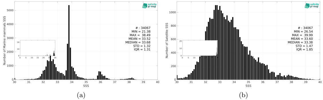
Figure 3: Histograms of SSS from Marine mammals (a) and SMAP SSS L2 v6 (RSS) (b) considering all match-up pairs per bins of 0.1 over the SMOS coastal zone (<800km) 60N-60S Pi-MEP region and for the full satellite product period.
