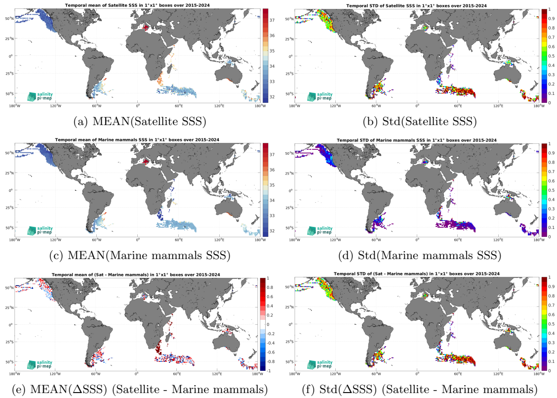
Figure 7: Temporal mean (left) and Std (right) of SSS from SMAP SSS L2 v6 (RSS) (top), Marine mammals (middle), and of \Delta SSS (Satellite - Marine mammals). Only match-up pairs are used to generate these maps.
