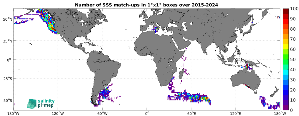
Figure 5: Number of SSS match-ups between Marine mammals SSS and the SMAP SSS L2 v6 (RSS) SSS product for the SMOS coastal zone (<800km) 60N-60S Pi-MEP region over 1^\circ \times 1^\circ boxes and for the full satellite product period.
