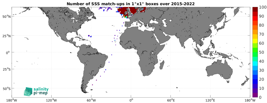
Figure 5: Number of SSS match-ups between ICES SSS and the SMAP SSS L2 v6 (RSS) SSS product for the SMOS coastal zone (<800km) 60N-60S Pi-MEP region over 1^\circ \times 1^\circ boxes and for the full satellite product period.
