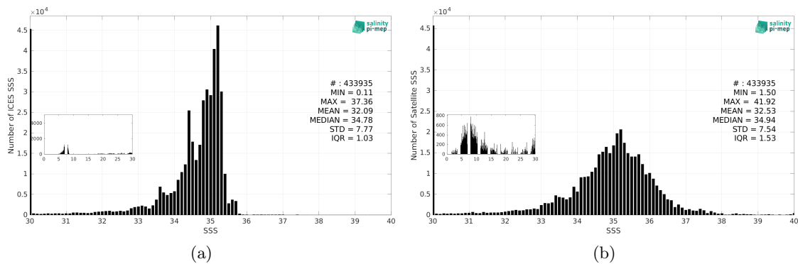
Figure 3: Histograms of SSS from ICES (a) and SMAP SSS L2 v6 (RSS) (b) considering all match-up pairs per bins of 0.1 over the SMOS coastal zone (<800km) 60N-60S Pi-MEP region and for the full satellite product period.
