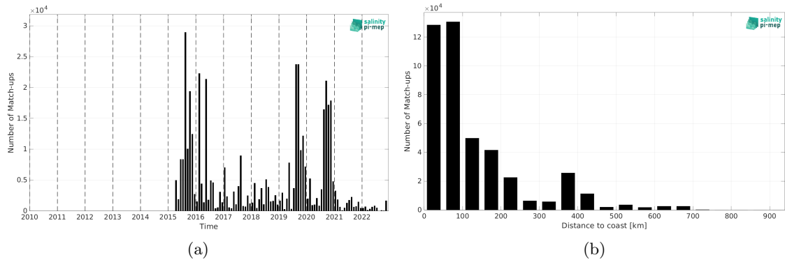
Figure 2: Number of match-ups between ICES and SMAP SSS L2 v6 (RSS) SSS as a function of time (a) and as function of the distance to coast (b) over the SMOS coastal zone (<800km) 60N-60S Pi-MEP region and for the full satellite product period.
