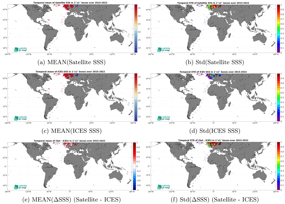
Figure 7: Temporal mean (left) and Std (right) of SSS from SMAP SSS L2 v6 (RSS) (top), ICES (middle), and of \Delta SSS (Satellite - ICES). Only match-up pairs are used to generate these maps.
