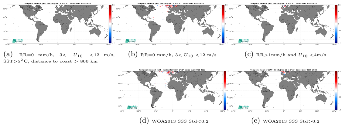
Figure 14: Temporal mean gridded over spatial boxes of size 1^\circ \times 1^\circ of \Delta SSS (SMAP SSS L2 v6 (RSS) - ICES) for 5 different subdatasets corresponding to:RR=0 mm/h, 3 < U_{10} < 12 m/s, SST >5^\circ\text{C} , distance to coast > 800 km (a), RR=0 mm/h, 3 < U_{10} < 12 m/s (b), RR >1 mm/h and U_{10} < 4 m/s (c), WOA2013 SSS Std <0.2 (d), WOA2013 SSS Std >0.2 (e).
