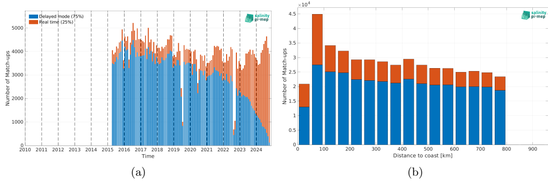
Figure 2: Number of match-ups between Argo and SMAP SSS L2 v6 (RSS) SSS as a function of time (a) and as function of the distance to coast (b) over the SMOS coastal zone (<800km) 60N-60S Pi-MEP region and for the full satellite product period.
