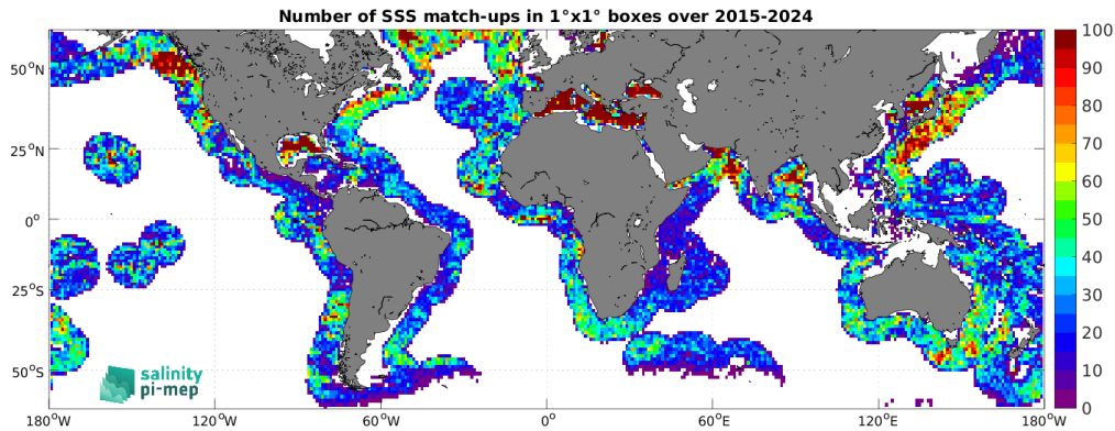
Figure 5: Number of SSS match-ups between Argo SSS and the SMAP SSS L2 v6 (RSS) SSS product for the SMOS coastal zone (<800km) 60N-60S Pi-MEP region over 1^\circ \times 1^\circ boxes and for the full satellite product period.
