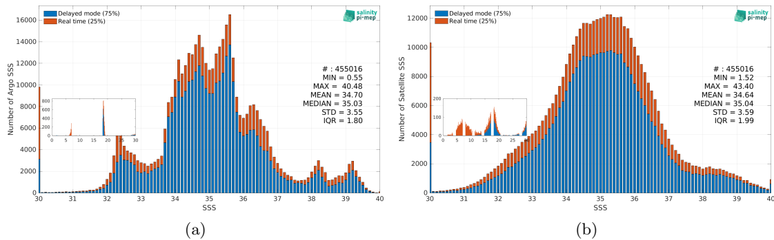
Figure 3: Histograms of SSS from Argo (a) and SMAP SSS L2 v6 (RSS) (b) considering all match-up pairs per bins of 0.1 over the SMOS coastal zone (<800km) 60N-60S Pi-MEP region and for the full satellite product period.
