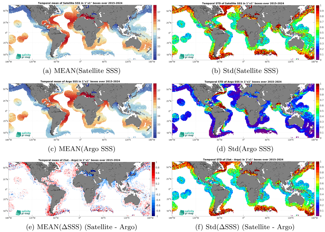
Figure 7: Temporal mean (left) and Std (right) of SSS from SMAP SSS L2 v6 (RSS) (top), Argo (middle), and of \Delta SSS (Satellite - Argo). Only match-up pairs are used to generate these maps.
