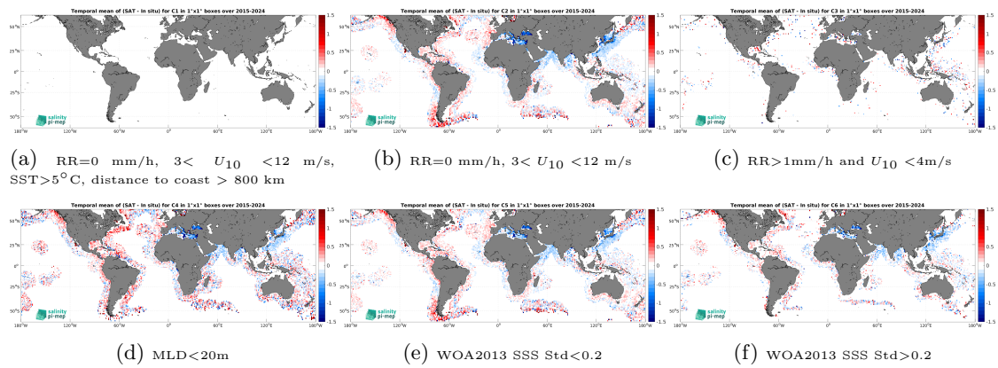
Figure 14: Temporal mean gridded over spatial boxes of size 1^\circ \times 1^\circ of \Delta SSS (SMAP SSS L2 v6 (RSS) - Argo) for 6 different subdatasets corresponding to:RR=0 mm/h, 3 < U_{10} < 12 m/s, SST > 5^\circ C, distance to coast > 800 km (a), RR=0 mm/h, 3 < U_{10} < 12 m/s (b), RR > 1 mm/h and U_{10} < 4 m/s (c),MLD < 20 m (d),WOA2013 SSS Std < 0.2 (e),WOA2013 SSS Std > 0.2 (f).
