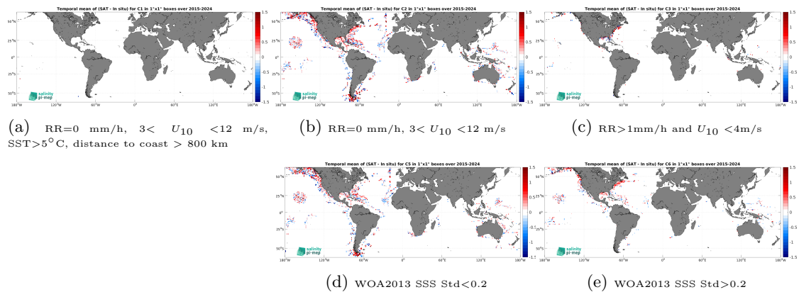
Figure 14: Temporal mean gridded over spatial boxes of size 1^\circ \times 1^\circ of \Delta\text{SSS} (SMAP SSS L2 v6 - 40 km (RSS) - TSG (SAMOS)) for 5 different subdatasets corresponding to: RR=0 mm/h, 3 < U_{10} < 12 m/s, SST > 5°C, distance to coast > 800 km (a), RR=0 mm/h, 3 < U_{10} < 12 m/s (b), RR > 1mm/h and U_{10} < 4 m/s (c), WOA2013 SSS Std < 0.2 (d), WOA2013 SSS Std > 0.2 (e).
