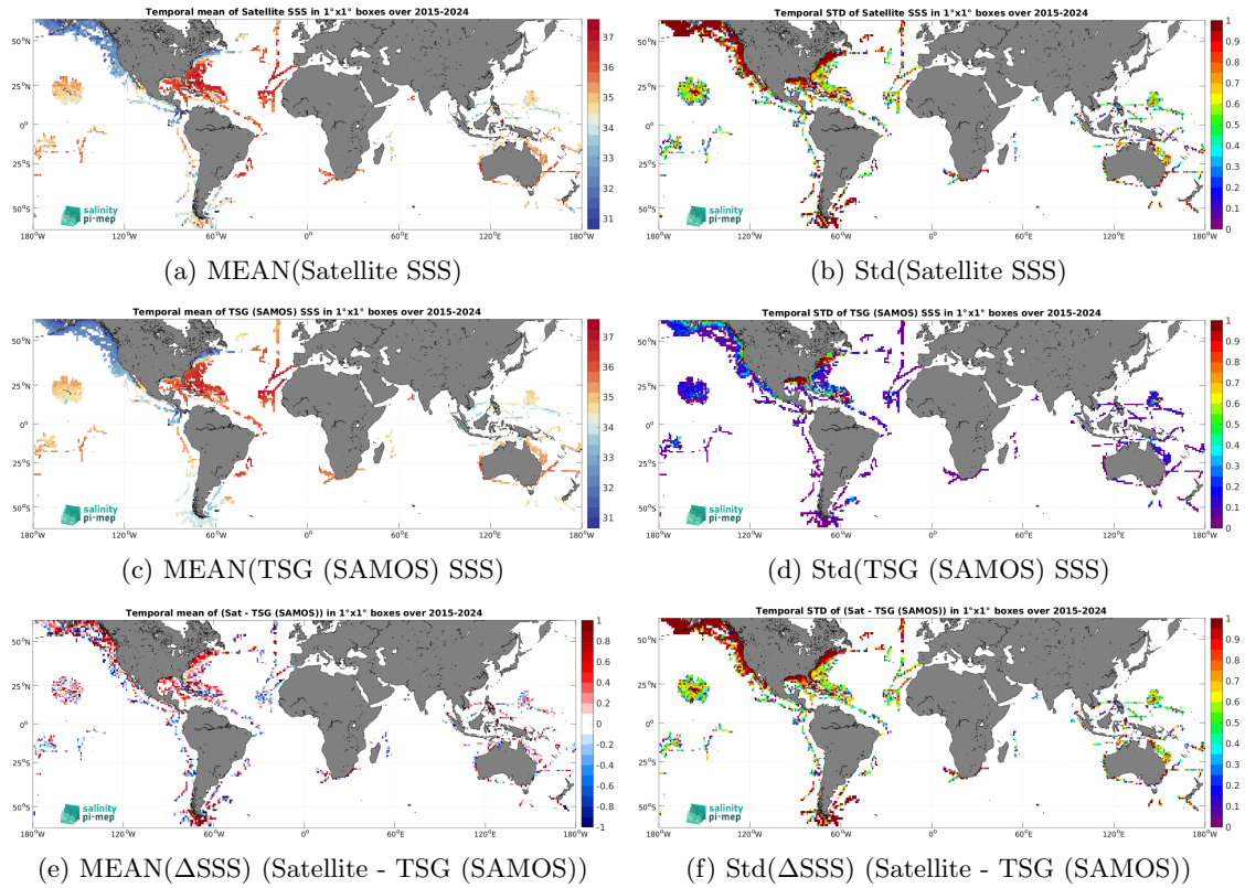
Figure 7: Temporal mean (left) and Std (right) of SSS from SMAP SSS L2 v6 - 40 km (RSS) (top), TSG (SAMOS) (middle), and of \Delta SSS (Satellite - TSG (SAMOS)). Only match-up pairs are used to generate these maps.
