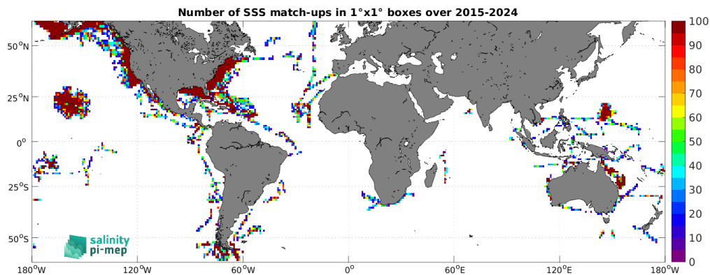
Figure 5: Number of SSS match-ups between TSG (SAMOS) SSS and the SMAP SSS L2 v6 - 40 km (RSS) SSS product for the SMOS coastal zone (<800km) 60N-60S Pi-MEP region over 1^\circ \times 1^\circ boxes and for the full satellite product period.
