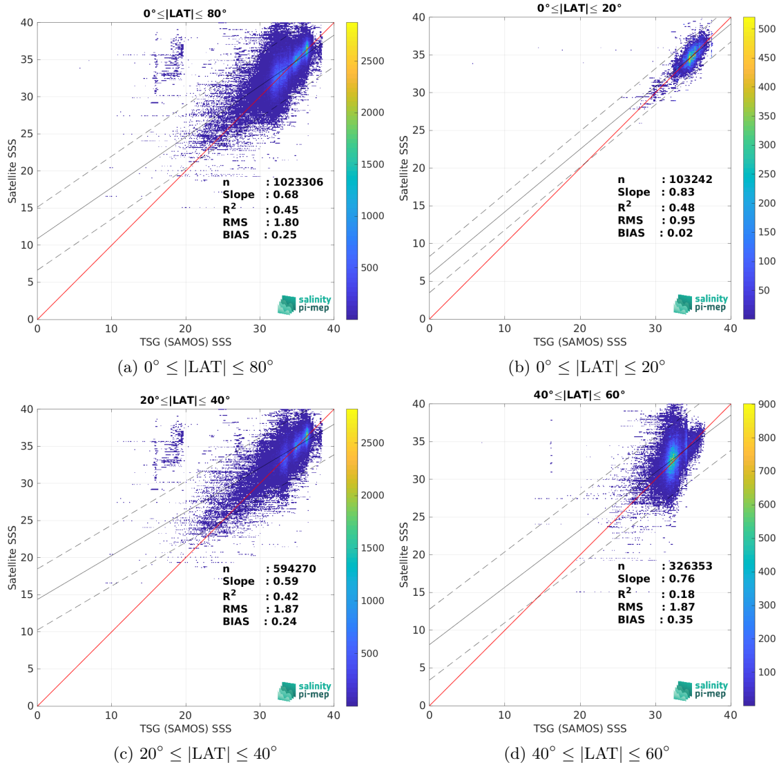
Figure 10: Contour maps of the concentration of SMAP SSS L2 v6 - 40 km (RSS) SSS (y-axis) versus TSG (SAMOS) SSS (x-axis) at match-up pairs for different latitude bands. For each plot, the red line shows x=y . The black thin and dashed lines indicate a linear fit through the data cloud and the \pm 95\% confidence levels, respectively. The number match-up pairs n , the slope and R^2 coefficient of the linear fit, the root mean square (RMS) and the mean bias between satellite and in situ data are indicated for each latitude band in each plots.
