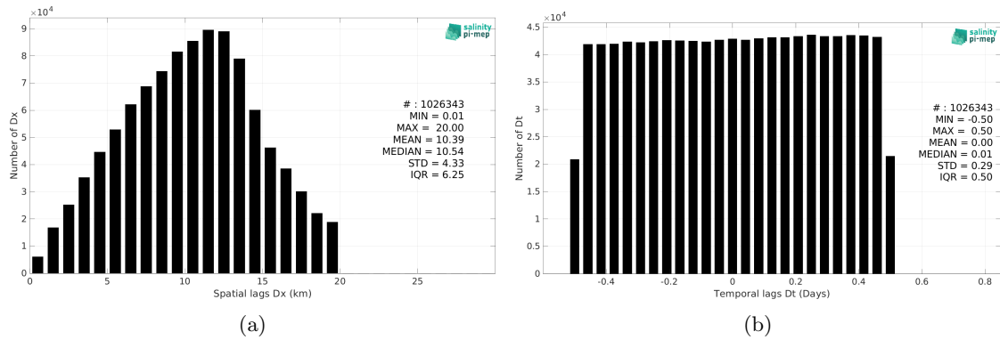
Figure 6: Histograms of the spatial (a) and temporal (b) lags between the location/time of the TSG (SAMOS) measurement and the date of the corresponding SMAP SSS L2 v6 - 40 km (RSS) SSS pixel.
