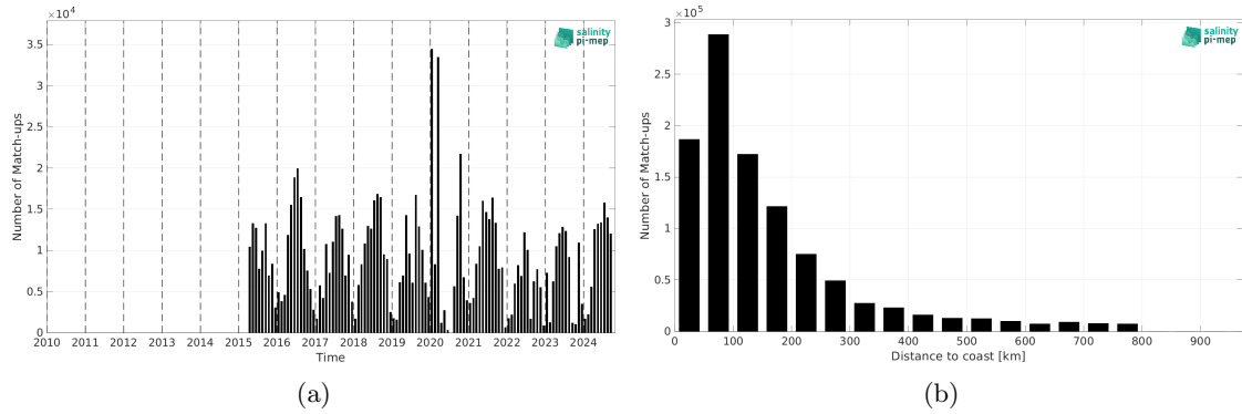
Figure 2: Number of match-ups between TSG (SAMOS) and SMAP SSS L2 v6 - 40 km (RSS) SSS as a function of time (a) and as function of the distance to coast (b) over the SMOS coastal zone (<800km) 60N-60S Pi-MEP region and for the full satellite product period.
