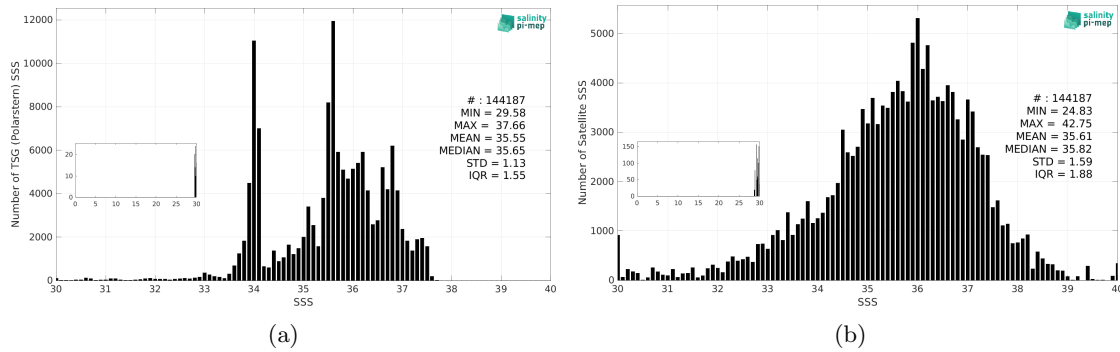
Figure 3: Histograms of SSS from TSG (Polarstern) (a) and SMAP SSS L2 v6 - 40 km (RSS) (b) considering all match-up pairs per bins of 0.1 over the SMOS coastal zone (<800km) 60N-60S Pi-MEP region and for the full satellite product period.
