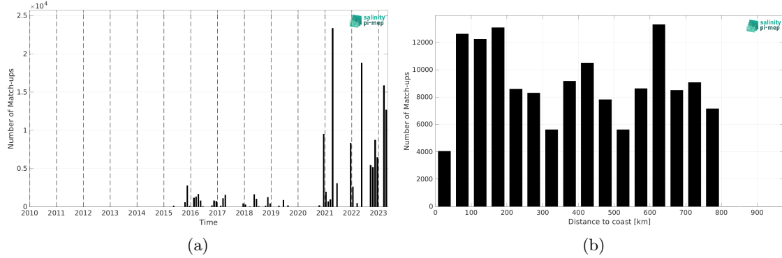
Figure 2: Number of match-ups between TSG (Polarstern) and SMAP SSS L2 v6 - 40 km (RSS) SSS as a function of time (a) and as function of the distance to coast (b) over the SMOS coastal zone (<800km) 60N-60S Pi-MEP region and for the full satellite product period.
