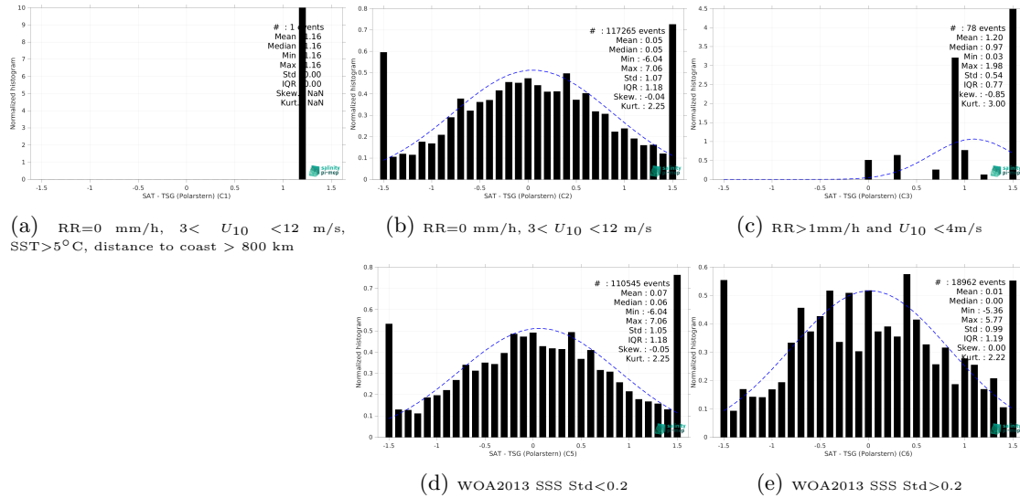
Figure 15: Normalized histogram of \Delta SSS (SMAP SSS L2 v6 - 40 km (RSS) - TSG (Polarstern)) for 5 different subdatasets corresponding to: RR=0 mm/h, 3 < U_{10} < 12 m/s, SST > 5^\circ C , distance to coast > 800 km (a), RR=0 mm/h, 3 < U_{10} < 12 m/s (b), RR > 1 mm/h and U_{10} < 4 m/s (c), WOA2013 SSS Std < 0.2 (d), WOA2013 SSS Std > 0.2 (e).
