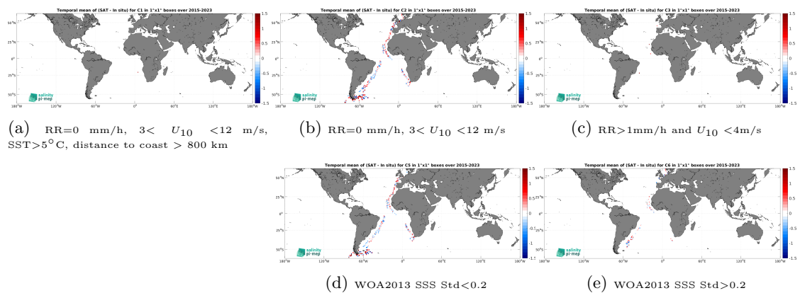
Figure 14: Temporal mean gridded over spatial boxes of size 1^\circ \times 1^\circ of \Delta\text{SSS} (SMAP SSS L2 v6 - 40 km (RSS) - TSG (Polarstern)) for 5 different subdatasets corresponding to:RR=0 mm/h, 3 < U_{10} < 12 m/s, SST >5^\circ\text{C} , distance to coast > 800 km (a), RR=0 mm/h, 3 < U_{10} < 12 m/s (b), RR >1 mm/h and U_{10} < 4 m/s (c), WOA2013 SSS Std <0.2 (d), WOA2013 SSS Std >0.2 (e).
