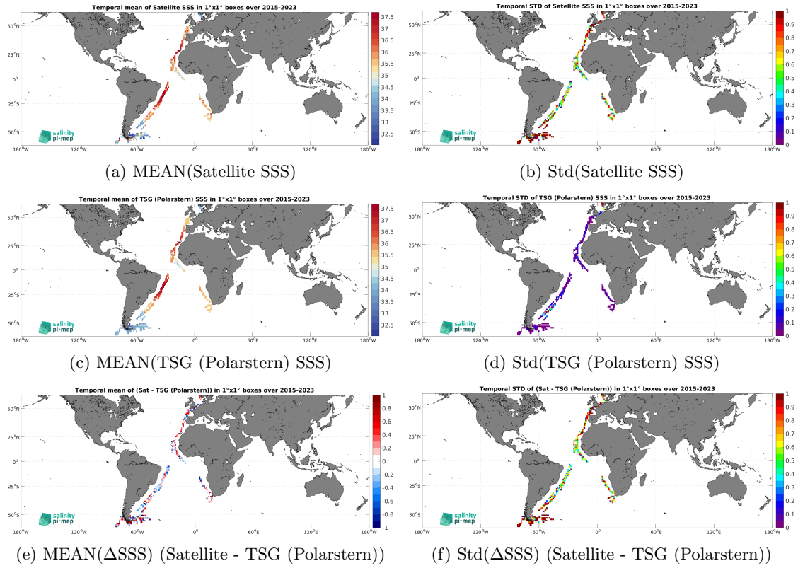
Figure 7: Temporal mean (left) and Std (right) of SSS from SMAP SSS L2 v6 - 40 km (RSS) (top), TSG (Polarstern) (middle), and of \Delta SSS (Satellite - TSG (Polarstern)). Only match-up pairs are used to generate these maps.
