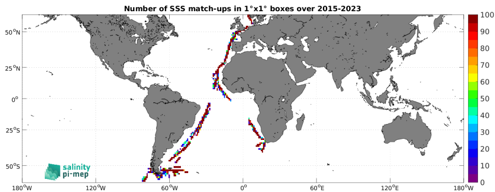
Figure 5: Number of SSS match-ups between TSG (Polarstern) SSS and the SMAP SSS L2 v6 - 40 km (RSS) SSS product for the SMOS coastal zone (<800km) 60N-60S Pi-MEP region over 1^\circ \times 1^\circ boxes and for the full satellite product period.
