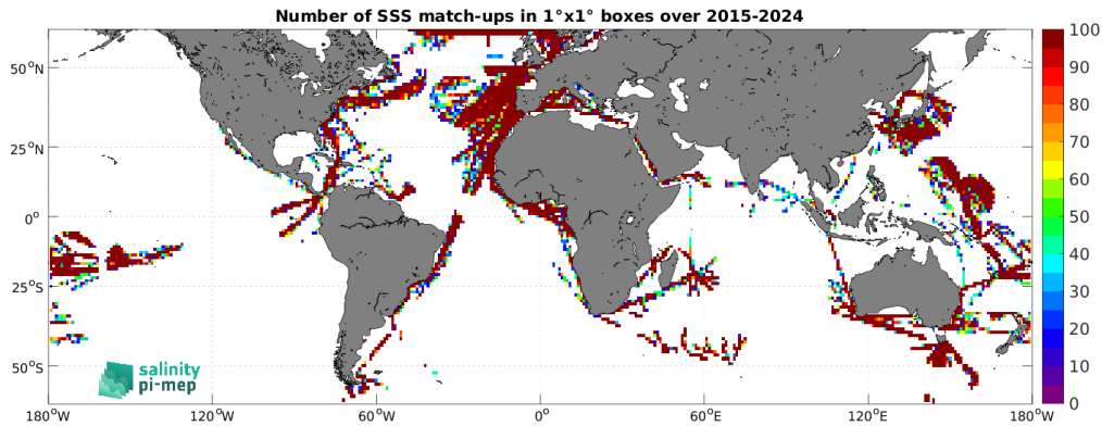
Figure 5: Number of SSS match-ups between TSG (LEGOS-DM) SSS and the SMAP SSS L2 v6 - 40 km (RSS) SSS product for the SMOS coastal zone (<800km) 60N-60S Pi-MEP region over 1^\circ \times 1^\circ boxes and for the full satellite product period.
