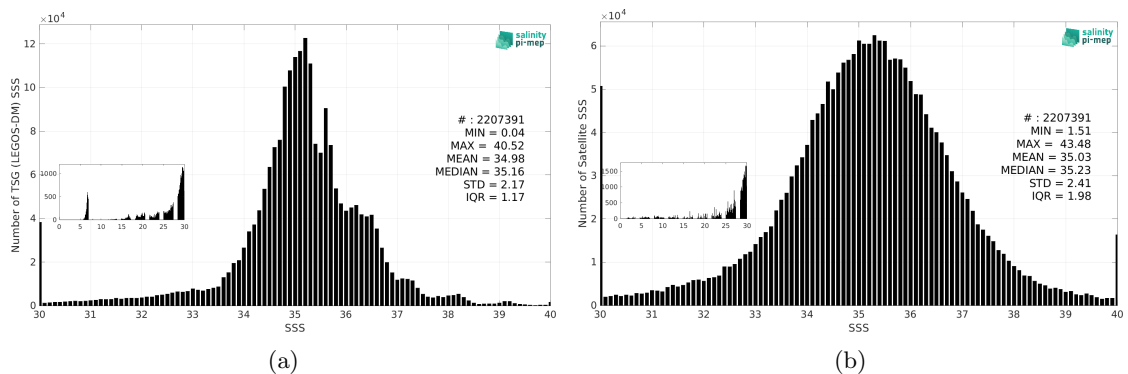
Figure 3: Histograms of SSS from TSG (LEGOS-DM) (a) and SMAP SSS L2 v6 - 40 km (RSS) (b) considering all match-up pairs per bins of 0.1 over the SMOS coastal zone (<800km) 60N-60S Pi-MEP region and for the full satellite product period.
