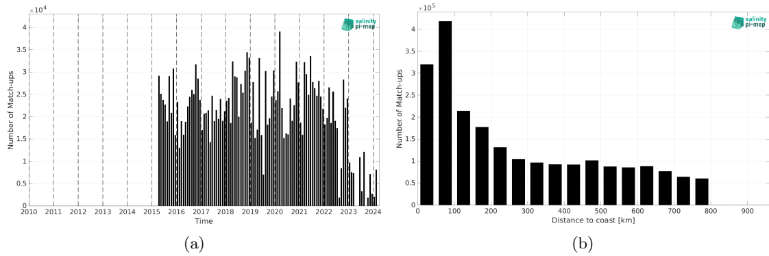
Figure 2: Number of match-ups between TSG (LEGOS-DM) and SMAP SSS L2 v6 - 40 km (RSS) SSS as a function of time (a) and as function of the distance to coast (b) over the SMOS coastal zone (<800km) 60N-60S Pi-MEP region and for the full satellite product period.
