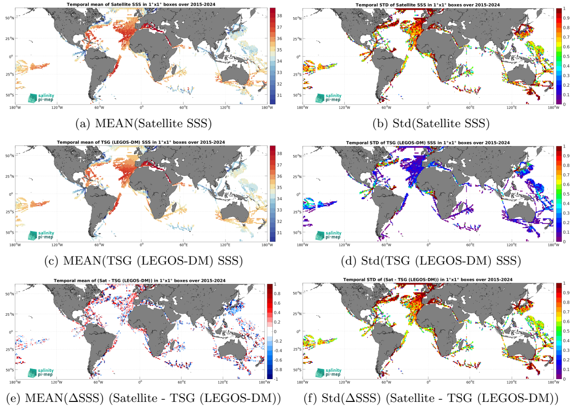
Figure 7: Temporal mean (left) and Std (right) of SSS from SMAP SSS L2 v6 - 40 km (RSS) (top), TSG (LEGOS-DM) (middle), and of \Delta SSS (Satellite - TSG (LEGOS-DM)). Only match-up pairs are used to generate these maps.
