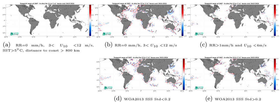
Figure 14: Temporal mean gridded over spatial boxes of size 1^\circ \times 1^\circ of \Delta\text{SSS} (SMAP SSS L2 v6 - 40 km (RSS) - TSG (LEGOS-DM)) for 5 different subdatasets corresponding to:RR=0 mm/h, 3 < U_{10} < 12 m/s, SST >5^\circ\text{C} , distance to coast > 800 km (a), RR=0 mm/h, 3 < U_{10} < 12 m/s (b), RR >1 mm/h and U_{10} < 4 m/s (c), WOA2013 SSS Std <0.2 (d), WOA2013 SSS Std >0.2 (e).
