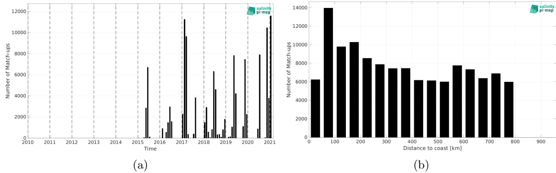
Figure 2: Number of match-ups between TSG (GOSUD-Sailing-ship) and SMAP SSS L2 v6 - 40 km (RSS) SSS as a function of time (a) and as function of the distance to coast (b) over the SMOS coastal zone (<800km) 60N-60S Pi-MEP region and for the full satellite product period.
