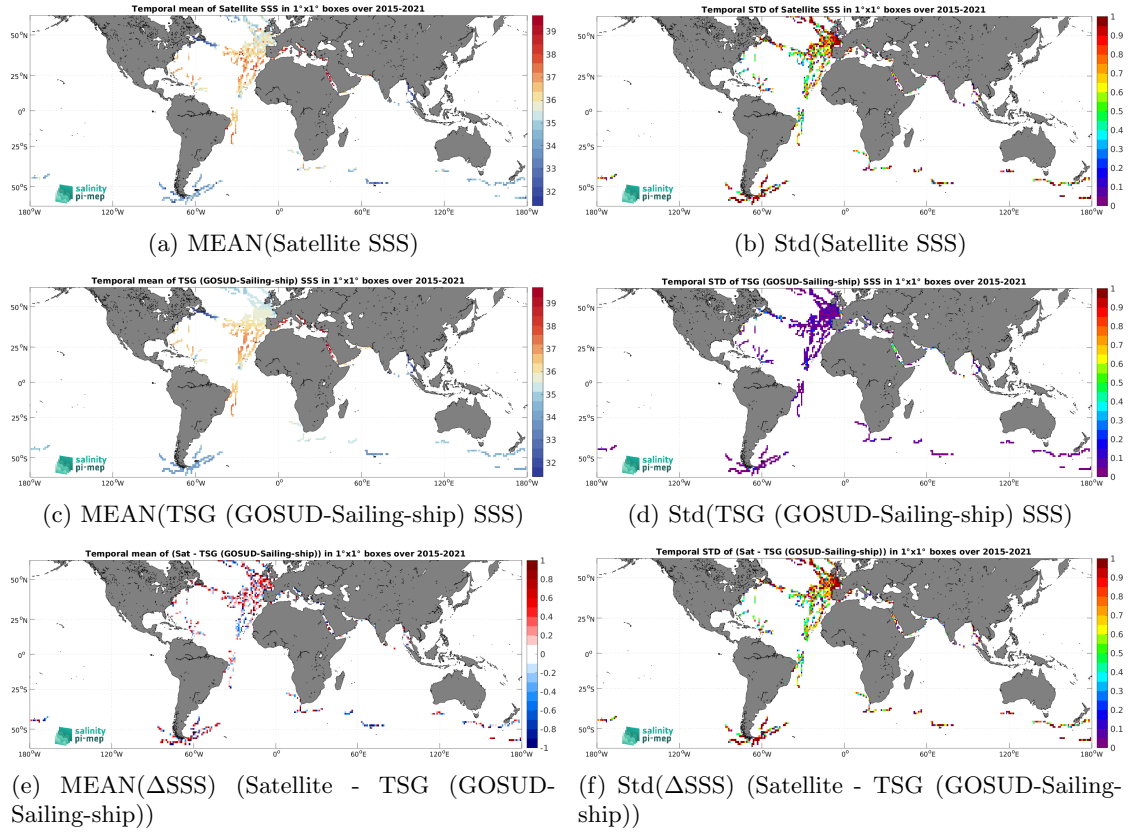
Figure 7: Temporal mean (left) and Std (right) of SSS from SMAP SSS L2 v6 - 40 km (RSS) (top), TSG (GOSUD-Sailing-ship) (middle), and of \Delta SSS (Satellite - TSG (GOSUD-Sailing-ship)). Only match-up pairs are used to generate these maps.
