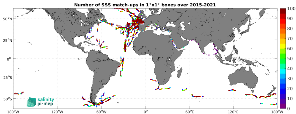
Figure 5: Number of SSS match-ups between TSG (GOSUD-Sailing-ship) SSS and the SMAP SSS L2 v6 - 40 km (RSS) SSS product for the SMOS coastal zone ( <800\text{km} ) 60N-60S Pi-MEP region over 1^\circ \times 1^\circ boxes and for the full satellite product period.
