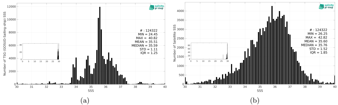
Figure 3: Histograms of SSS from TSG (GOSUD-Sailing-ship) (a) and SMAP SSS L2 v6 - 40 km (RSS) (b) considering all match-up pairs per bins of 0.1 over the SMOS coastal zone (<800km) 60N-60S Pi-MEP region and for the full satellite product period.
