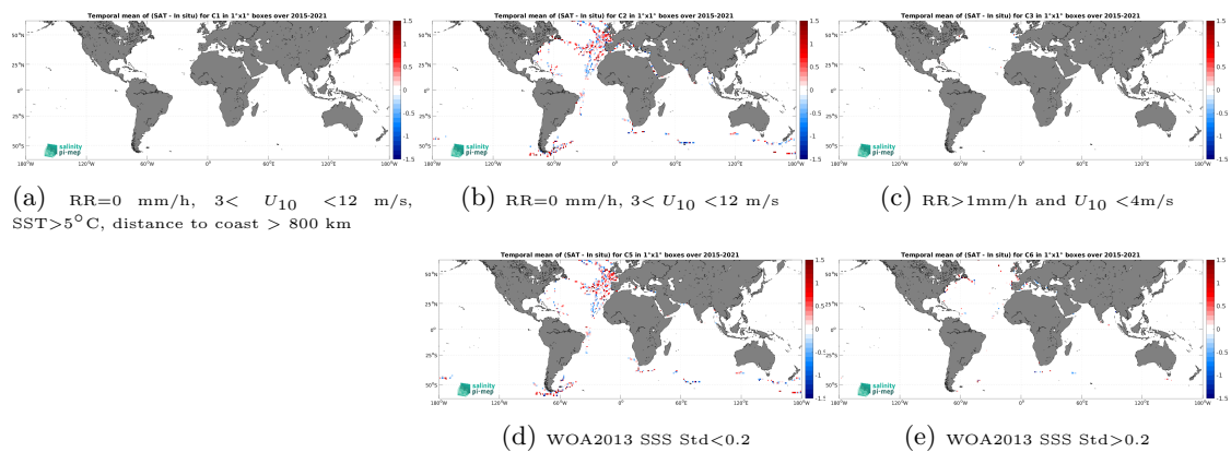
Figure 14: Temporal mean gridded over spatial boxes of size 1^\circ \times 1^\circ of \Delta\text{SSS} (SMAP SSS L2 v6 - 40 km (RSS) - TSG (GOSUD-Sailing-ship)) for 5 different subdatasets corresponding to: RR=0 mm/h, 3 < U_{10} < 12 m/s, SST > 5°C, distance to coast > 800 km (a), RR=0 mm/h, 3 < U_{10} < 12 m/s (b), RR > 1mm/h and U_{10} < 4 m/s (c), WOA2013 SSS Std < 0.2 (d), WOA2013 SSS Std > 0.2 (e).
