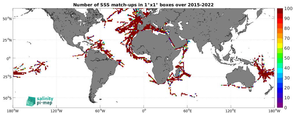
Figure 5: Number of SSS match-ups between TSG (GOSUD-Research-vessel) SSS and the SMAP SSS L2 v6 - 40 km (RSS) SSS product for the SMOS coastal zone (<800km) 60N-60S Pi-MEP region over 1^\circ \times 1^\circ boxes and for the full satellite product period.
