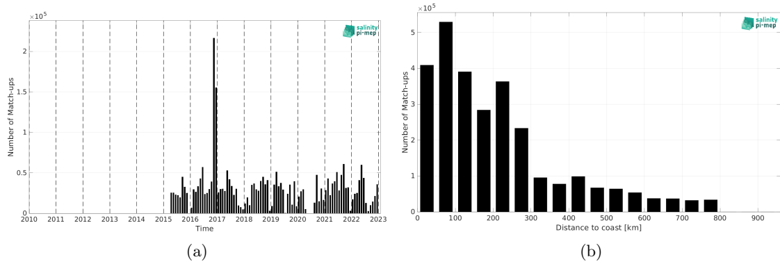
Figure 2: Number of match-ups between TSG (GOSUD-Research-vessel) and SMAP SSS L2 v6 - 40 km (RSS) SSS as a function of time (a) and as function of the distance to coast (b) over the SMOS coastal zone (<800km) 60N-60S Pi-MEP region and for the full satellite product period.
