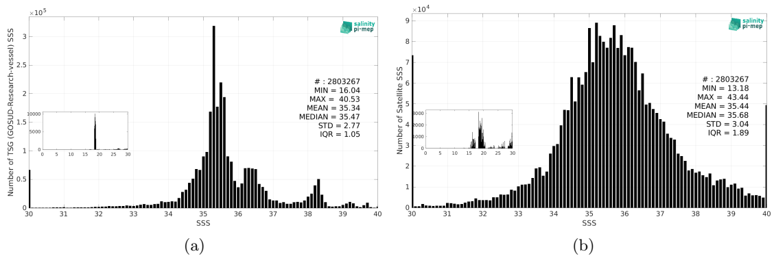
Figure 3: Histograms of SSS from TSG (GOSUD-Research-vessel) (a) and SMAP SSS L2 v6 - 40 km (RSS) (b) considering all match-up pairs per bins of 0.1 over the SMOS coastal zone (<800km) 60N-60S Pi-MEP region and for the full satellite product period.
