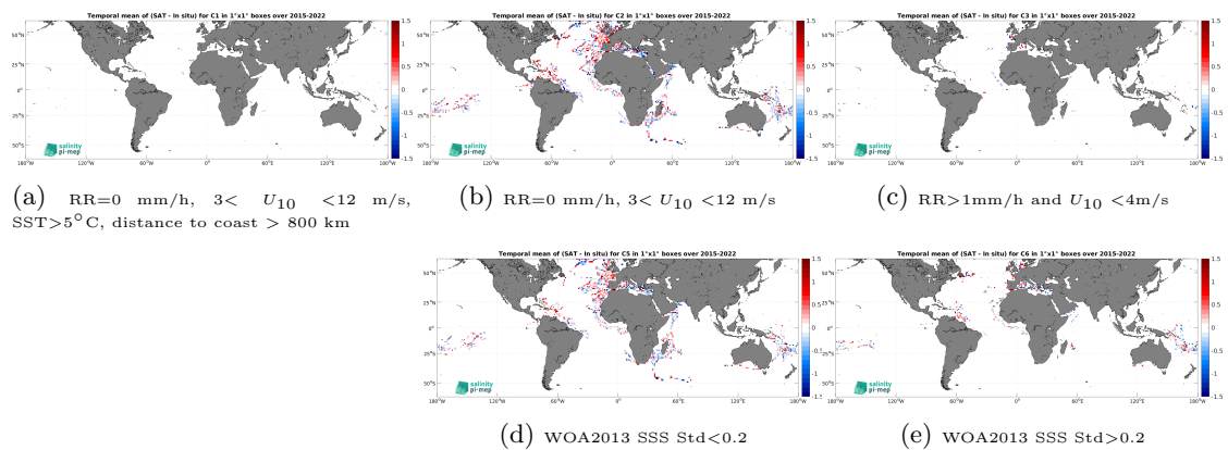
Figure 14: Temporal mean gridded over spatial boxes of size 1^\circ \times 1^\circ of \Delta SSS (SMAP SSS L2 v6 - 40 km (RSS) - TSG (GOSUD-Research-vessel)) for 5 different subdatasets corresponding to:RR=0 mm/h, 3 < U_{10} < 12 m/s, SST > 5^\circ\text{C} , distance to coast > 800 km (a), RR=0 mm/h, 3 < U_{10} < 12 m/s (b), RR > 1 mm/h and U_{10} < 4 m/s (c), WOA2013 SSS Std < 0.2 (d), WOA2013 SSS Std > 0.2 (e).
