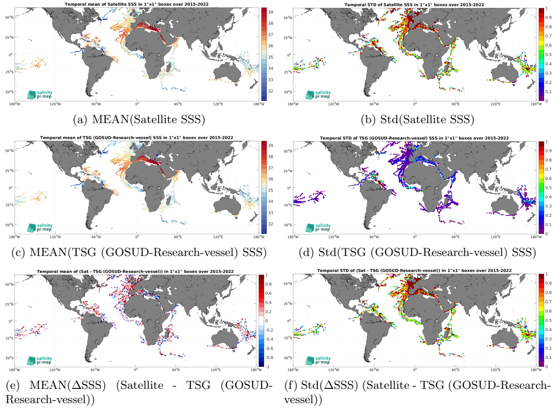
Figure 7: Temporal mean (left) and Std (right) of SSS from SMAP SSS L2 v6 - 40 km (RSS) (top), TSG (GOSUD-Research-vessel) (middle), and of \Delta SSS (Satellite - TSG (GOSUD-Research-vessel)). Only match-up pairs are used to generate these maps.
