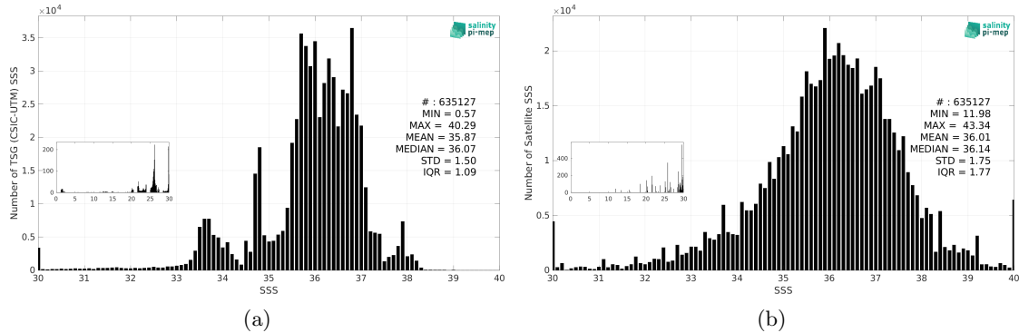
Figure 3: Histograms of SSS from TSG (CSIC-UTM) (a) and SMAP SSS L2 v6 - 40 km (RSS) (b) considering all match-up pairs per bins of 0.1 over the SMOS coastal zone (<800km) 60N-60S Pi-MEP region and for the full satellite product period.
