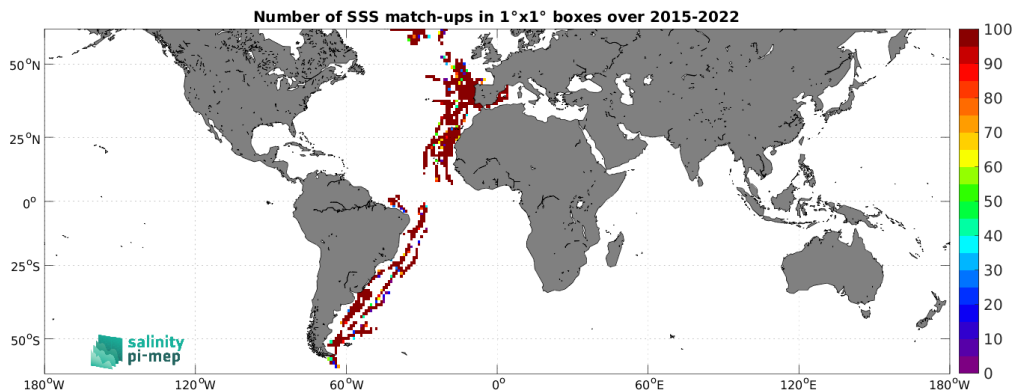
Figure 5: Number of SSS match-ups between TSG (CSIC-UTM) SSS and the SMAP SSS L2 v6 - 40 km (RSS) SSS product for the SMOS coastal zone (<800km) 60N-60S Pi-MEP region over 1^\circ \times 1^\circ boxes and for the full satellite product period.
