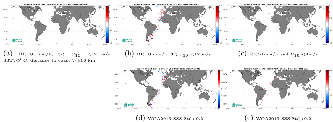
Figure 14: Temporal mean gridded over spatial boxes of size 1^\circ \times 1^\circ of \Delta\text{SSS} (SMAP SSS L2 v6 - 40 km (RSS) - TSG (CSIC-UTM)) for 5 different subdatasets corresponding to:RR=0 mm/h, 3 < U_{10} < 12 m/s, SST>5°C, distance to coast > 800 km (a), RR=0 mm/h, 3 < U_{10} < 12 m/s (b), RR>1mm/h and U_{10} < 4 m/s (c), WOA2013 SSS Std<0.2 (d), WOA2013 SSS Std>0.2 (e).
