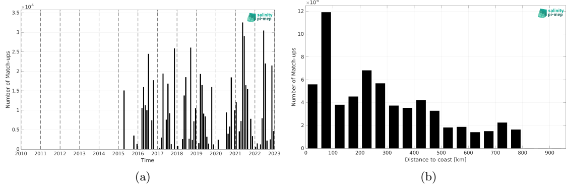
Figure 2: Number of match-ups between TSG (CSIC-UTM) and SMAP SSS L2 v6 - 40 km (RSS) SSS as a function of time (a) and as function of the distance to coast (b) over the SMOS coastal zone (<800km) 60N-60S Pi-MEP region and for the full satellite product period.
