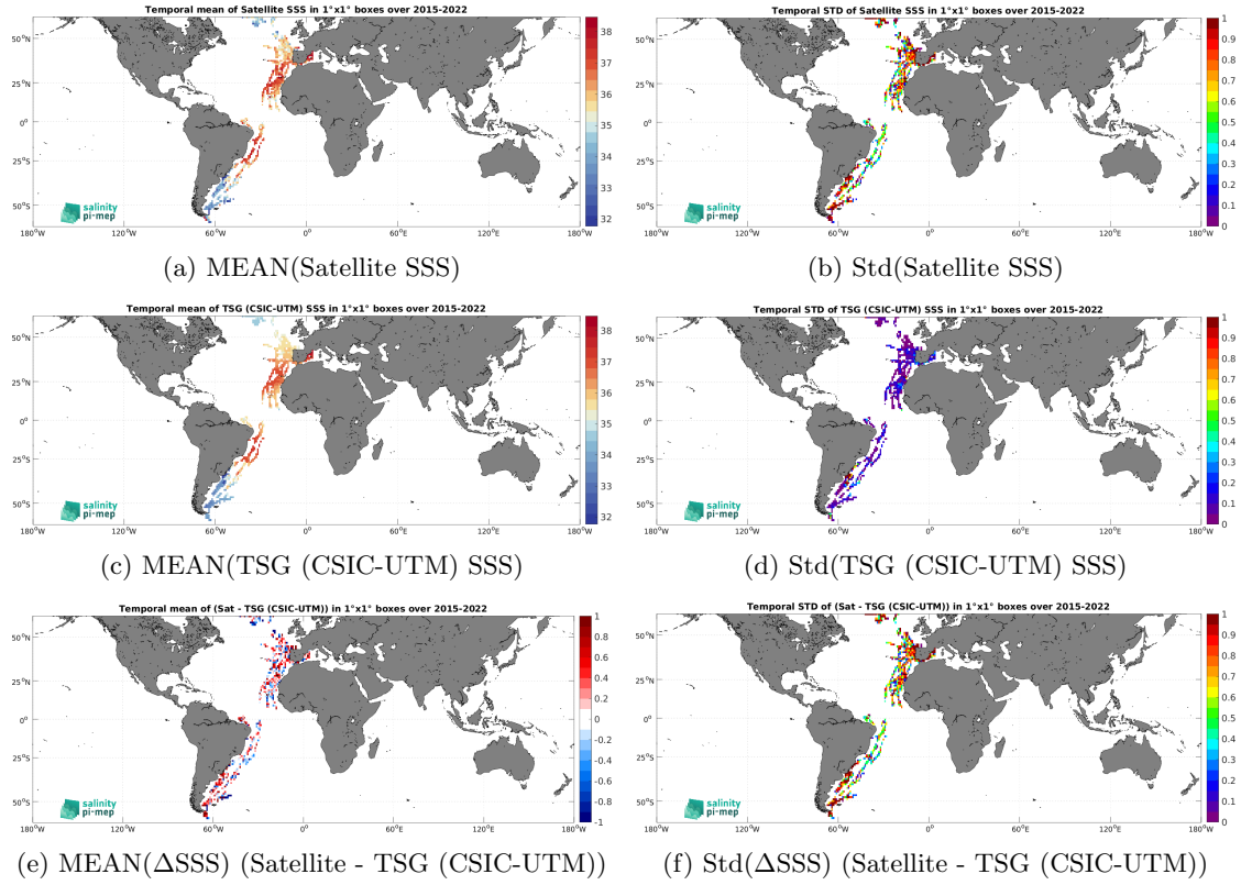
Figure 7: Temporal mean (left) and Std (right) of SSS from SMAP SSS L2 v6 - 40 km (RSS) (top), TSG (CSIC-UTM) (middle), and of \Delta SSS (Satellite - TSG (CSIC-UTM)). Only match-up pairs are used to generate these maps.
