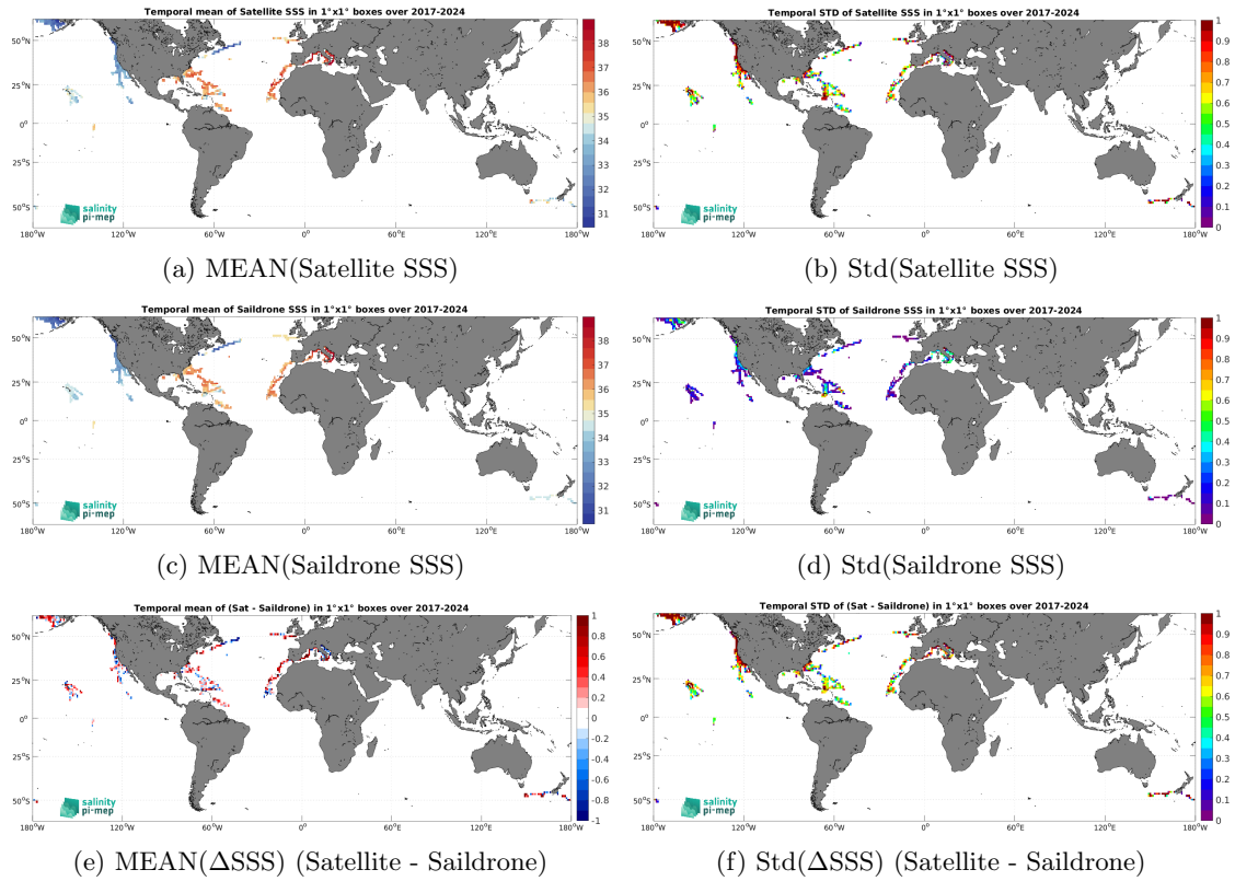
Figure 7: Temporal mean (left) and Std (right) of SSS from SMAP SSS L2 v6 - 40 km (RSS) (top), Saildrone (middle), and of \Delta SSS (Satellite - Saildrone). Only match-up pairs are used to generate these maps.
