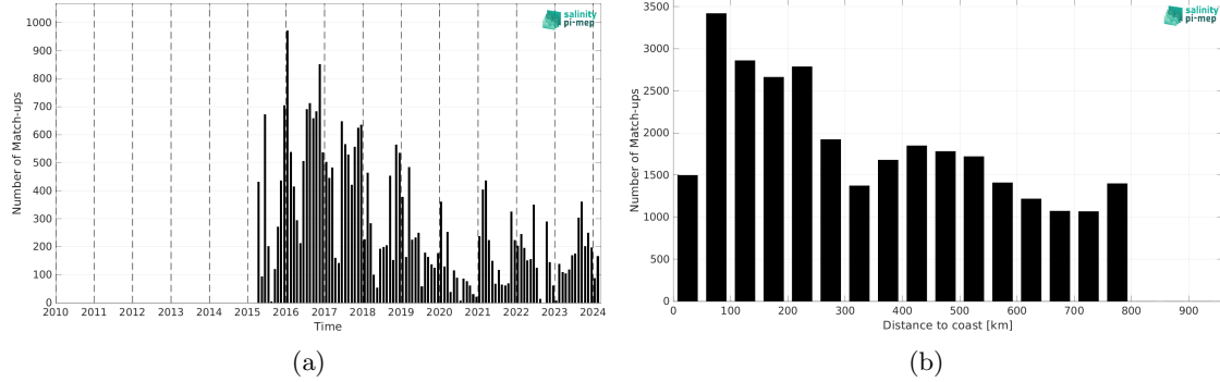
Figure 2: Number of match-ups between Marine mammals and SMAP SSS L2 v6 - 40 km (RSS) SSS as a function of time (a) and as function of the distance to coast (b) over the SMOS coastal zone (<800km) 60N-60S Pi-MEP region and for the full satellite product period.
