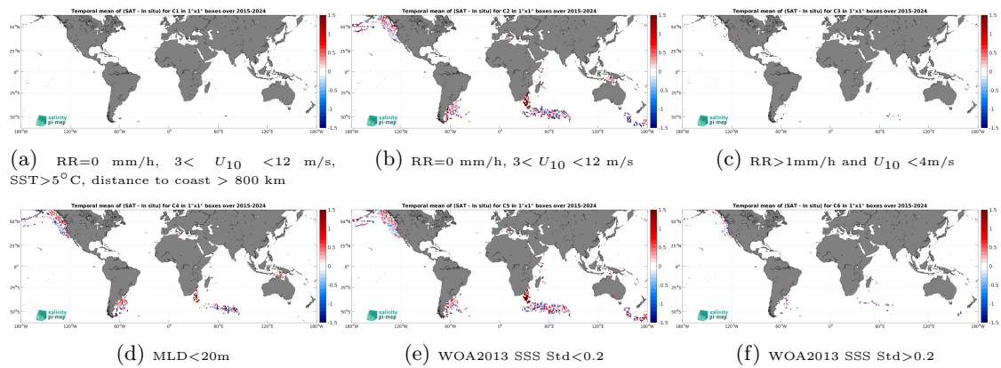
Figure 14: Temporal mean gridded over spatial boxes of size 1^\circ \times 1^\circ of \Delta\text{SSS} (SMAP SSS L2 v6 - 40 km (RSS) - Marine mammals) for 6 different subdatasets corresponding to: RR=0 mm/h, 3 < U_{10} < 12 m/s, SST > 5°C, distance to coast > 800 km (a), RR=0 mm/h, 3 < U_{10} < 12 m/s (b), RR > 1mm/h and U_{10} < 4 m/s (c), MLD < 20m (d), WOA2013 SSS Std < 0.2 (e), WOA2013 SSS Std > 0.2 (f).
