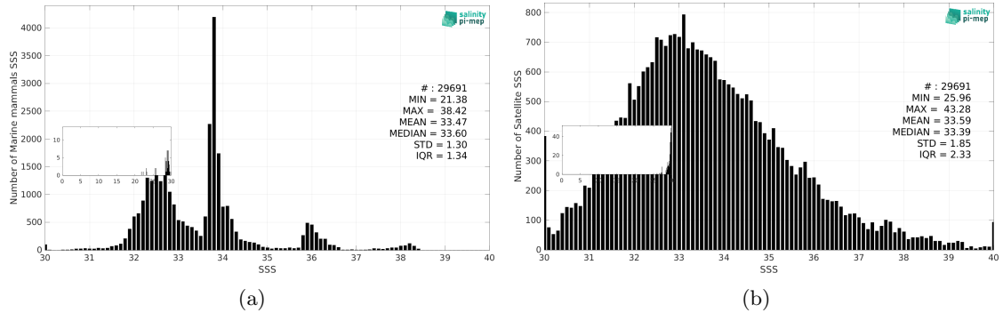
Figure 3: Histograms of SSS from Marine mammals (a) and SMAP SSS L2 v6 - 40 km (RSS) (b) considering all match-up pairs per bins of 0.1 over the SMOS coastal zone (<800km) 60N-60S Pi-MEP region and for the full satellite product period.
