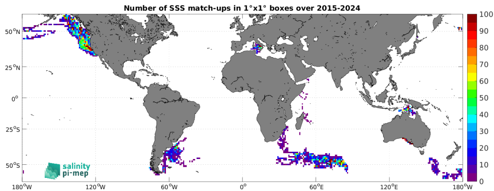
Figure 5: Number of SSS match-ups between Marine mammals SSS and the SMAP SSS L2 v6 - 40 km (RSS) SSS product for the SMOS coastal zone (<800km) 60N-60S Pi-MEP region over 1^\circ \times 1^\circ boxes and for the full satellite product period.
