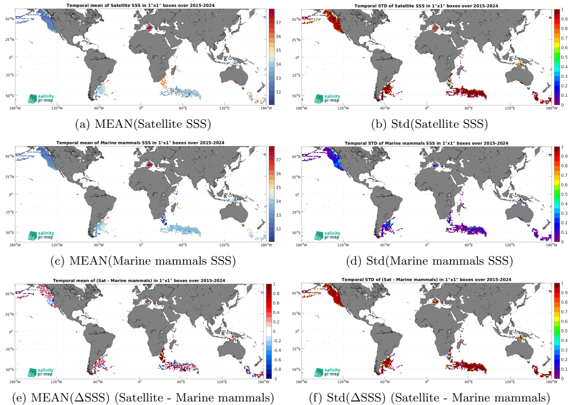
Figure 7: Temporal mean (left) and Std (right) of SSS from SMAP SSS L2 v6 - 40 km (RSS) (top), Marine mammals (middle), and of \Delta SSS (Satellite - Marine mammals). Only match-up pairs are used to generate these maps.
