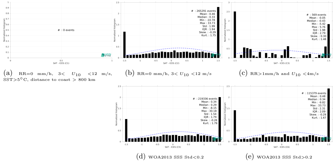
Figure 15: Normalized histogram of \Delta SSS (SMAP SSS L2 v6 - 40 km (RSS) - ICES) for 5 different subdatasets corresponding to: RR=0 mm/h, 3 < U_{10} < 12 m/s, SST > 5°C, distance to coast > 800 km (a), RR=0 mm/h, 3 < U_{10} < 12 m/s (b), RR > 1mm/h and U_{10} < 4 m/s (c), WOA2013 SSS Std < 0.2 (d), WOA2013 SSS Std > 0.2 (e).
