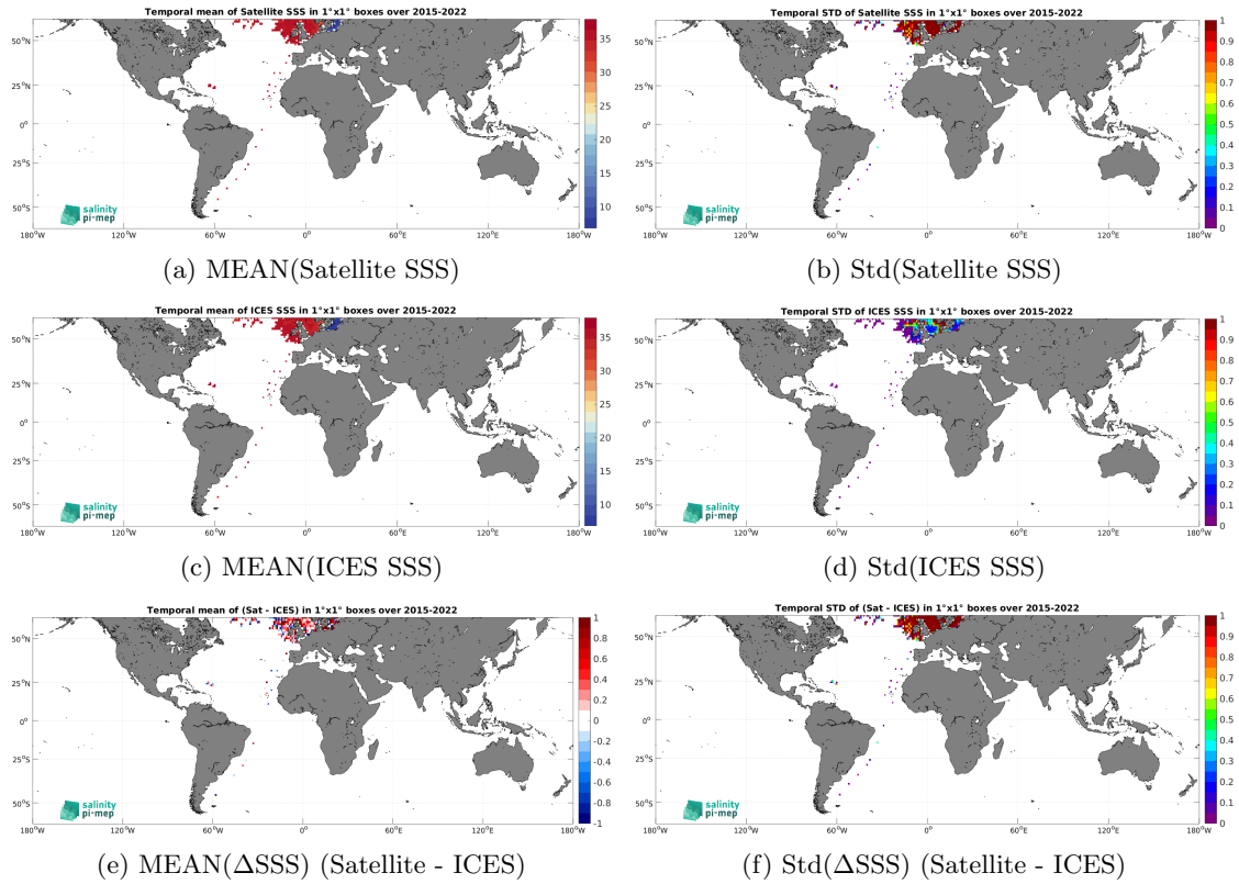
Figure 7: Temporal mean (left) and Std (right) of SSS from SMAP SSS L2 v6 - 40 km (RSS) (top), ICES (middle), and of \Delta SSS (Satellite - ICES). Only match-up pairs are used to generate these maps.
