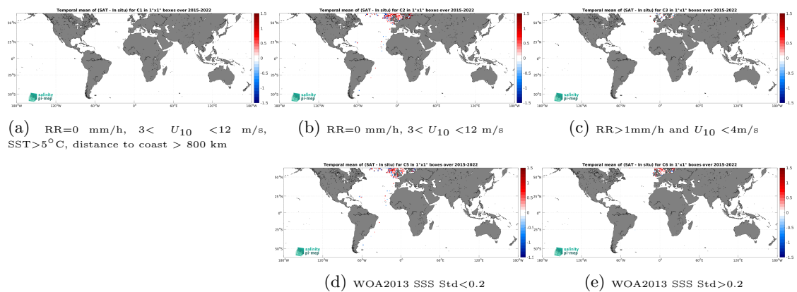
Figure 14: Temporal mean gridded over spatial boxes of size 1^\circ \times 1^\circ of \Delta SSS (SMAP SSS L2 v6 - 40 km (RSS) - ICES) for 5 different subdatasets corresponding to:RR=0 mm/h, 3 < U_{10} < 12 m/s, SST >5^\circ C, distance to coast > 800 km (a), RR=0 mm/h, 3 < U_{10} < 12 m/s (b), RR >1 mm/h and U_{10} < 4 m/s (c), WOA2013 SSS Std <0.2 (d), WOA2013 SSS Std >0.2 (e).
