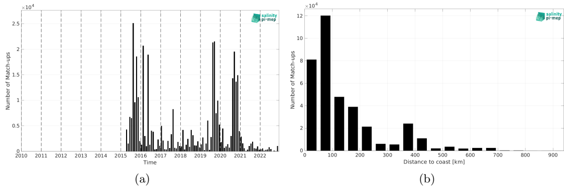
Figure 2: Number of match-ups between ICES and SMAP SSS L2 v6 - 40 km (RSS) SSS as a function of time (a) and as function of the distance to coast (b) over the SMOS coastal zone (<800km) 60N-60S Pi-MEP region and for the full satellite product period.
