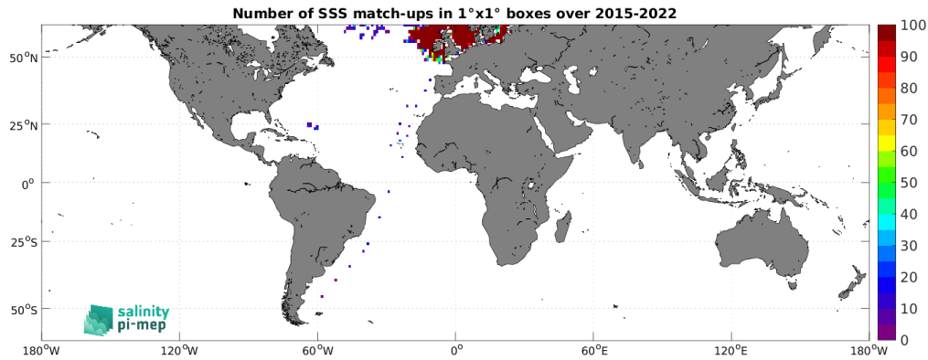
Figure 5: Number of SSS match-ups between ICES SSS and the SMAP SSS L2 v6 - 40 km (RSS) SSS product for the SMOS coastal zone (<800km) 60N-60S Pi-MEP region over 1^\circ \times 1^\circ boxes and for the full satellite product period.
