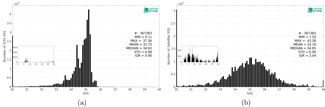
Figure 3: Histograms of SSS from ICES (a) and SMAP SSS L2 v6 - 40 km (RSS) (b) considering all match-up pairs per bins of 0.1 over the SMOS coastal zone (<800km) 60N-60S Pi-MEP region and for the full satellite product period.
