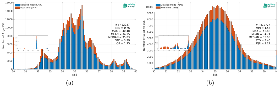
Figure 3: Histograms of SSS from Argo (a) and SMAP SSS L2 v6 - 40 km (RSS) (b) considering all match-up pairs per bins of 0.1 over the SMOS coastal zone (<800km) 60N-60S Pi-MEP region and for the full satellite product period.
