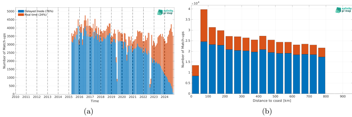
Figure 2: Number of match-ups between Argo and SMAP SSS L2 v6 - 40 km (RSS) SSS as a function of time (a) and as function of the distance to coast (b) over the SMOS coastal zone (<800km) 60N-60S Pi-MEP region and for the full satellite product period.
