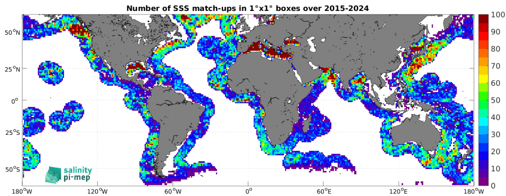
Figure 5: Number of SSS match-ups between Argo SSS and the SMAP SSS L2 v6 - 40 km (RSS) SSS product for the SMOS coastal zone (<800km) 60N-60S Pi-MEP region over 1^\circ \times 1^\circ boxes and for the full satellite product period.
