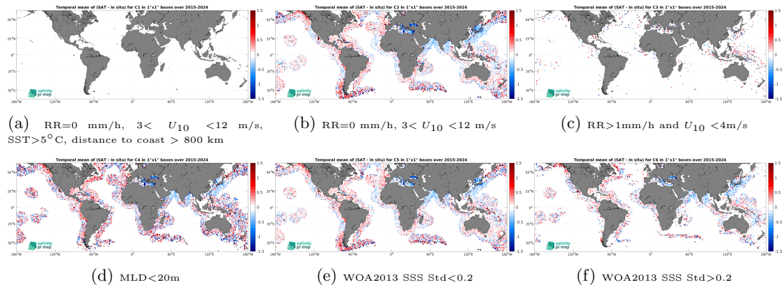
Figure 14: Temporal mean gridded over spatial boxes of size 1^\circ \times 1^\circ of \Delta SSS (SMAP SSS L2 v6 - 40 km (RSS) - Argo) for 6 different subdatasets corresponding to:RR=0 mm/h, 3 < U_{10} < 12 m/s, SST > 5^\circ\text{C} , distance to coast > 800 km (a), RR=0 mm/h, 3 < U_{10} < 12 m/s (b), RR > 1 mm/h and U_{10} < 4 m/s (c),MLD < 20 m (d),WOA2013 SSS Std < 0.2 (e),WOA2013 SSS Std > 0.2 (f).
