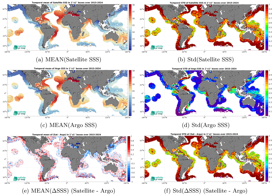
Figure 7: Temporal mean (left) and Std (right) of SSS from SMAP SSS L2 v6 - 40 km (RSS) (top), Argo (middle), and of \Delta SSS (Satellite - Argo). Only match-up pairs are used to generate these maps.
