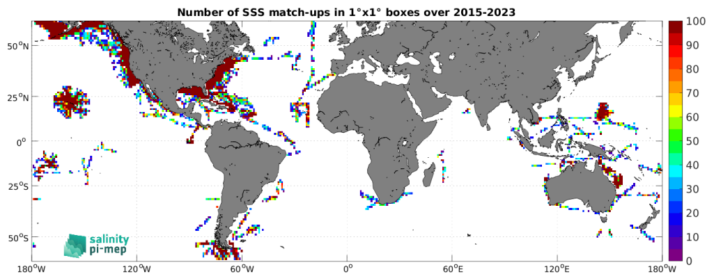
Figure 4: Number of SSS match-ups between TSG (SAMOS) SSS and the SMAP SSS L2 v5 (RSS) SSS product for the SMOS coastal zone ( <800\text{km} ) 60\text{N} - 60\text{S} Pi-MEP region over 1^\circ \times 1^\circ boxes and for the full satellite product period.
