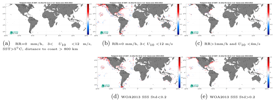
Figure 12: Temporal mean gridded over spatial boxes of size 1^\circ \times 1^\circ of \Delta\text{SSS} (SMAP SSS L2 v5 (RSS) - TSG (SAMOS)) for 5 different subdatasets corresponding to:RR=0 mm/h, 3 < U_{10} < 12 m/s, SST >5^\circ\text{C} , distance to coast > 800 km (a), RR=0 mm/h, 3 < U_{10} < 12 m/s (b), RR >1 mm/h and U_{10} < 4 m/s (c), WOA2013 SSS Std <0.2 (d), WOA2013 SSS Std >0.2 (e).
