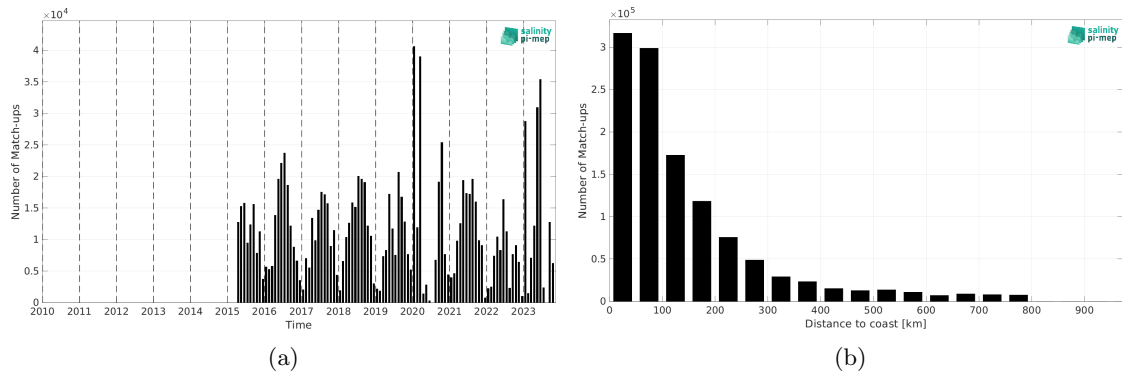
Figure 1: Number of match-ups between TSG (SAMOS) and SMAP SSS L2 v5 (RSS) SSS as a function of time (a) and as function of the distance to coast (b) over the SMOS coastal zone (<800km) 60N-60S Pi-MEP region and for the full satellite product period.
