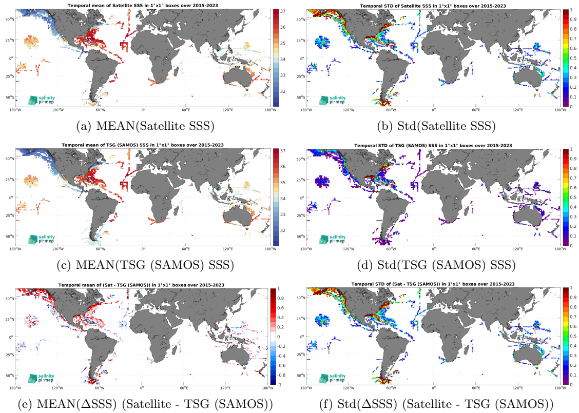
Figure 6: Temporal mean (left) and Std (right) of SSS from SMAP SSS L2 v5 (RSS) (top), TSG (SAMOS) (middle), and of \Delta SSS (Satellite - TSG (SAMOS)). Only match-up pairs are used to generate these maps.
