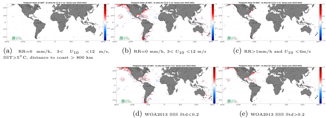
Figure 12: Temporal mean gridded over spatial boxes of size 1^\circ \times 1^\circ of \Delta SSS (SMAP SSS L2 v5 (RSS) - TSG (SAMOS)) for 5 different subdatasets corresponding to:RR=0 mm/h, 3 < U_{10} < 12 m/s, SST >5^\circ\text{C} , distance to coast > 800 km (a), RR=0 mm/h, 3 < U_{10} < 12 m/s (b), RR >1 mm/h and U_{10} < 4 m/s (c), WOA2013 SSS Std <0.2 (d), WOA2013 SSS Std >0.2 (e).
