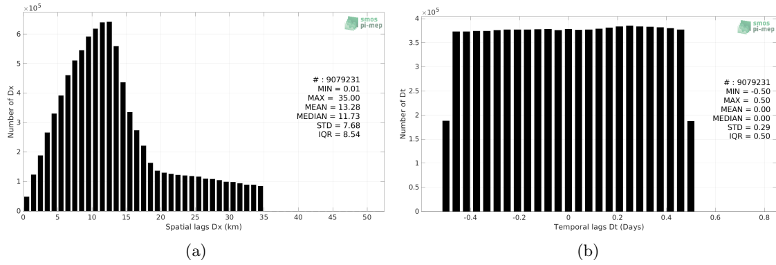
Figure 5: Histograms of the spatial (a) and temporal (b) lags between the location/time of the TSG (SAMOS) measurement and the date of the corresponding SMAP SSS L2 v5 (RSS) SSS pixel.
