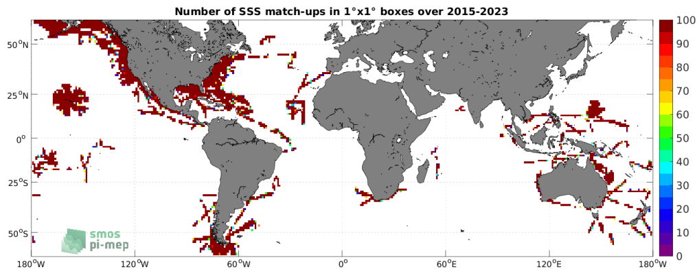
Figure 4: Number of SSS match-ups between TSG (SAMOS) SSS and the SMAP SSS L2 v5 (RSS) SSS product for the SMOS coastal zone (<800km) 60N-60S Pi-MEP region over 1^\circ \times 1^\circ boxes and for the full satellite product period.
