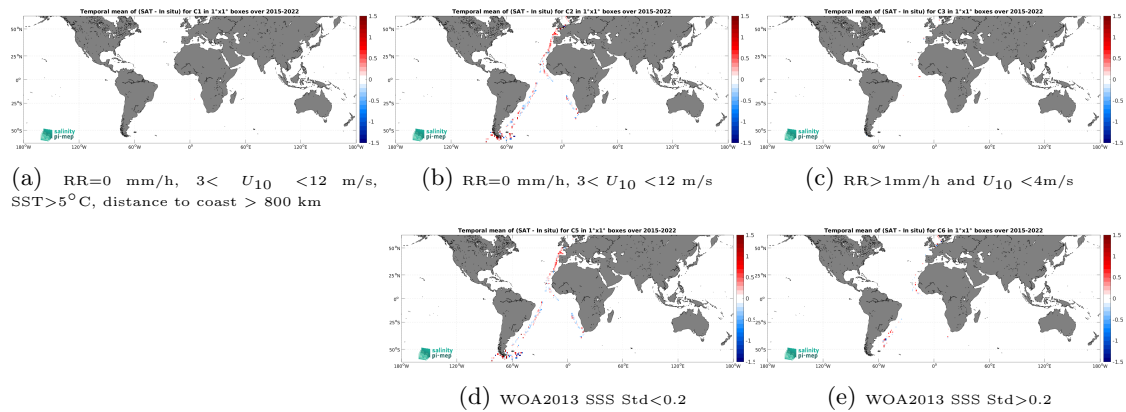
Figure 12: Temporal mean gridded over spatial boxes of size 1^\circ \times 1^\circ of \Delta\text{SSS} (SMAP SSS L2 v5 (RSS) - TSG (Polarstern)) for 5 different subdatasets corresponding to:RR=0 mm/h, 3 < U_{10} < 12 m/s, SST >5^\circ\text{C} , distance to coast > 800 km (a), RR=0 mm/h, 3 < U_{10} < 12 m/s (b), RR >1 mm/h and U_{10} < 4 m/s (c), WOA2013 SSS Std <0.2 (d), WOA2013 SSS Std >0.2 (e).
