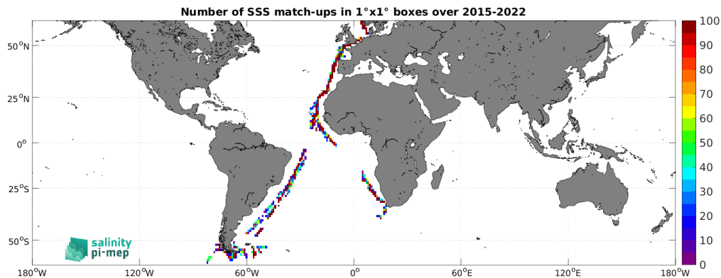
Figure 4: Number of SSS match-ups between TSG (Polarstern) SSS and the SMAP SSS L2 v5 (RSS) SSS product for the SMOS coastal zone (<800km) 60N-60S Pi-MEP region over 1^\circ \times 1^\circ boxes and for the full satellite product period.
