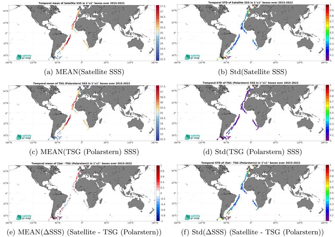
Figure 6: Temporal mean (left) and Std (right) of SSS from SMAP SSS L2 v5 (RSS) (top), TSG (Polarstern) (middle), and of \Delta SSS (Satellite - TSG (Polarstern)). Only match-up pairs are used to generate these maps.
