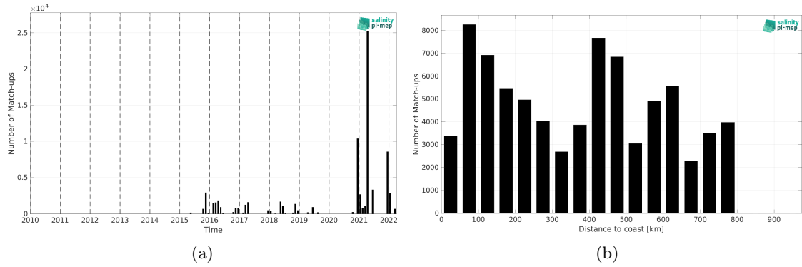
Figure 1: Number of match-ups between TSG (Polarstern) and SMAP SSS L2 v5 (RSS) SSS as a function of time (a) and as function of the distance to coast (b) over the SMOS coastal zone (<800km) 60N-60S Pi-MEP region and for the full satellite product period.
