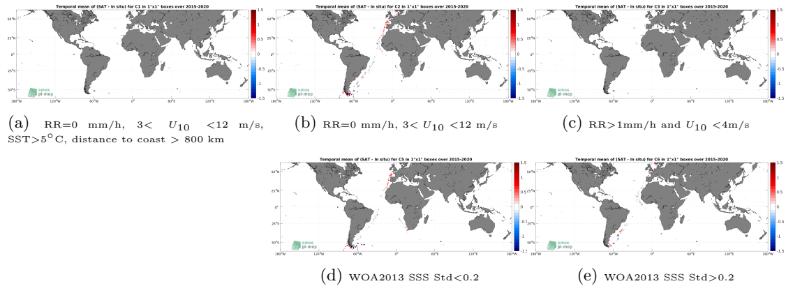
Figure 12: Temporal mean gridded over spatial boxes of size 1^\circ \times 1^\circ of \Delta SSS (SMAP SSS L2 v5 (RSS) - TSG (Polarstern)) for 5 different subdatasets corresponding to:RR=0 mm/h, 3 < U_{10} < 12 m/s, SST >5^\circ\text{C} , distance to coast > 800 km (a), RR=0 mm/h, 3 < U_{10} < 12 m/s (b), RR >1 mm/h and U_{10} < 4 m/s (c), WOA2013 SSS Std <0.2 (d), WOA2013 SSS Std >0.2 (e).
