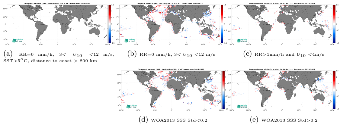
Figure 12: Temporal mean gridded over spatial boxes of size 1^\circ \times 1^\circ of \Delta SSS (SMAP SSS L2 v5 (RSS) - TSG (LEGOS-DM)) for 5 different subdatasets corresponding to:RR=0 mm/h, 3 < U_{10} < 12 m/s, SST >5^\circ\text{C} , distance to coast > 800 km (a), RR=0 mm/h, 3 < U_{10} < 12 m/s (b), RR >1 mm/h and U_{10} < 4 m/s (c), WOA2013 SSS Std <0.2 (d), WOA2013 SSS Std >0.2 (e).
