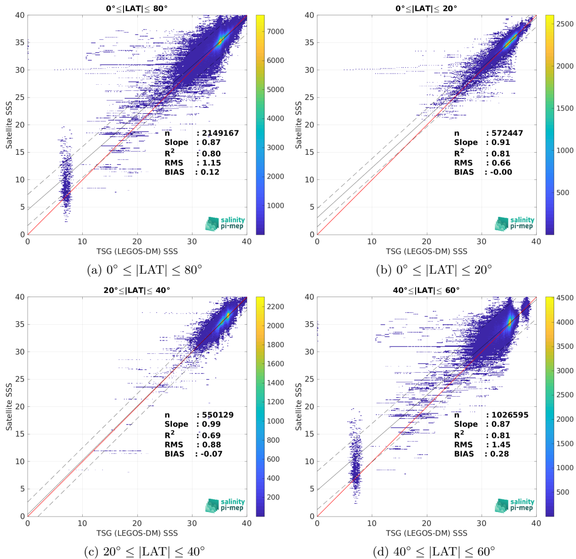
Figure 9: Contour maps of the concentration of SMAP SSS L2 v5 (RSS) SSS (y-axis) versus TSG (LEGOS-DM) SSS (x-axis) at match-up pairs for different latitude bands. For each plot, the red line shows x=y . The black thin and dashed lines indicate a linear fit through the data cloud and the \pm 95\% confidence levels, respectively. The number match-up pairs n , the slope and R^2 coefficient of the linear fit, the root mean square (RMS) and the mean bias between satellite and in situ data are indicated for each latitude band in each plots.
