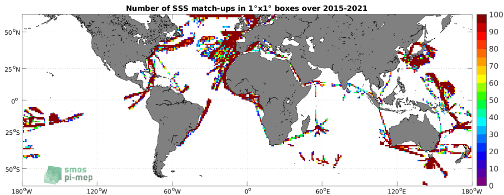
Figure 4: Number of SSS match-ups between TSG (LEGOS-DM) SSS and the SMAP SSS L2 v5 (RSS) SSS product for the SMOS coastal zone (<800km) 60N-60S Pi-MEP region over 1°x1° boxes and for the full satellite product period.
