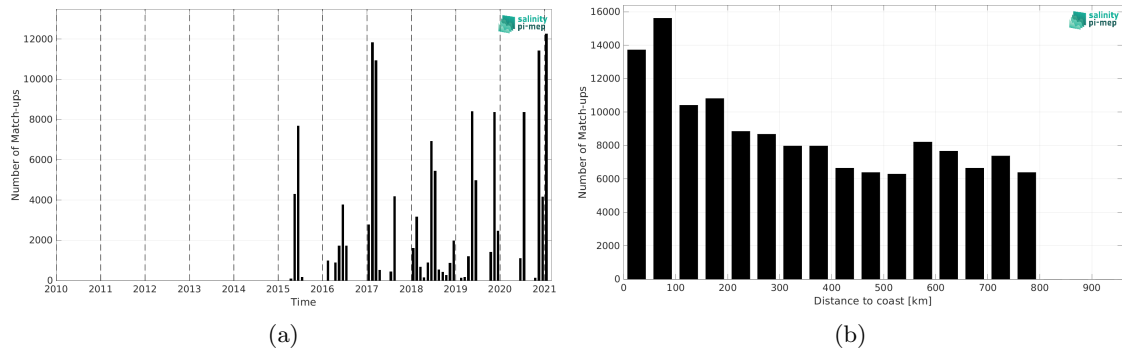
Figure 1: Number of match-ups between TSG (GOSUD-Sailing-ship) and SMAP SSS L2 v5 (RSS) SSS as a function of time (a) and as function of the distance to coast (b) over the SMOS coastal zone (<800km) 60N-60S Pi-MEP region and for the full satellite product period.
