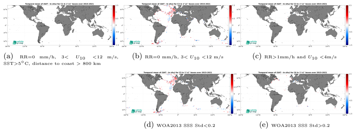
Figure 12: Temporal mean gridded over spatial boxes of size 1^\circ \times 1^\circ of \Delta SSS (SMAP SSS L2 v5 (RSS) - TSG (GOSUD-Sailing-ship)) for 5 different subdatasets corresponding to:RR=0 mm/h, 3 < U_{10} < 12 m/s, SST >5^\circ\text{C} , distance to coast > 800 km (a), RR=0 mm/h, 3 < U_{10} < 12 m/s (b), RR >1 mm/h and U_{10} < 4 m/s (c), WOA2013 SSS Std <0.2 (d), WOA2013 SSS Std >0.2 (e).
