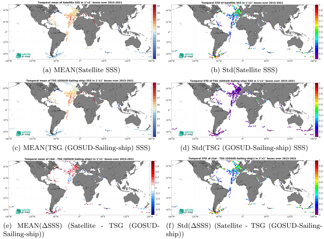
Figure 6: Temporal mean (left) and Std (right) of SSS from SMAP SSS L2 v5 (RSS) (top), TSG (GOSUD-Sailing-ship) (middle), and of \Delta SSS (Satellite - TSG (GOSUD-Sailing-ship)). Only match-up pairs are used to generate these maps.
