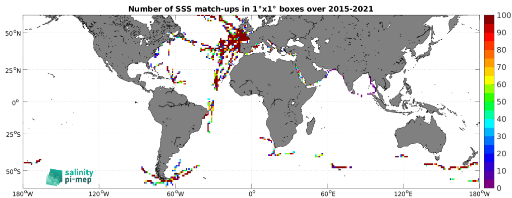
Figure 4: Number of SSS match-ups between TSG (GOSUD-Sailing-ship) SSS and the SMAP SSS L2 v5 (RSS) SSS product for the SMOS coastal zone ( <800\text{km} ) 60N-60S Pi-MEP region over 1^\circ \times 1^\circ boxes and for the full satellite product period.
