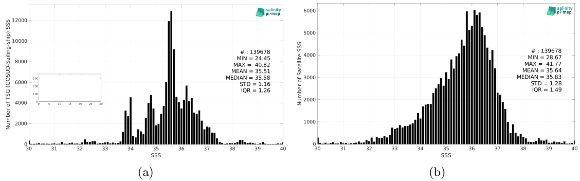
Figure 2: Histograms of SSS from TSG (GOSUD-Sailing-ship) (a) and SMAP SSS L2 v5 (RSS) (b) considering all match-up pairs per bins of 0.1 over the SMOS coastal zone (<800km) 60N-60S Pi-MEP region and for the full satellite product period.
