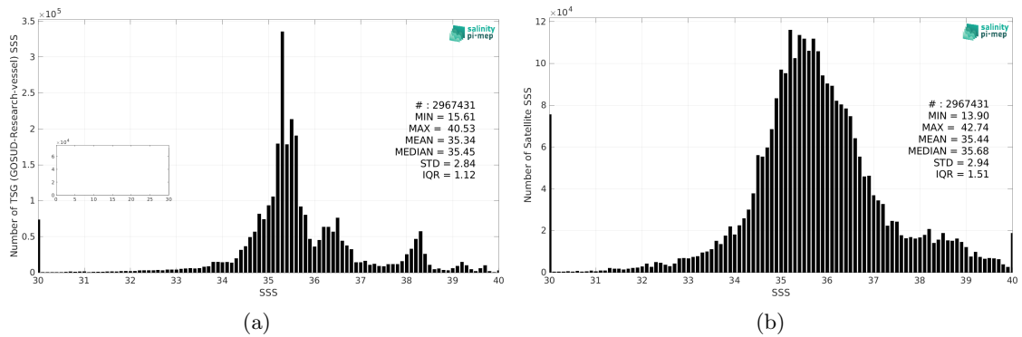
Figure 2: Histograms of SSS from TSG (GOSUD-Research-vessel) (a) and SMAP SSS L2 v5 (RSS) (b) considering all match-up pairs per bins of 0.1 over the SMOS coastal zone (<800km) 60N-60S Pi-MEP region and for the full satellite product period.
