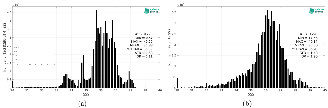
Figure 2: Histograms of SSS from TSG (CSIC-UTM) (a) and SMAP SSS L2 v5 (RSS) (b) considering all match-up pairs per bins of 0.1 over the SMOS coastal zone (<800km) 60N-60S Pi-MEP region and for the full satellite product period.
