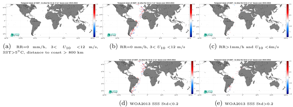
Figure 12: Temporal mean gridded over spatial boxes of size 1^\circ \times 1^\circ of \Delta\text{SSS} (SMAP SSS L2 v5 (RSS) - TSG (CSIC-UTM)) for 5 different subdatasets corresponding to:RR=0 mm/h, 3 < U_{10} < 12 m/s, SST >5^\circ\text{C} , distance to coast > 800 km (a), RR=0 mm/h, 3 < U_{10} < 12 m/s (b), RR >1 mm/h and U_{10} < 4 m/s (c), WOA2013 SSS Std <0.2 (d), WOA2013 SSS Std >0.2 (e).
