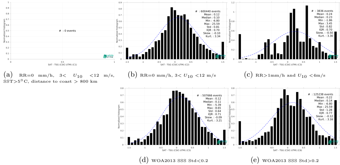
Figure 13: Normalized histogram of \Delta SSS (SMAP SSS L2 v5 (RSS) - TSG (CSIC-UTM)) for 5 different subdatasets corresponding to: RR=0 mm/h, 3 < U_{10} < 12 m/s, SST > 5°C, distance to coast > 800 km (a), RR=0 mm/h, 3 < U_{10} < 12 m/s (b), RR > 1mm/h and U_{10} < 4 m/s (c), WOA2013 SSS Std < 0.2 (d), WOA2013 SSS Std > 0.2 (e).
