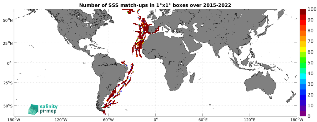
Figure 4: Number of SSS match-ups between TSG (CSIC-UTM) SSS and the SMAP SSS L2 v5 (RSS) SSS product for the SMOS coastal zone (<800km) 60N-60S Pi-MEP region over 1^\circ \times 1^\circ boxes and for the full satellite product period.
