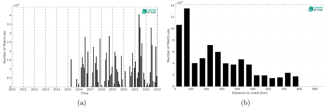
Figure 1: Number of match-ups between TSG (CSIC-UTM) and SMAP SSS L2 v5 (RSS) SSS as a function of time (a) and as function of the distance to coast (b) over the SMOS coastal zone (<800km) 60N-60S Pi-MEP region and for the full satellite product period.
