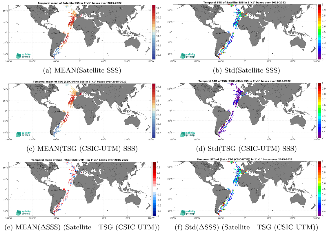
Figure 6: Temporal mean (left) and Std (right) of SSS from SMAP SSS L2 v5 (RSS) (top), TSG (CSIC-UTM) (middle), and of \Delta SSS (Satellite - TSG (CSIC-UTM)). Only match-up pairs are used to generate these maps.
