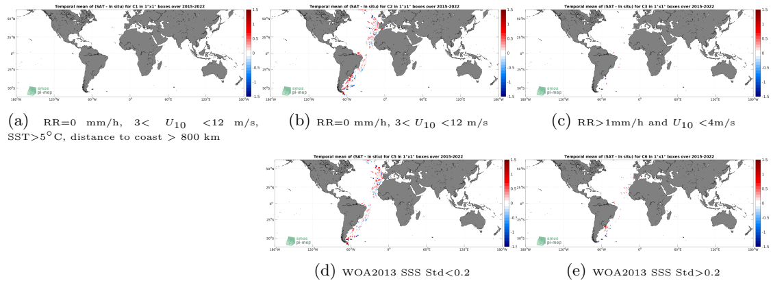
Figure 12: Temporal mean gridded over spatial boxes of size 1^\circ \times 1^\circ of \Delta\text{SSS} (SMAP SSS L2 v5 (RSS) - TSG (CSIC-UTM)) for 5 different subdatasets corresponding to: \text{RR}=0 mm/h, 3 < U_{10} < 12 m/s, \text{SST} > 5^\circ\text{C} , distance to coast > 800 km (a), \text{RR}=0 mm/h, 3 < U_{10} < 12 m/s (b), \text{RR} > 1\text{mm/h} and U_{10} < 4\text{m/s} (c), WOA2013 SSS Std < 0.2 (d), WOA2013 SSS Std > 0.2 (e).
