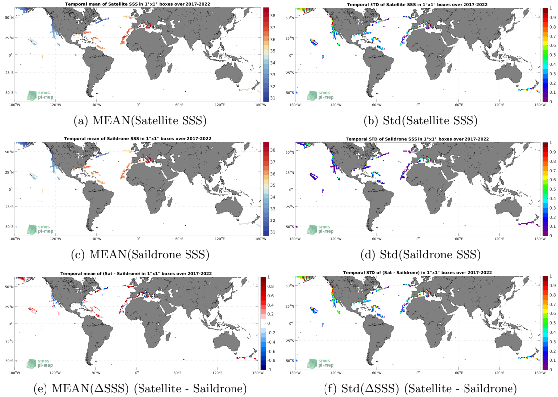
Figure 6: Temporal mean (left) and Std (right) of SSS from SMAP SSS L2 v5 (RSS) (top), Saildrone (middle), and of \Delta SSS (Satellite - Saildrone). Only match-up pairs are used to generate these maps.
