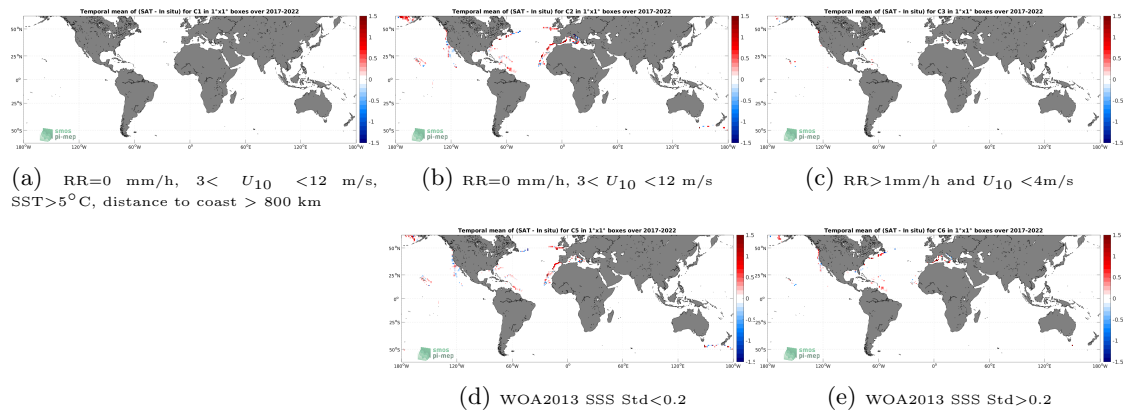
Figure 12: Temporal mean gridded over spatial boxes of size 1^\circ \times 1^\circ of \Delta SSS (SMAP SSS L2 v5 (RSS) - Saldrone) for 5 different subdatasets corresponding to: RR=0 mm/h, 3 < U_{10} < 12 m/s, SST > 5^\circ\text{C} , distance to coast > 800 km (a), RR=0 mm/h, 3 < U_{10} < 12 m/s (b), RR > 1 mm/h and U_{10} < 4 m/s (c), WOA2013 SSS Std < 0.2 (d), WOA2013 SSS Std > 0.2 (e).
