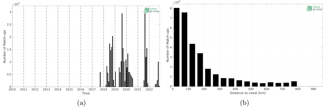
Figure 1: Number of match-ups between Saildrone and SMAP SSS L2 v5 (RSS) SSS as a function of time (a) and as function of the distance to coast (b) over the SMOS coastal zone ( <800\text{km} ) 60N-60S Pi-MEP region and for the full satellite product period.
