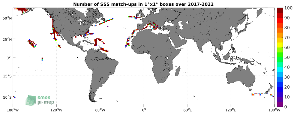
Figure 4: Number of SSS match-ups between Saildrone SSS and the SMAP SSS L2 v5 (RSS) SSS product for the SMOS coastal zone (<800km) 60N-60S Pi-MEP region over 1^\circ \times 1^\circ boxes and for the full satellite product period.
