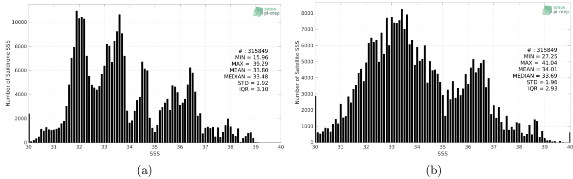
Figure 2: Histograms of SSS from Saildrone (a) and SMAP SSS L2 v5 (RSS) (b) considering all match-up pairs per bins of 0.1 over the SMOS coastal zone ( <800\text{km} ) 60N-60S Pi-MEP region and for the full satellite product period.
