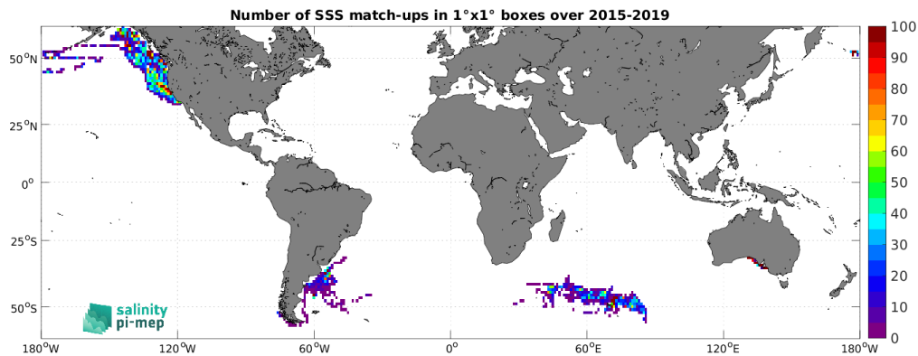
Figure 4: Number of SSS match-ups between Marine mammals SSS and the SMAP SSS L2 v5 (RSS) SSS product for the SMOS coastal zone (<800km) 60N-60S Pi-MEP region over 1^\circ \times 1^\circ boxes and for the full satellite product period.
