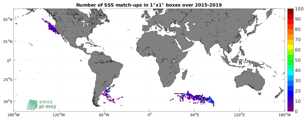
Figure 4: Number of SSS match-ups between Marine mammals SSS and the SMAP SSS L2 v5 (RSS) SSS product for the SMOS coastal zone (<800km) 60N-60S Pi-MEP region over 1°x1° boxes and for the full satellite product period.
