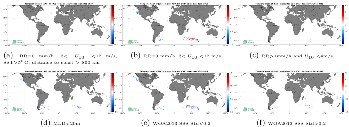
Figure 12: Temporal mean gridded over spatial boxes of size 1^\circ \times 1^\circ of \Delta SSS (SMAP SSS L2 v5 (RSS) - Marine mammals) for 6 different subdatasets corresponding to:RR=0 mm/h, 3 < U_{10} < 12 m/s, SST > 5^\circ\text{C} , distance to coast > 800 km (a), RR=0 mm/h, 3 < U_{10} < 12 m/s (b), RR > 1 mm/h and U_{10} < 4 m/s (c),MLD < 20 m (d),WOA2013 SSS Std < 0.2 (e),WOA2013 SSS Std > 0.2 (f).
