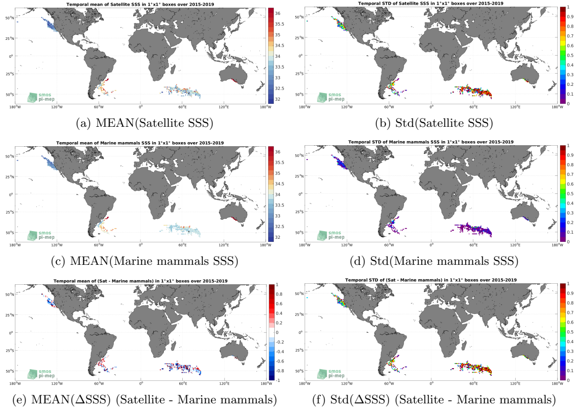
Figure 6: Temporal mean (left) and Std (right) of SSS from SMAP SSS L2 v5 (RSS) (top), Marine mammals (middle), and of \Delta SSS (Satellite - Marine mammals). Only match-up pairs are used to generate these maps.
