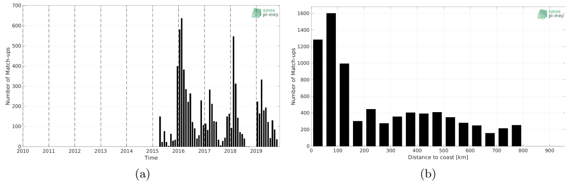
Figure 1: Number of match-ups between Marine mammals and SMAP SSS L2 v5 (RSS) SSS as a function of time (a) and as function of the distance to coast (b) over the SMOS coastal zone (<800km) 60N-60S Pi-MEP region and for the full satellite product period.
