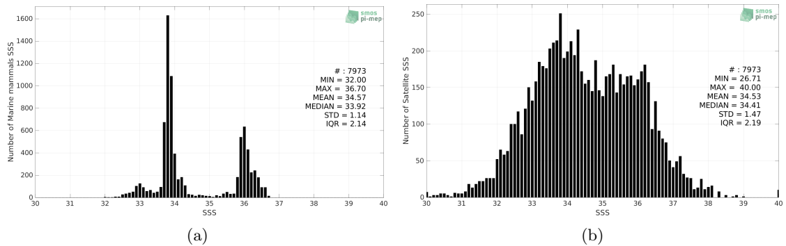
Figure 2: Histograms of SSS from Marine mammals (a) and SMAP SSS L2 v5 (RSS) (b) considering all match-up pairs per bins of 0.1 over the SMOS coastal zone (<800km) 60N-60S Pi-MEP region and for the full satellite product period.
