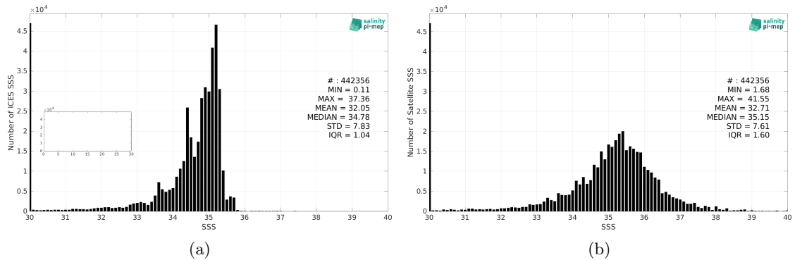
Figure 2: Histograms of SSS from ICES (a) and SMAP SSS L2 v5 (RSS) (b) considering all match-up pairs per bins of 0.1 over the SMOS coastal zone (<800km) 60N-60S Pi-MEP region and for the full satellite product period.
