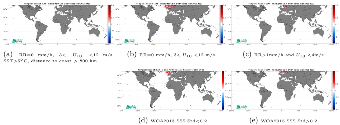
Figure 12: Temporal mean gridded over spatial boxes of size 1^\circ \times 1^\circ of \Delta SSS (SMAP SSS L2 v5 (RSS) - ICES) for 5 different subdatasets corresponding to:RR=0 mm/h, 3 < U_{10} < 12 m/s, SST >5^\circ\text{C} , distance to coast > 800 km (a), RR=0 mm/h, 3 < U_{10} < 12 m/s (b), RR >1 mm/h and U_{10} < 4 m/s (c), WOA2013 SSS Std <0.2 (d), WOA2013 SSS Std >0.2 (e).
