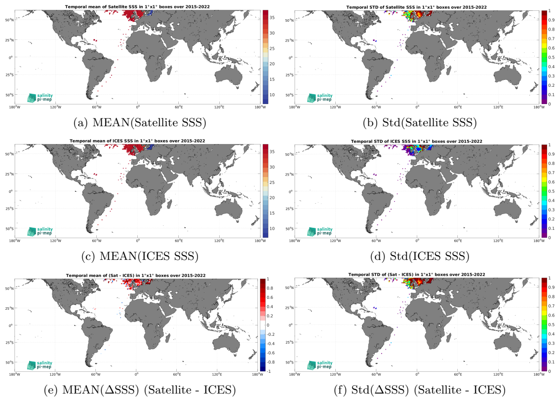
Figure 6: Temporal mean (left) and Std (right) of SSS from SMAP SSS L2 v5 (RSS) (top), ICES (middle), and of \Delta SSS (Satellite - ICES). Only match-up pairs are used to generate these maps.
