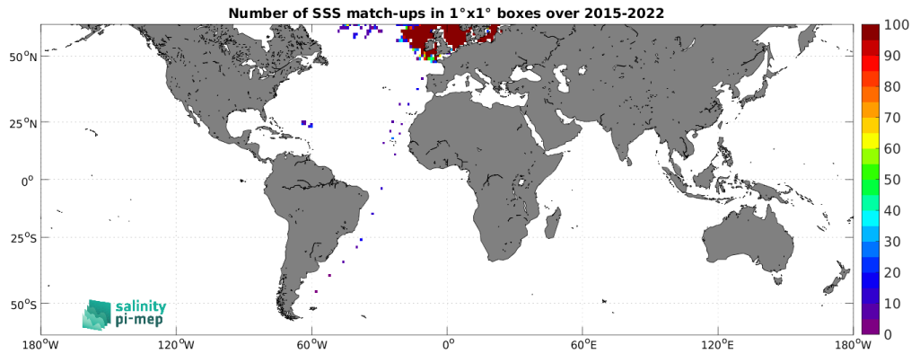
Figure 4: Number of SSS match-ups between ICES SSS and the SMAP SSS L2 v5 (RSS) SSS product for the SMOS coastal zone (<800km) 60N-60S Pi-MEP region over 1^\circ \times 1^\circ boxes and for the full satellite product period.
