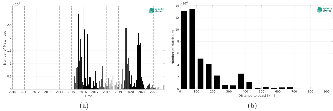
Figure 1: Number of match-ups between ICES and SMAP SSS L2 v5 (RSS) SSS as a function of time (a) and as function of the distance to coast (b) over the SMOS coastal zone (<800km) 60N-60S Pi-MEP region and for the full satellite product period.
