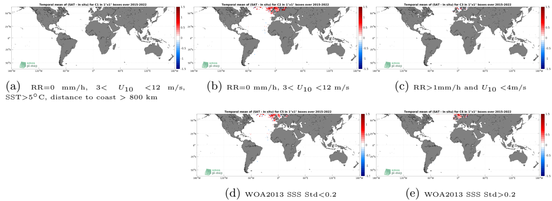
Figure 12: Temporal mean gridded over spatial boxes of size 1^\circ \times 1^\circ of \Delta\text{SSS} (SMAP SSS L2 v5 (RSS) - ICES) for 5 different subdatasets corresponding to:RR=0 mm/h, 3 < U_{10} < 12 m/s, SST >5^\circ\text{C} , distance to coast > 800 km (a), RR=0 mm/h, 3 < U_{10} < 12 m/s (b), RR >1 mm/h and U_{10} < 4 m/s (c), WOA2013 SSS Std <0.2 (d), WOA2013 SSS Std >0.2 (e).
