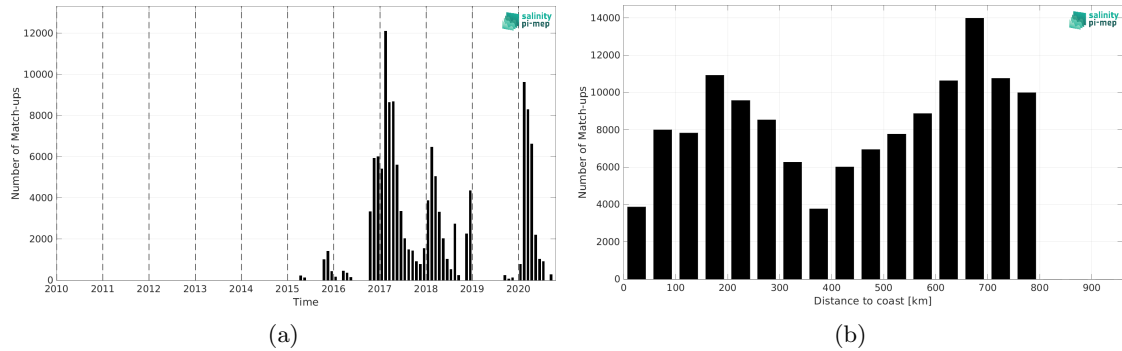
Figure 1: Number of match-ups between Surface drifters and SMAP SSS L2 v5 (RSS) SSS as a function of time (a) and as function of the distance to coast (b) over the SMOS coastal zone (<800km) 60N-60S Pi-MEP region and for the full satellite product period.
