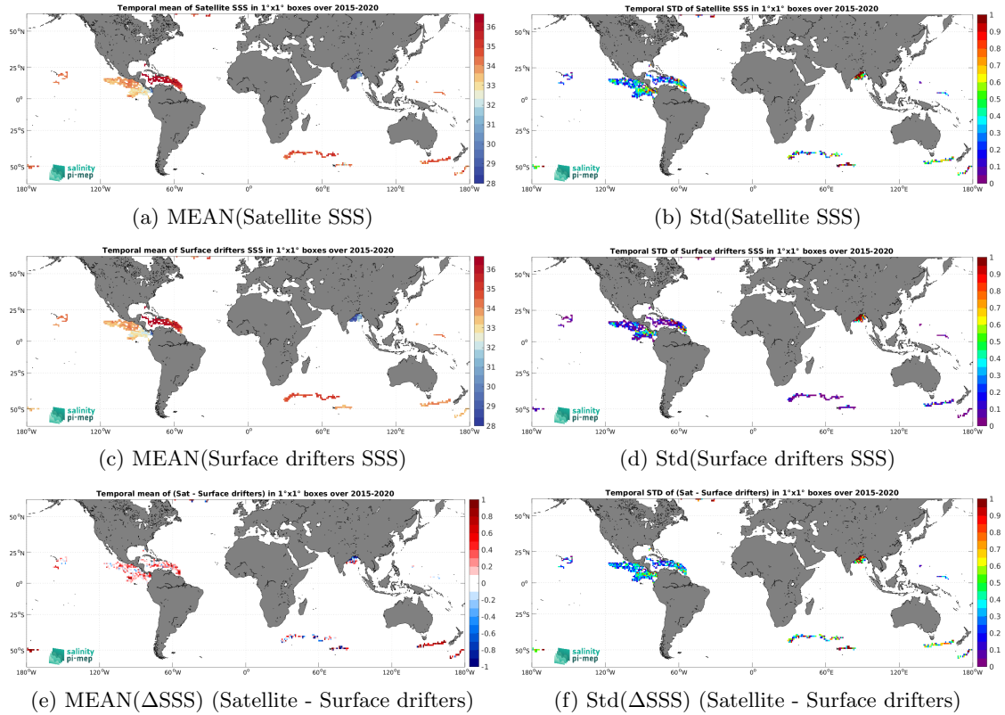
Figure 5: Temporal mean (left) and Std (right) of SSS from SMAP SSS L2 v5 (RSS) (top), Surface drifters (middle), and of \Delta SSS (Satellite - Surface drifters). Only match-up pairs are used to generate these maps.
