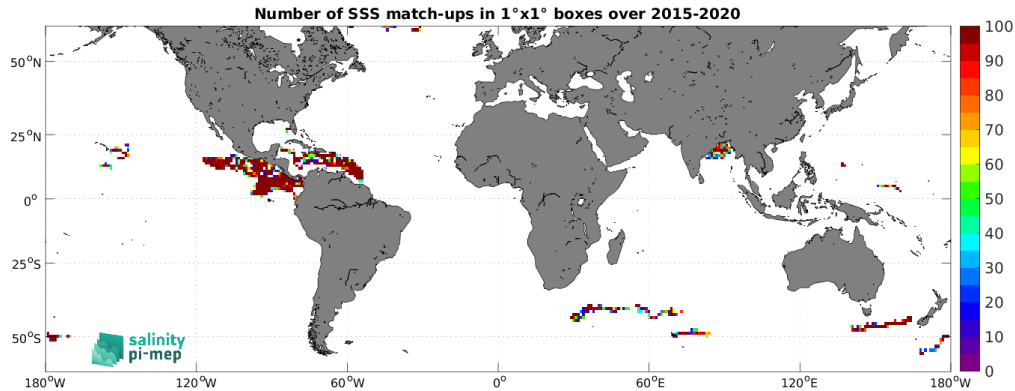
Figure 3: Number of SSS match-ups between Surface drifters SSS and the SMAP SSS L2 v5 (RSS) SSS product for the SMOS coastal zone (<800km) 60N-60S Pi-MEP region over 1^\circ \times 1^\circ boxes and for the full satellite product period.
