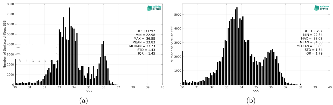
Figure 2: Histograms of SSS from Surface drifters (a) and SMAP SSS L2 v5 (RSS) (b) considering all match-up pairs per bins of 0.1 over the SMOS coastal zone (<800km) 60N-60S Pi-MEP region and for the full satellite product period.
