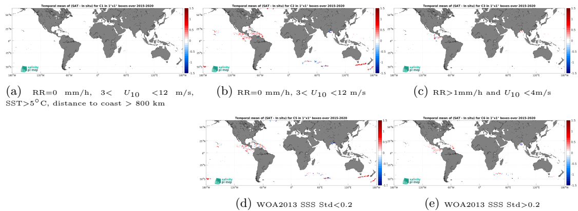
Figure 11: Temporal mean gridded over spatial boxes of size 1^\circ \times 1^\circ of \Delta\text{SSS} (SMAP SSS L2 v5 (RSS) - Surface drifters) for 5 different subdatasets corresponding to:RR=0 mm/h, 3 < U_{10} < 12 m/s, SST >5^\circ\text{C} , distance to coast > 800 km (a), RR=0 mm/h, 3 < U_{10} < 12 m/s (b), RR >1 mm/h and U_{10} < 4 m/s (c), WOA2013 SSS Std <0.2 (d), WOA2013 SSS Std >0.2 (e).
