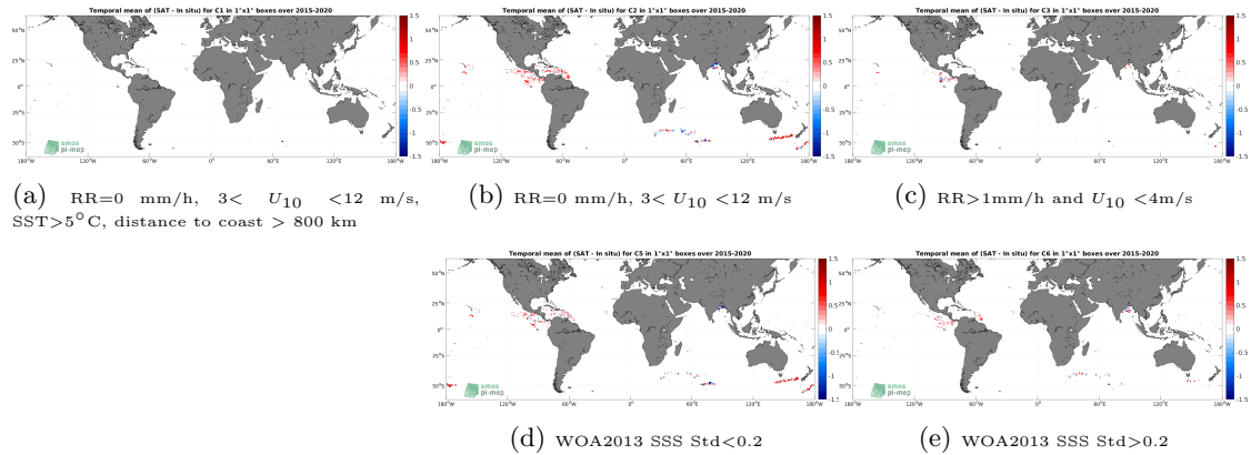
Figure 11: Temporal mean gridded over spatial boxes of size 1^\circ \times 1^\circ of \Delta SSS (SMAP SSS L2 v5 (RSS) - Surface drifters) for 5 different subdatasets corresponding to:RR=0 mm/h, 3 < U_{10} < 12 m/s, SST >5^\circ C, distance to coast > 800 km (a), RR=0 mm/h, 3 < U_{10} < 12 m/s (b), RR >1 mm/h and U_{10} < 4 m/s (c), WOA2013 SSS Std <0.2 (d), WOA2013 SSS Std >0.2 (e).
