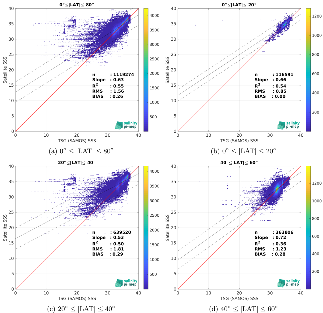
Figure 10: Contour maps of the concentration of SMAP SSS L2 v5.3 (RSS) SSS (y-axis) versus TSG (SAMOS) SSS (x-axis) at match-up pairs for different latitude bands. For each plot, the red line shows x=y . The black thin and dashed lines indicate a linear fit through the data cloud and the \pm 95\% confidence levels, respectively. The number match-up pairs n , the slope and R^2 coefficient of the linear fit, the root mean square (RMS) and the mean bias between satellite and in situ data are indicated for each latitude band in each plots.
