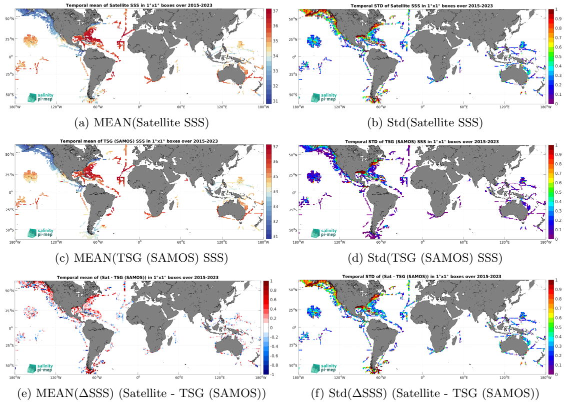
Figure 7: Temporal mean (left) and Std (right) of SSS from SMAP SSS L2 v5.3 (RSS) (top), TSG (SAMOS) (middle), and of \Delta SSS (Satellite - TSG (SAMOS)). Only match-up pairs are used to generate these maps.
