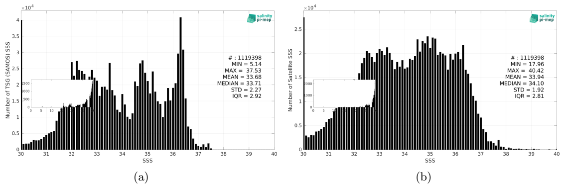
Figure 3: Histograms of SSS from TSG (SAMOS) (a) and SMAP SSS L2 v5.3 (RSS) (b) considering all match-up pairs per bins of 0.1 over the SMOS coastal zone (<800km) 60N-60S Pi-MEP region and for the full satellite product period.
