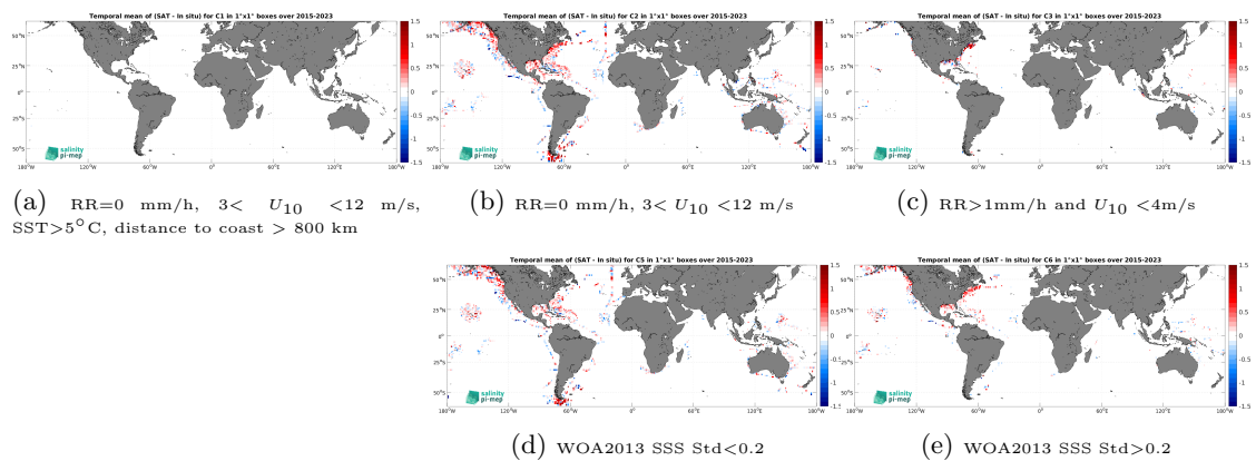
Figure 14: Temporal mean gridded over spatial boxes of size 1^\circ \times 1^\circ of \Delta\text{SSS} (SMAP SSS L2 v5.3 (RSS) - TSG (SAMOS)) for 5 different subdatasets corresponding to:RR=0 mm/h, 3 < U_{10} < 12 m/s, SST >5^\circ\text{C} , distance to coast > 800 km (a), RR=0 mm/h, 3 < U_{10} < 12 m/s (b), RR >1 mm/h and U_{10} < 4 m/s (c), WOA2013 SSS Std <0.2 (d), WOA2013 SSS Std >0.2 (e).
