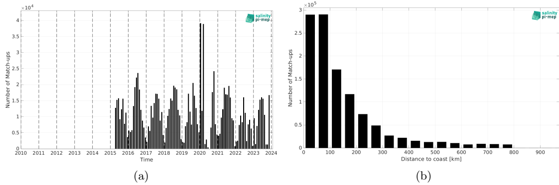
Figure 2: Number of match-ups between TSG (SAMOS) and SMAP SSS L2 v5.3 (RSS) SSS as a function of time (a) and as function of the distance to coast (b) over the SMOS coastal zone (<800km) 60N-60S Pi-MEP region and for the full satellite product period.
