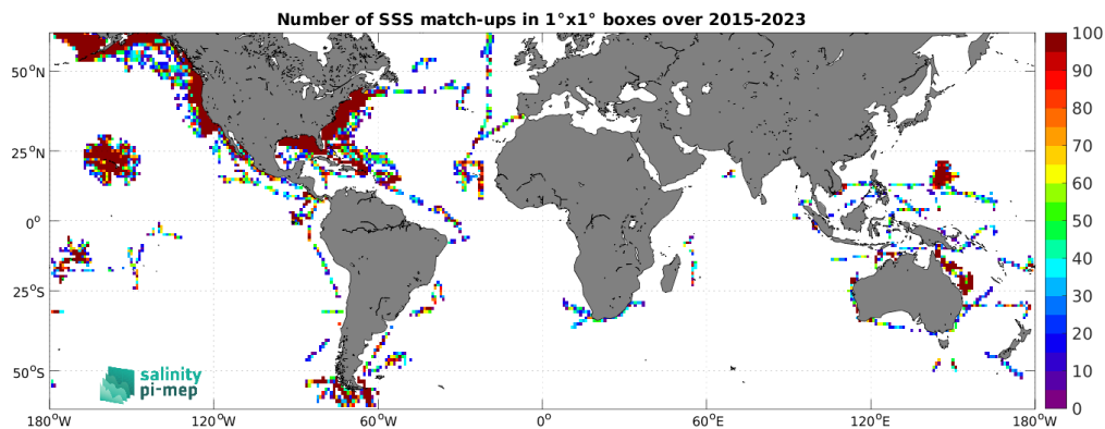
Figure 5: Number of SSS match-ups between TSG (SAMOS) SSS and the SMAP SSS L2 v5.3 (RSS) SSS product for the SMOS coastal zone ( <800\text{km} ) 60N-60S Pi-MEP region over 1^\circ \times 1^\circ boxes and for the full satellite product period.
