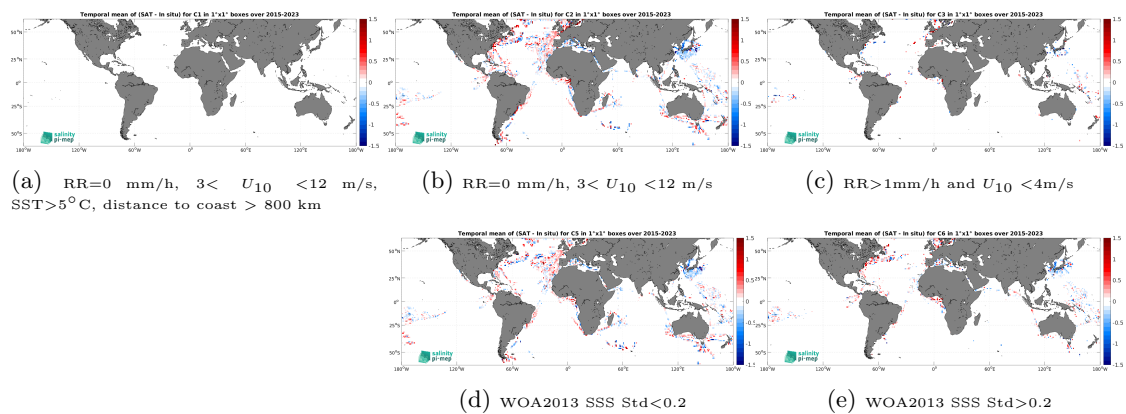
Figure 14: Temporal mean gridded over spatial boxes of size 1^\circ \times 1^\circ of \Delta\text{SSS} (SMAP SSS L2 v5.3 (RSS) - TSG (LEGOS-DM)) for 5 different subdatasets corresponding to:RR=0 mm/h, 3 < U_{10} < 12 m/s, SST >5^\circ\text{C} , distance to coast > 800 km (a), RR=0 mm/h, 3 < U_{10} < 12 m/s (b), RR >1 mm/h and U_{10} < 4 m/s (c), WOA2013 SSS Std <0.2 (d), WOA2013 SSS Std >0.2 (e).
