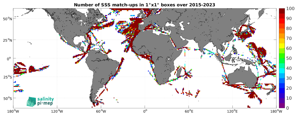
Figure 5: Number of SSS match-ups between TSG (LEGOS-DM) SSS and the SMAP SSS L2 v5.3 (RSS) SSS product for the SMOS coastal zone ( <800\text{km} ) 60\text{N} - 60\text{S} Pi-MEP region over 1^\circ \times 1^\circ boxes and for the full satellite product period.
