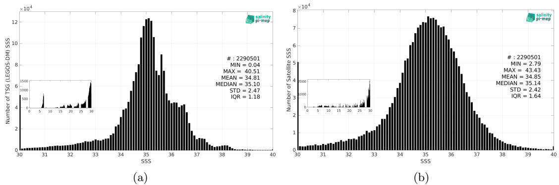
Figure 3: Histograms of SSS from TSG (LEGOS-DM) (a) and SMAP SSS L2 v5.3 (RSS) (b) considering all match-up pairs per bins of 0.1 over the SMOS coastal zone (<800km) 60N-60S Pi-MEP region and for the full satellite product period.
