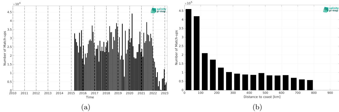
Figure 2: Number of match-ups between TSG (LEGOS-DM) and SMAP SSS L2 v5.3 (RSS) SSS as a function of time (a) and as function of the distance to coast (b) over the SMOS coastal zone (<800km) 60N-60S Pi-MEP region and for the full satellite product period.
