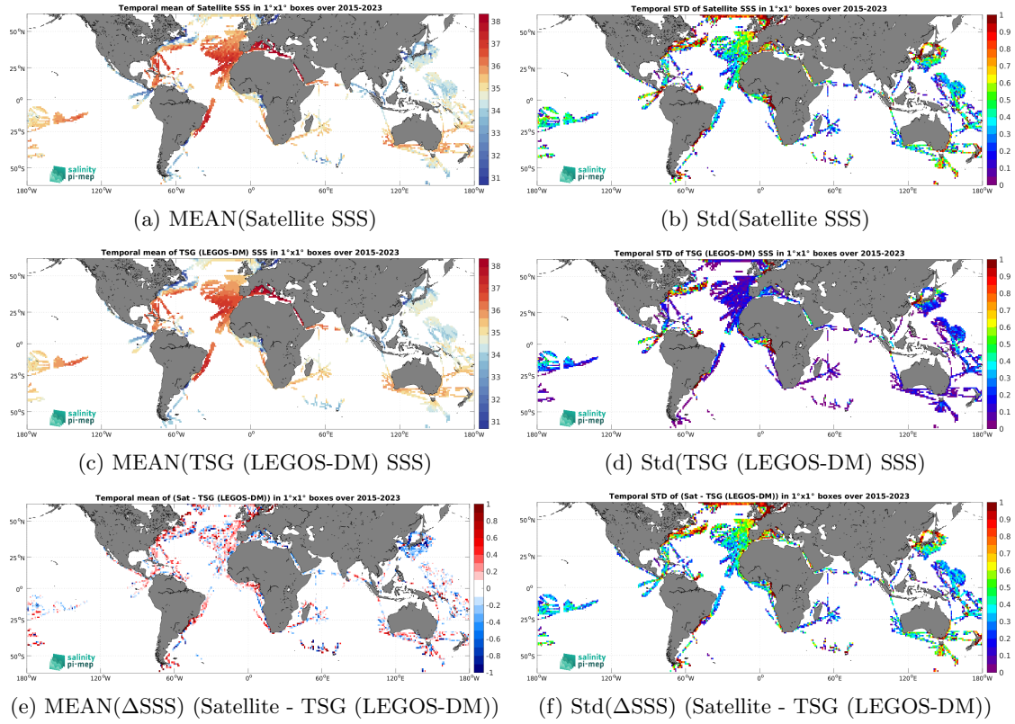
Figure 7: Temporal mean (left) and Std (right) of SSS from SMAP SSS L2 v5.3 (RSS) (top), TSG (LEGOS-DM) (middle), and of \Delta SSS (Satellite - TSG (LEGOS-DM)). Only match-up pairs are used to generate these maps.
